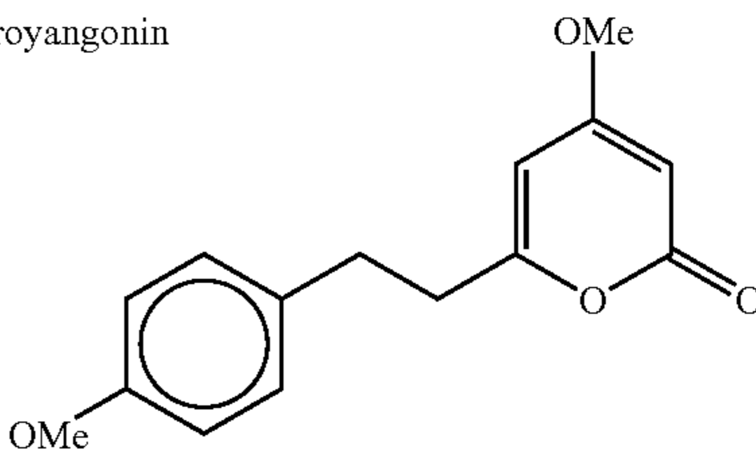
11. 10-Methoxy-yangonin
