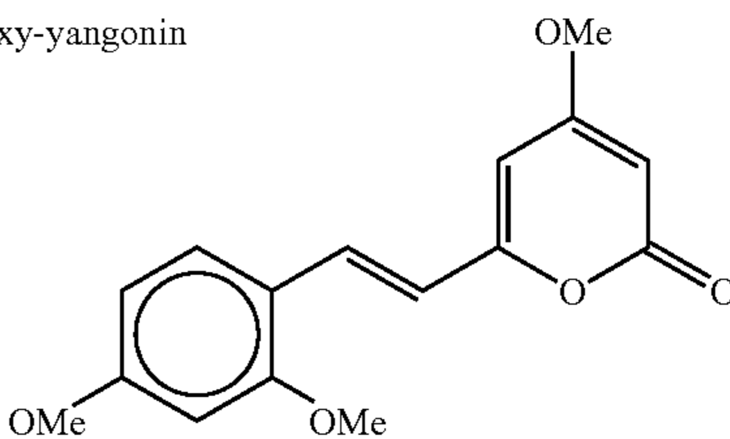
12. Methoxy-yangonin
