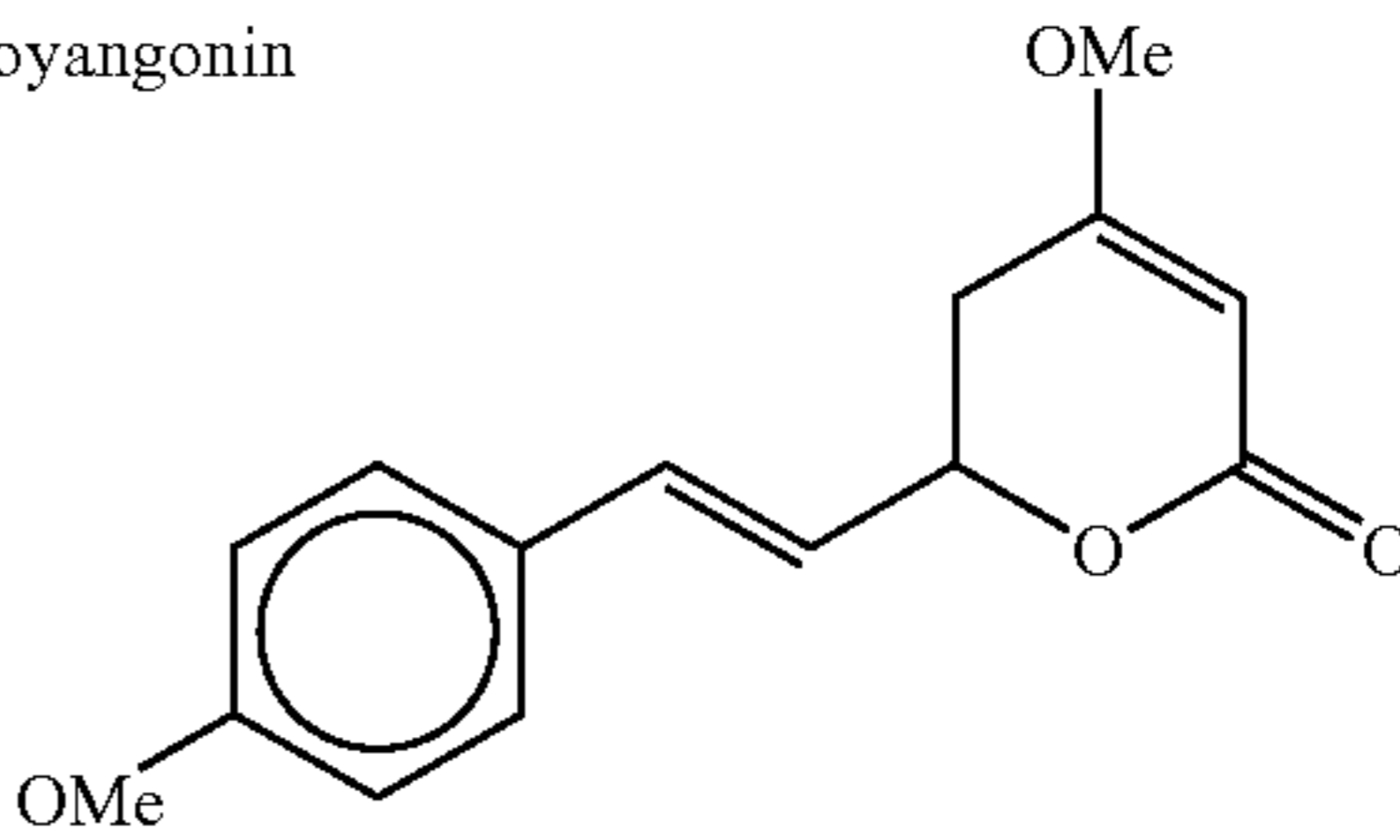
10. 7,8-Dihydroyangonin
