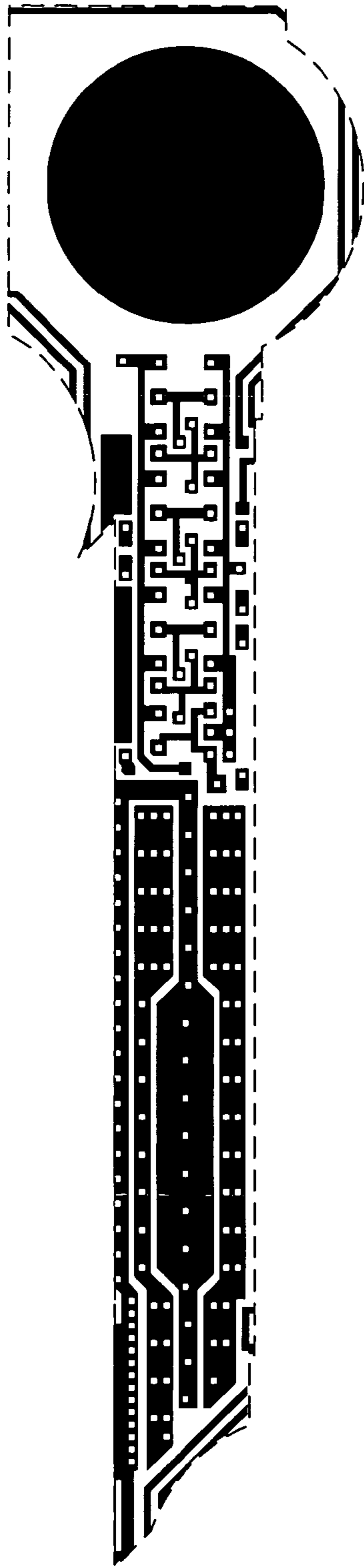
Metal 1 mask
