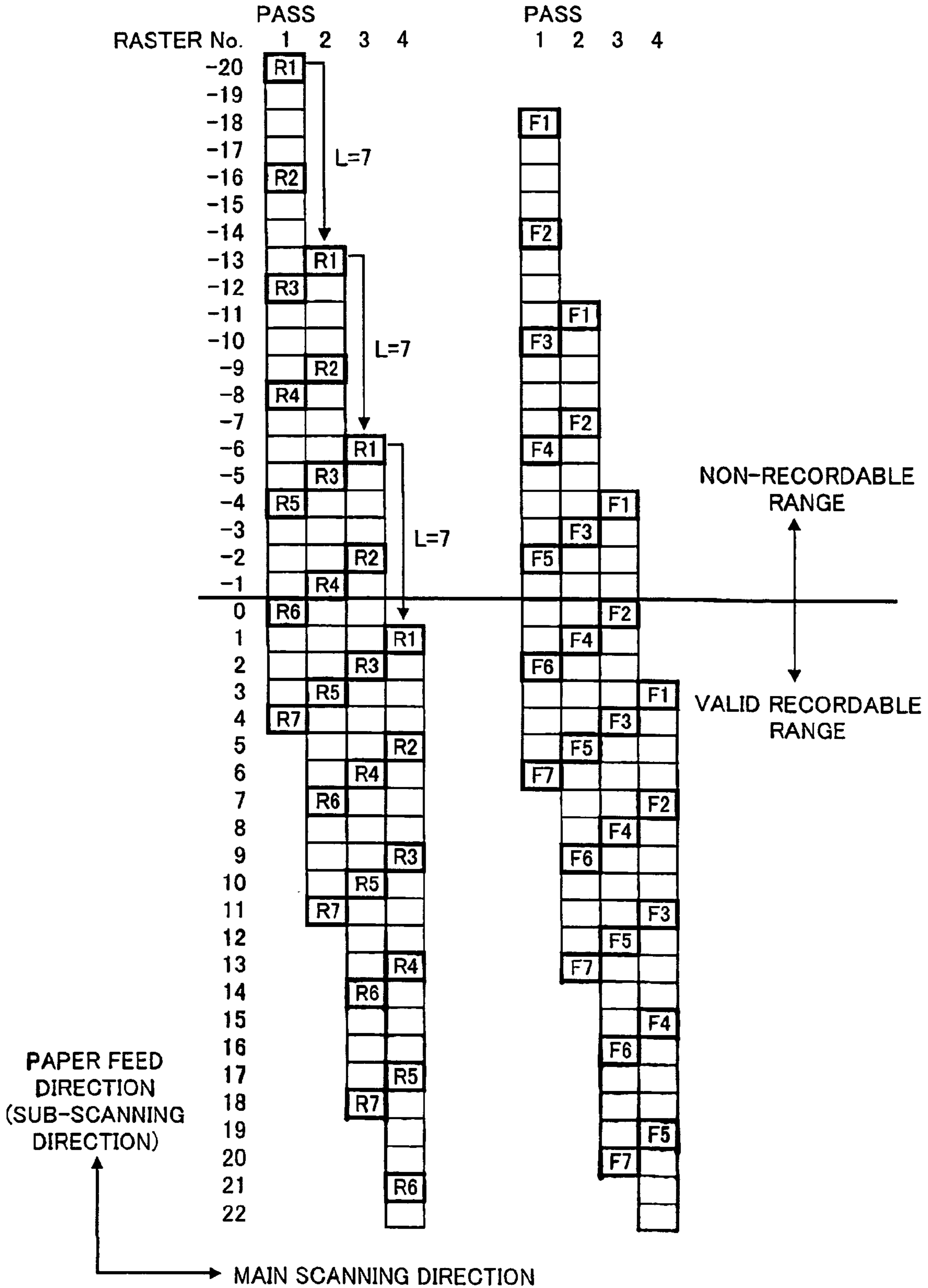
Fig. 17A TRAILING NOZZLE ARRAY RN
