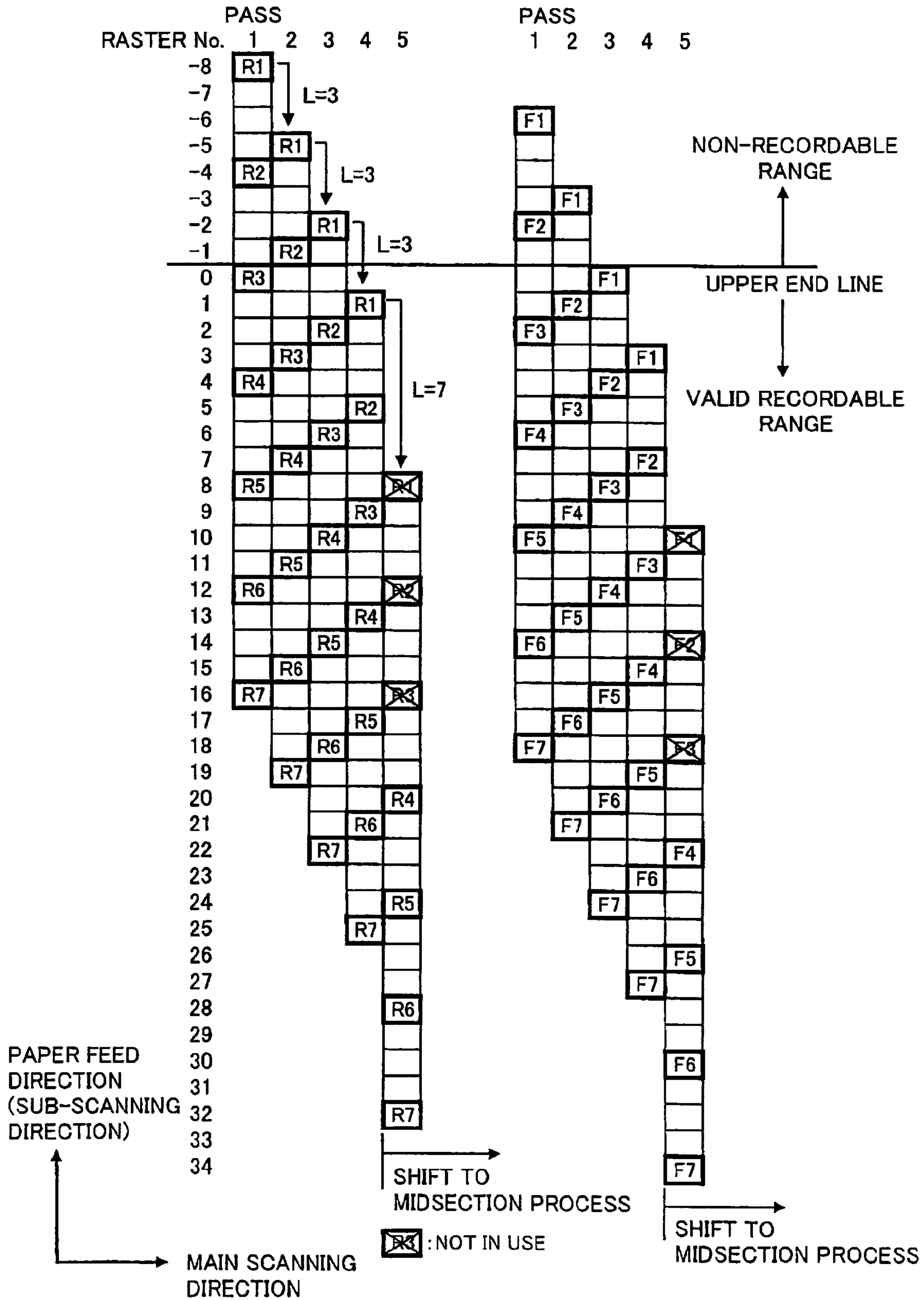
Fig. 19A TRAILING NOZZLE ARRAY RN
