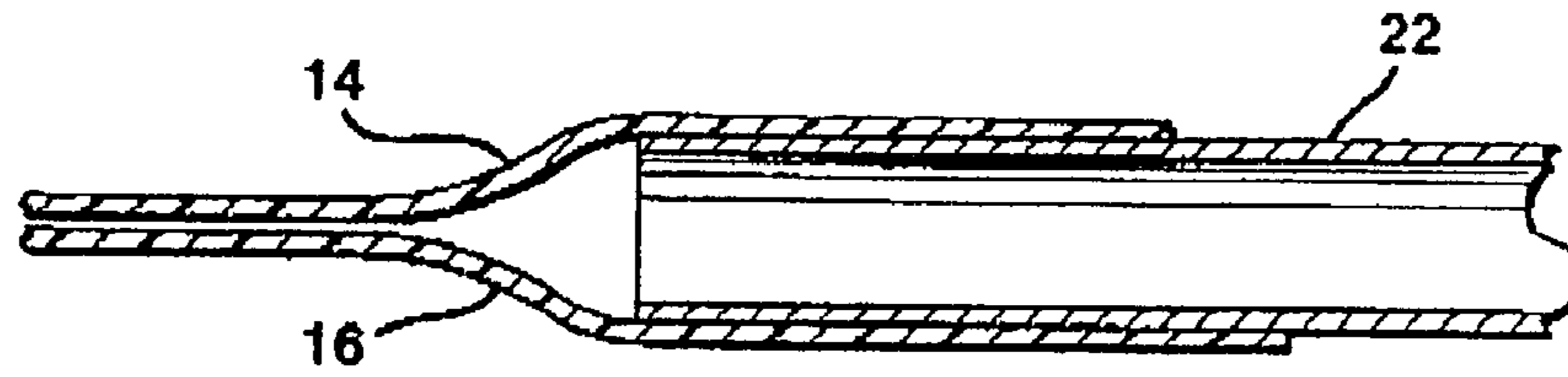
FIG. 3 PRIOR ART
