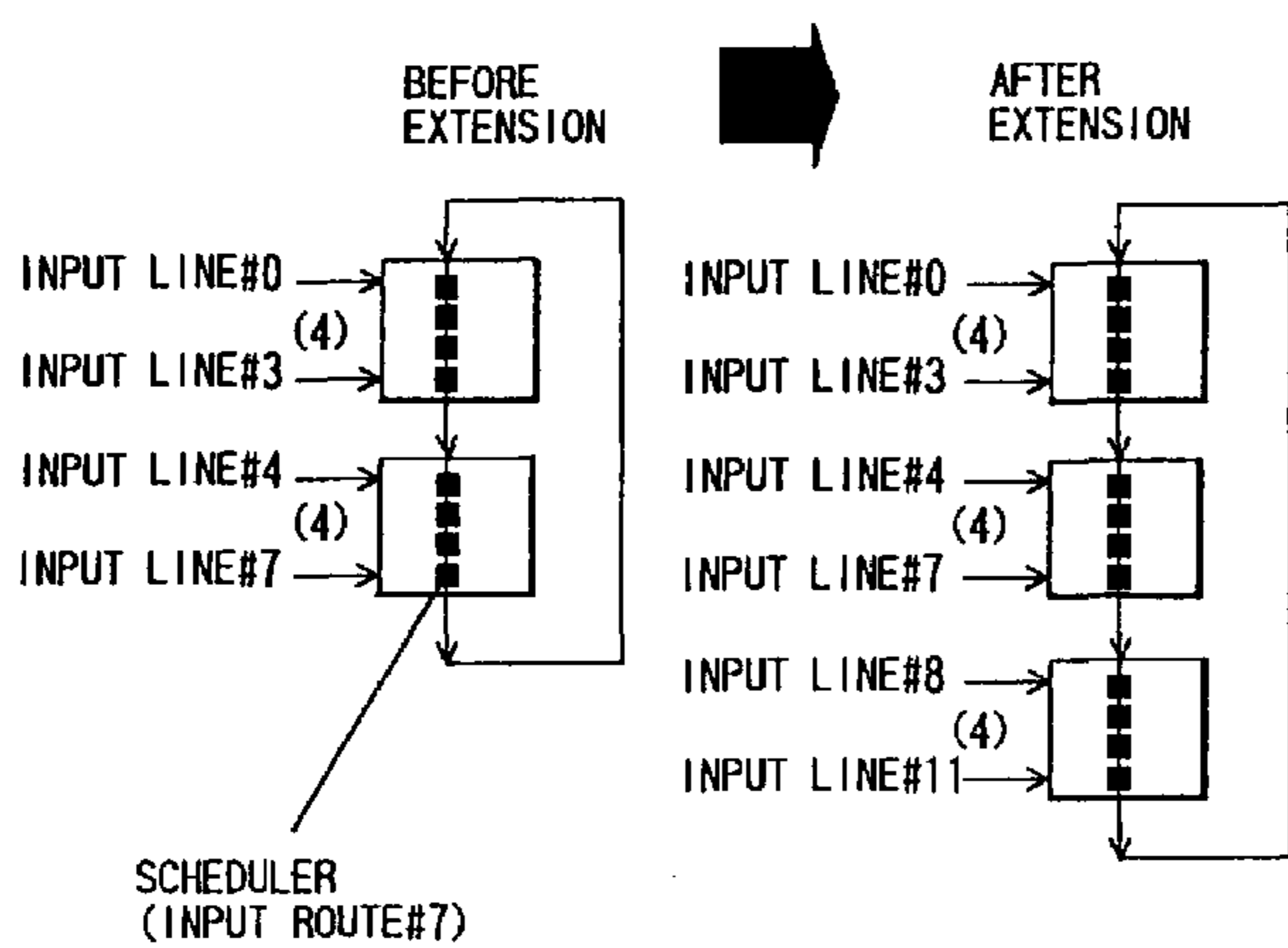
FIG. 58(a) RING CONNECTION
