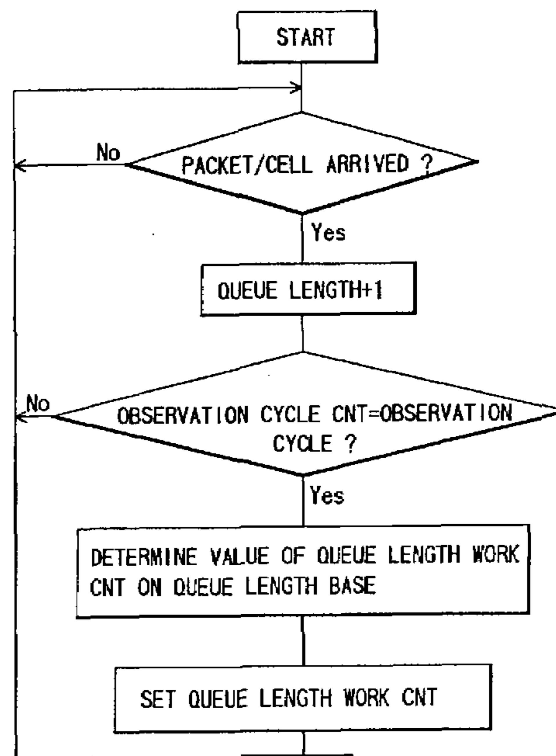
FIG. 54(b)(c) LOAD OBSERVATION FLOW BASED ON QUEUE LENGTH BASE (PART 2)
