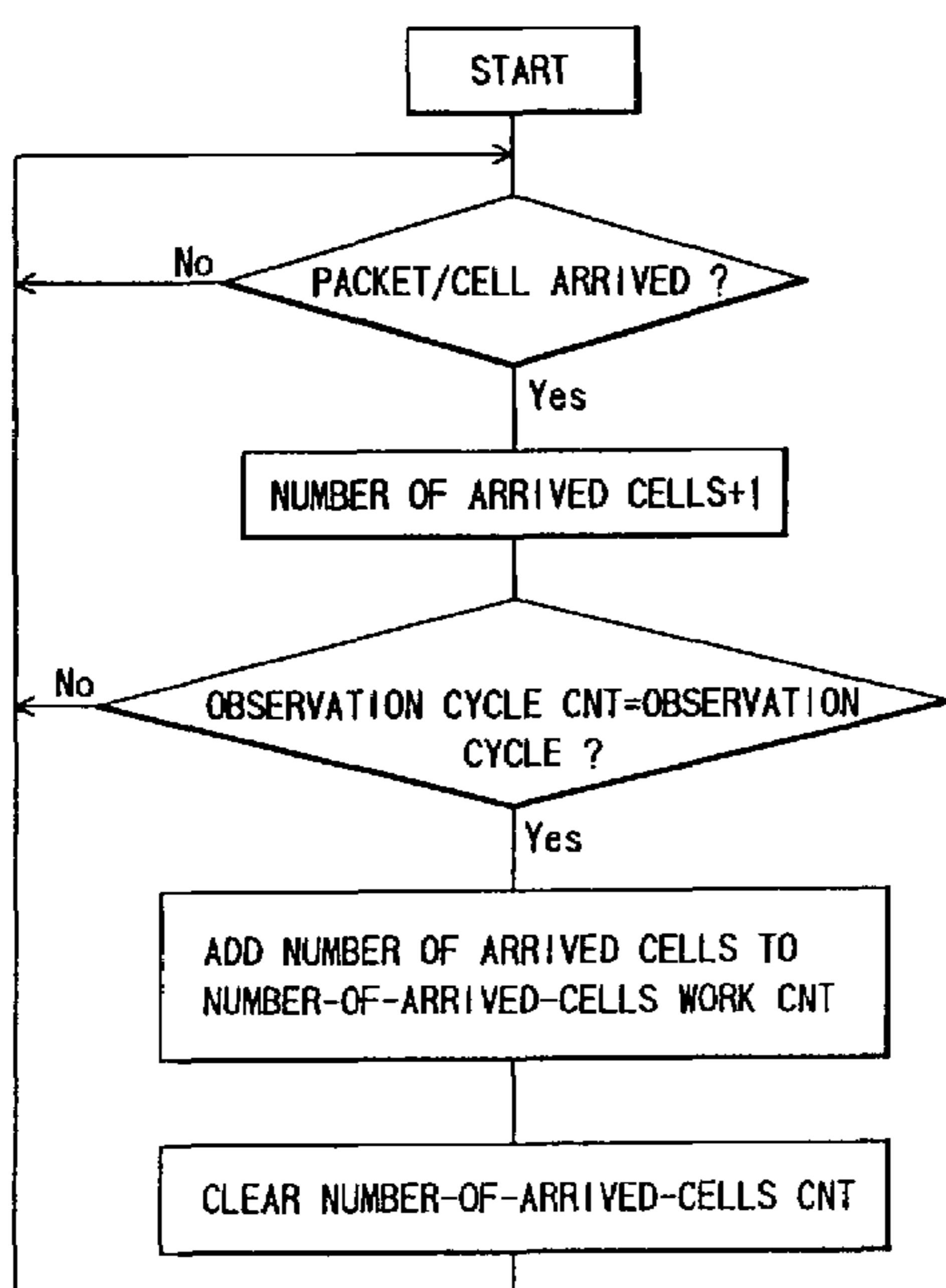
FIG. 50(a) LOAD OBSERVATION FLOW
