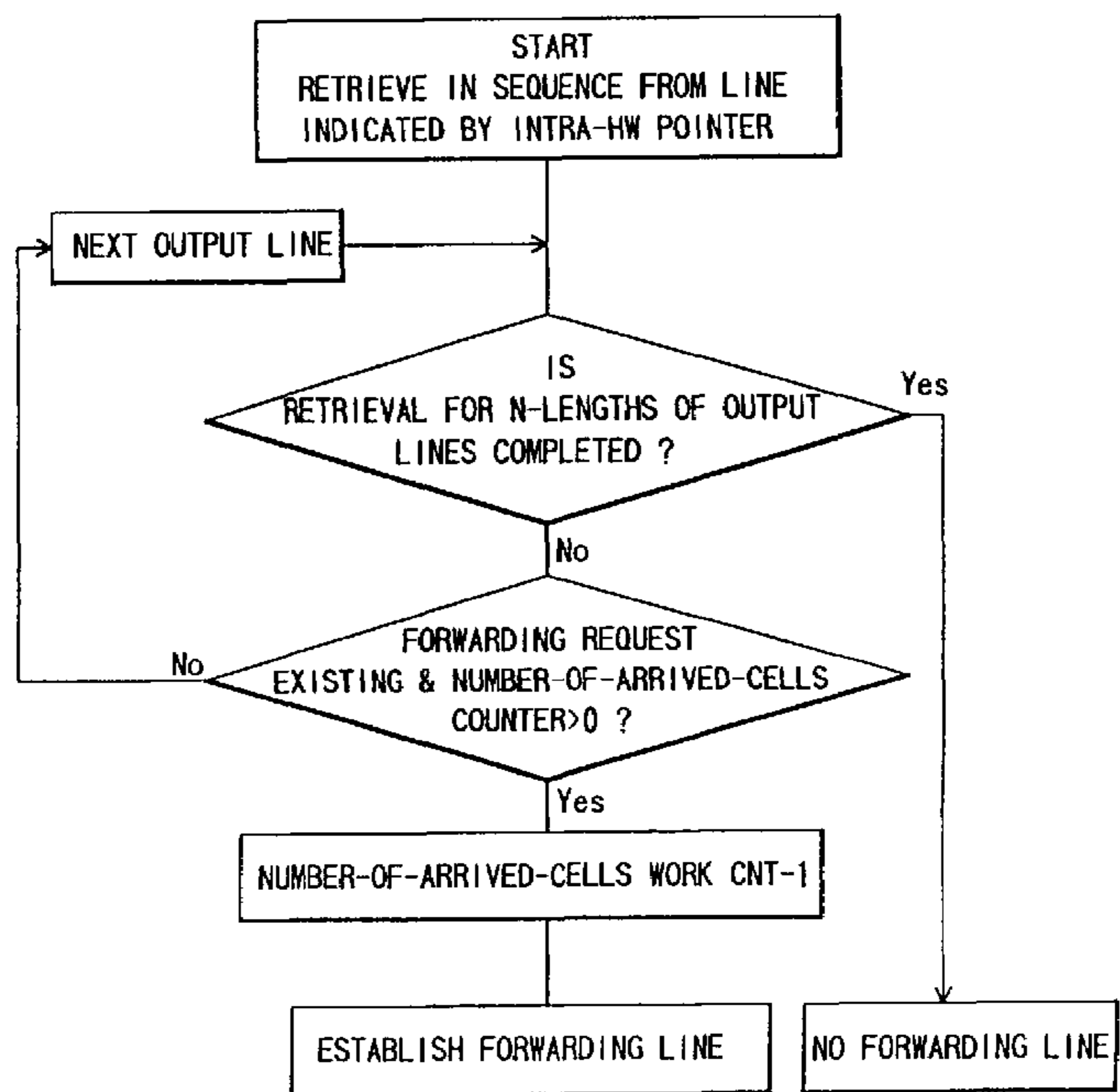
FIG. 50(b) SCHEDULING FLOW
