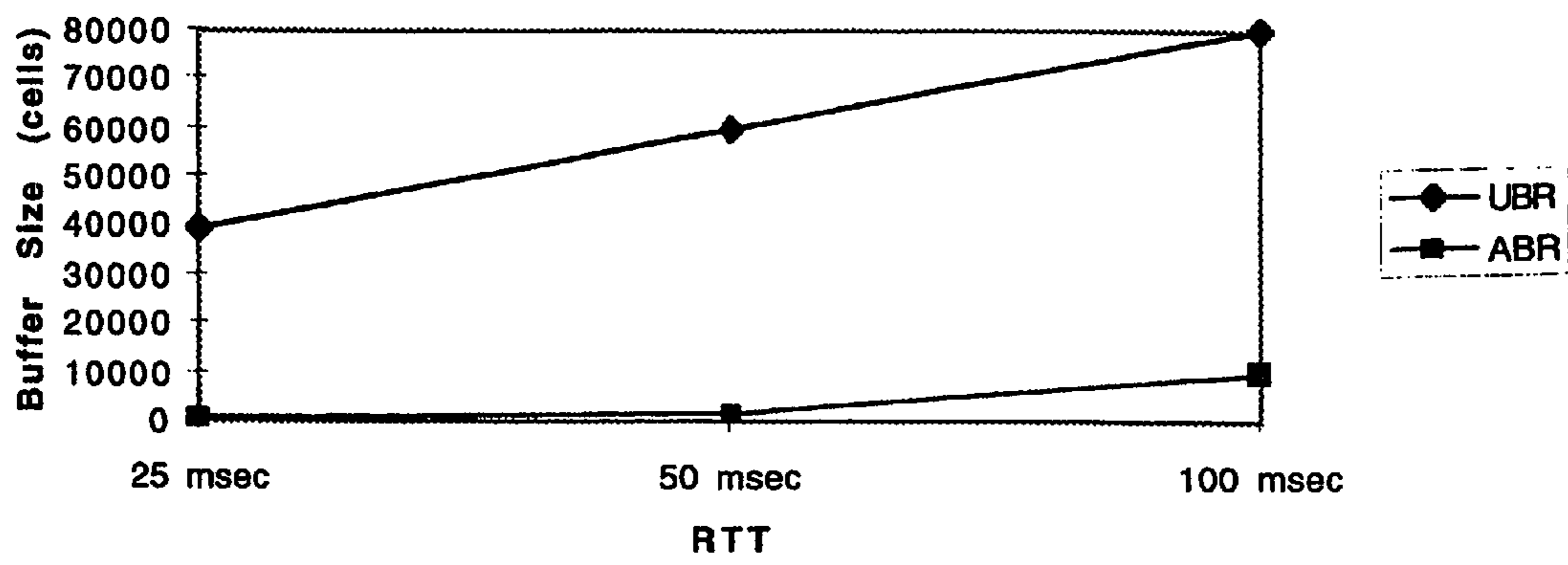
Figure 8 • Switch Buffer Requirements to Achieve Equivalent Goodput Performance
