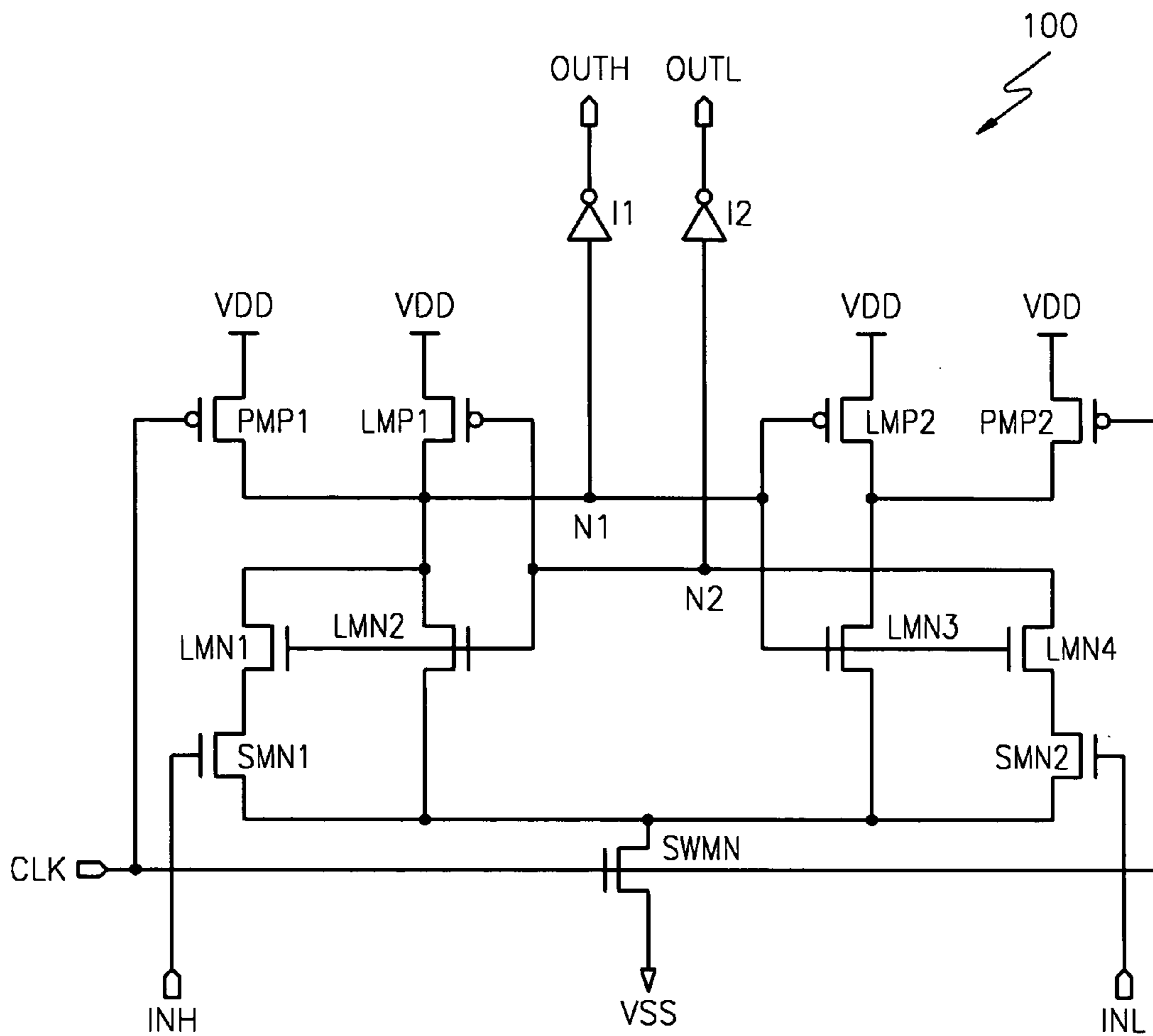
FIG. 1 (CONVENTIONAL ART)
