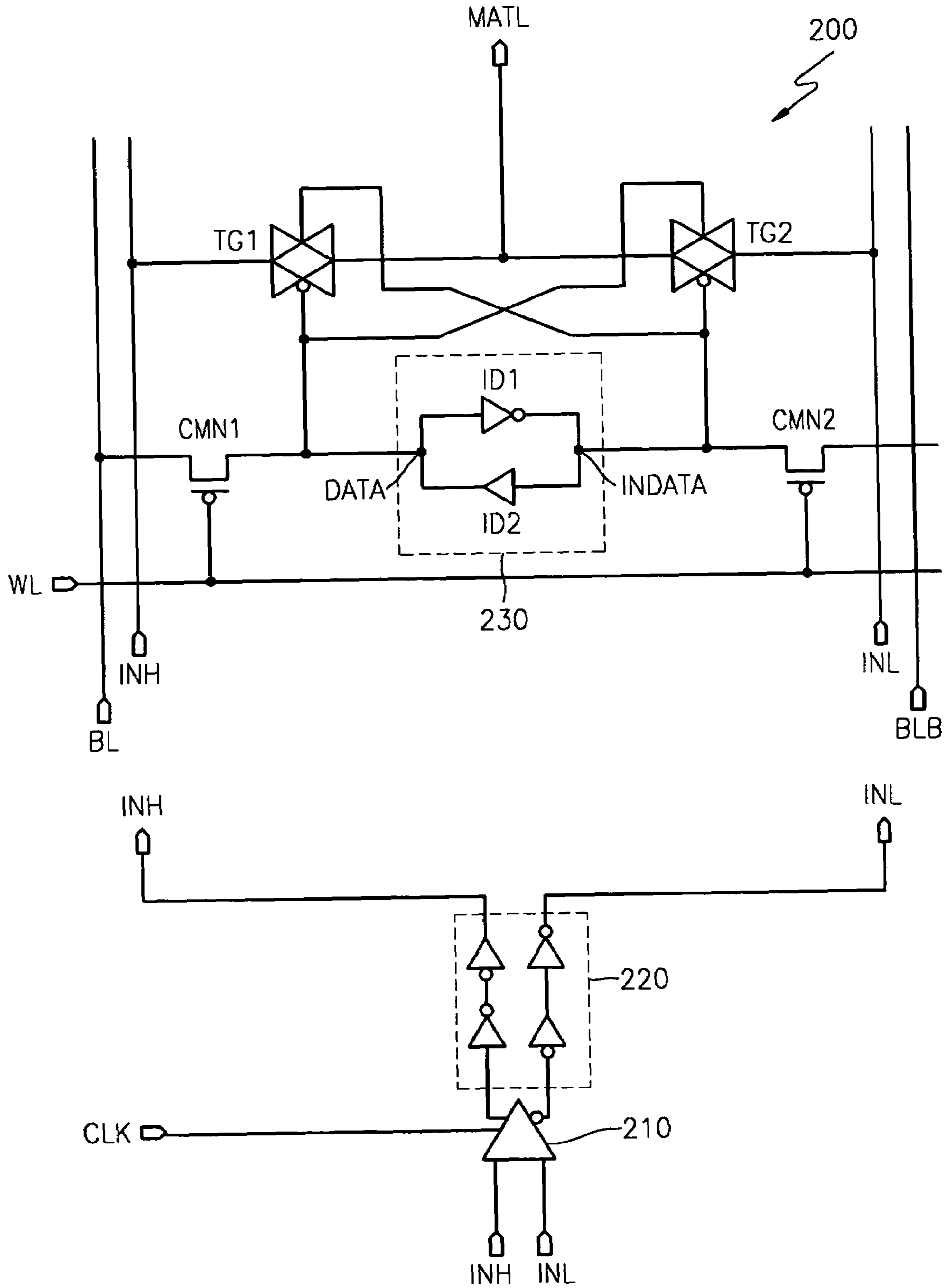
FIG. 2 (CONVENTIONAL ART)
