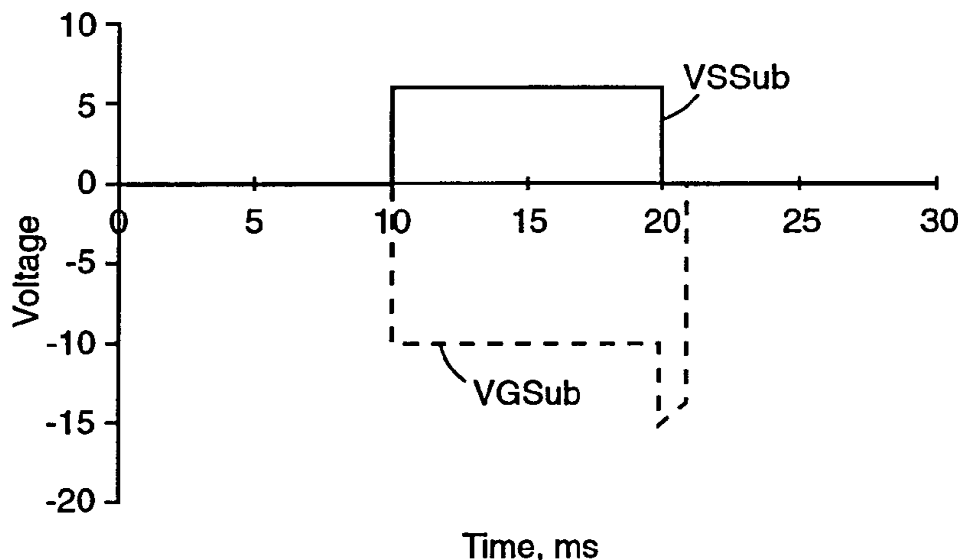
Source erase with delayed gate discharge
