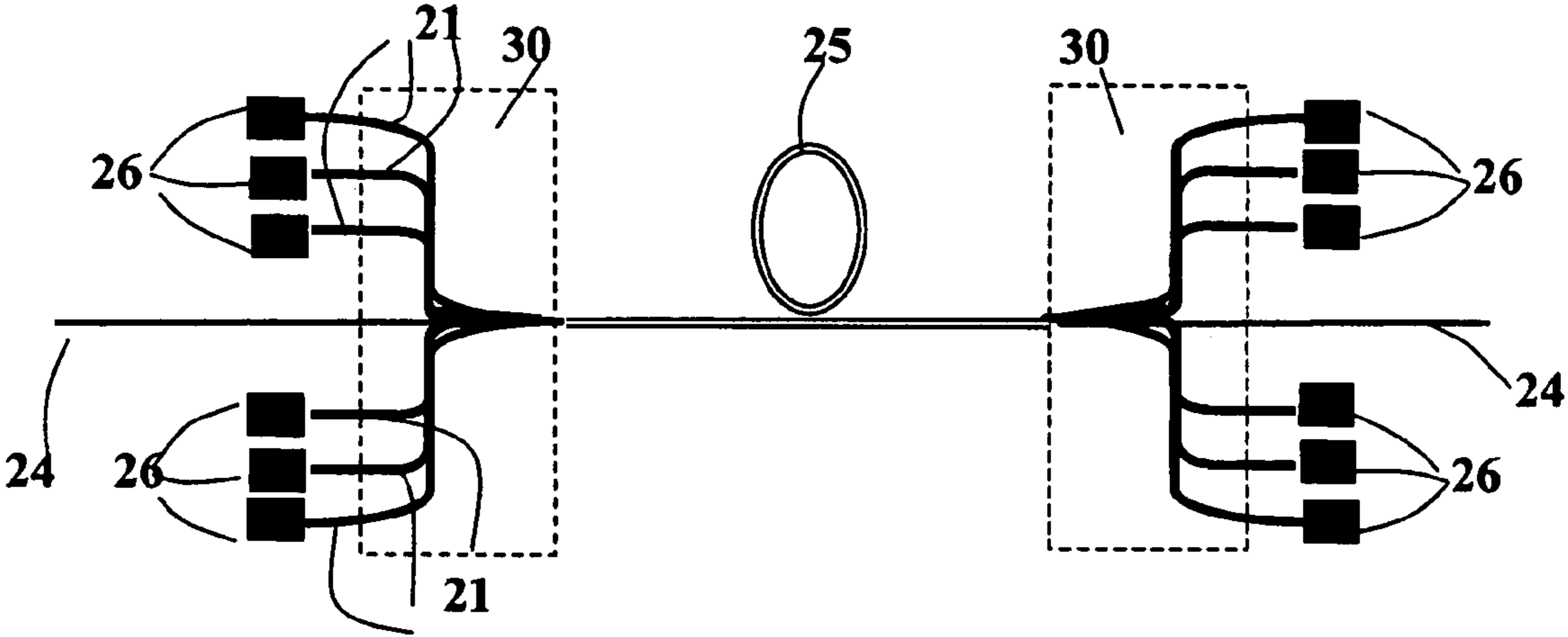
Fig.4 (Prior art)
