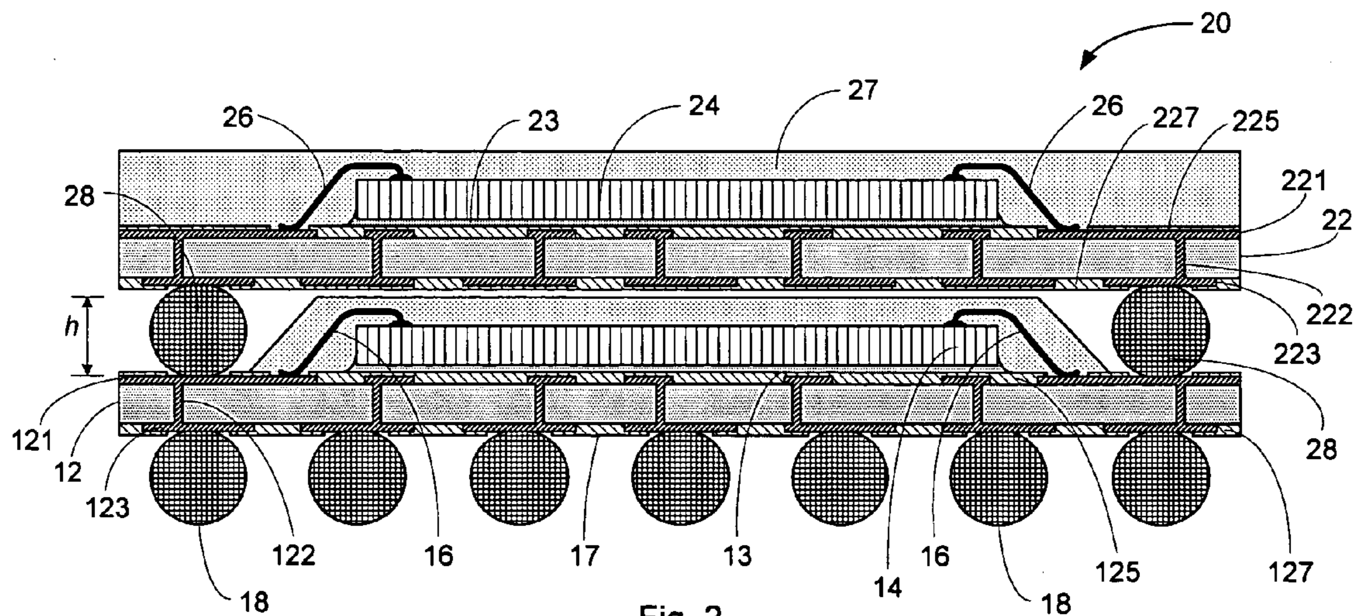
Fig. 2 PRIOR ART
