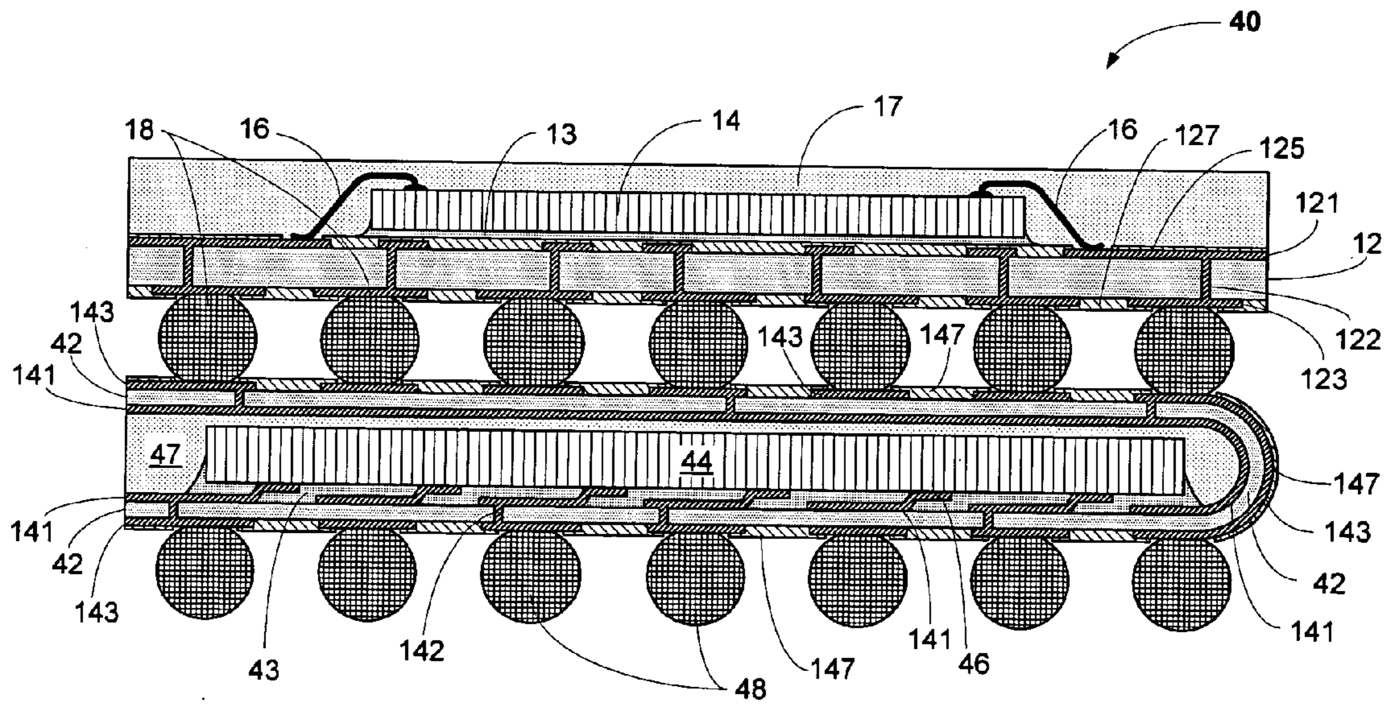
Fig. 4 PRIOR ART
