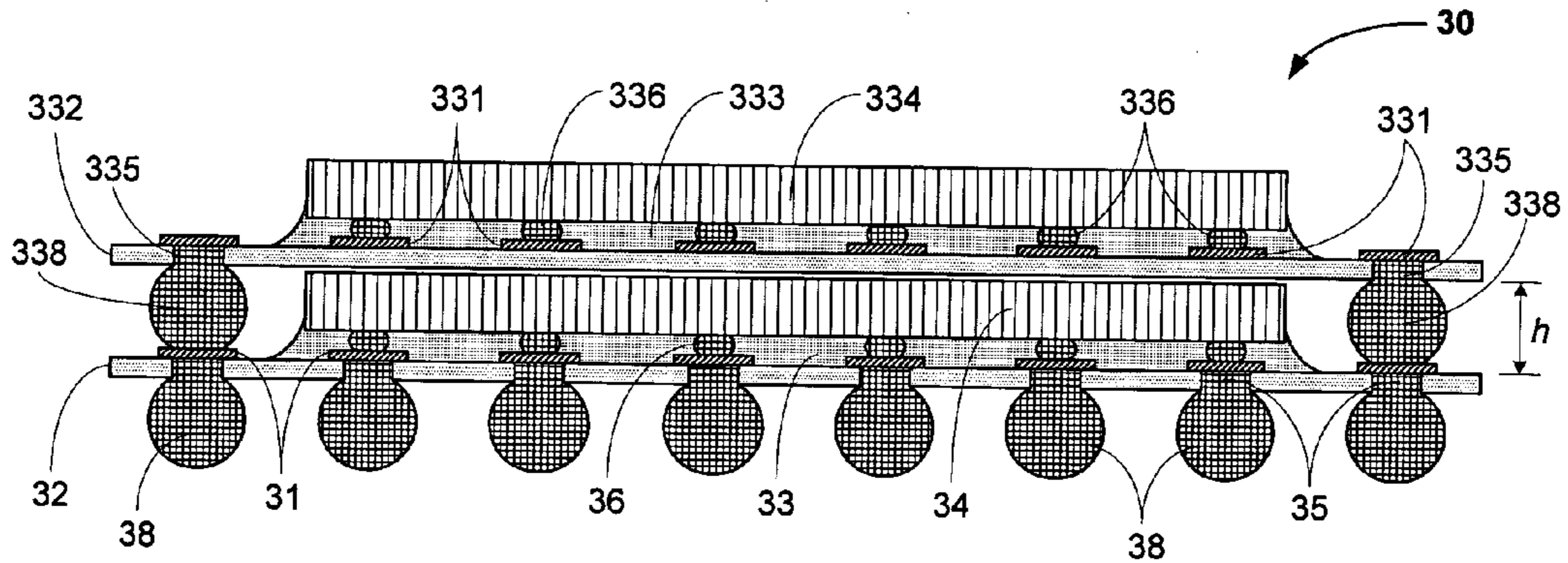
Fig. 3 PRIOR ART
