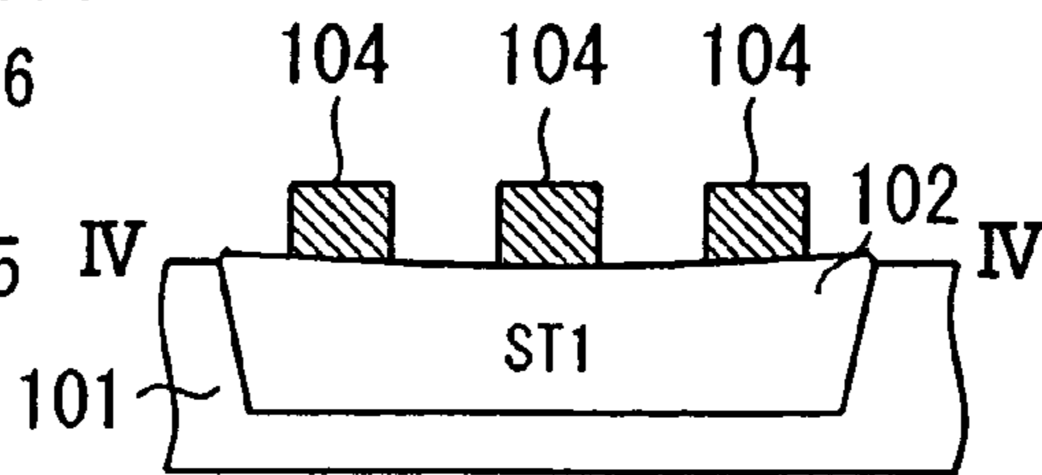
Fig. 13C (PRIOR ART)
