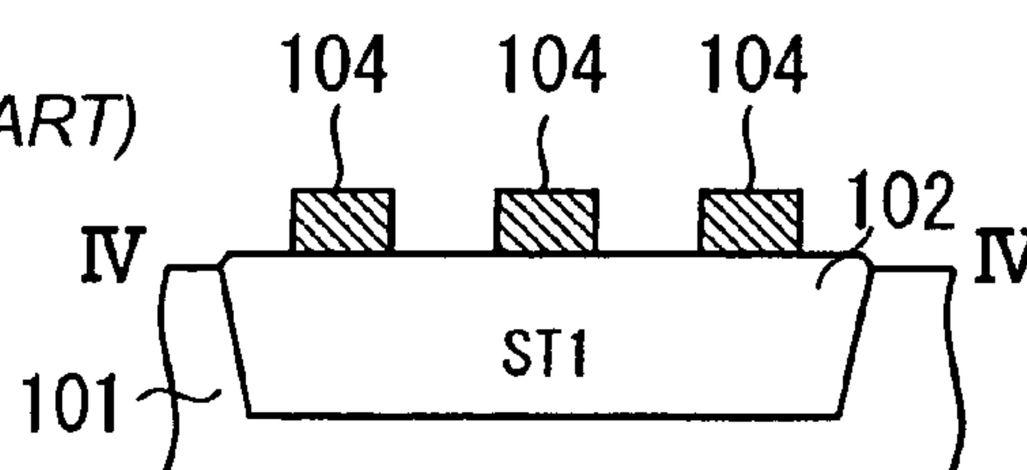
Fig. 13B (PRIOR ART)
