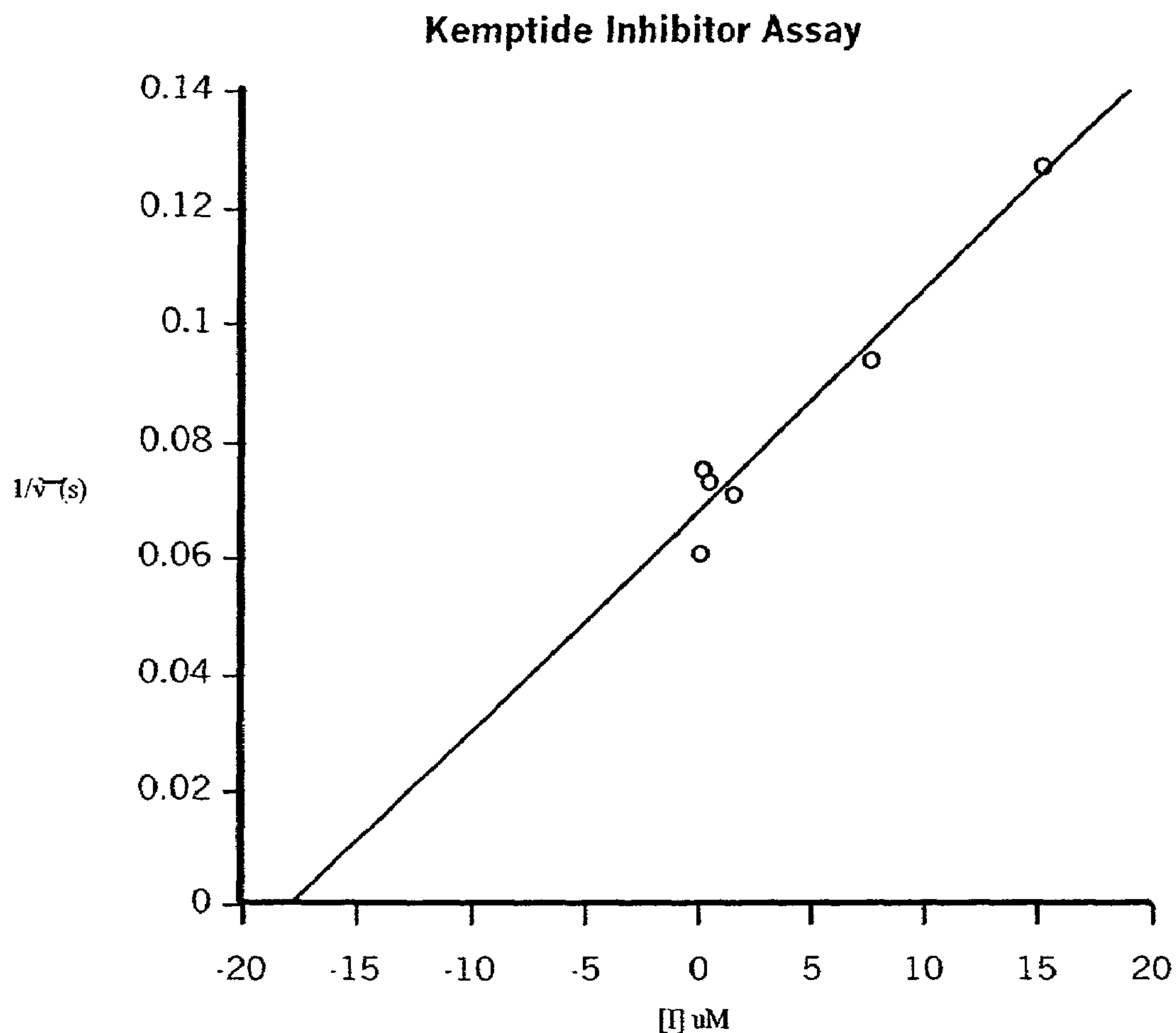
Inhibition assay for protein kinase A. Final concentrations for reaction components : ATP = 15 uM, kemptide = 25 uM, Mg 2+ = 10mM, Tris-HCl = 40 mM, bovine serum albumin (from enzyme mix) 150 ug/mL. All reactions were carried out at pH 7.5 and with a final enzyme concentration of 0.35 nM for 2 minutes at 30 degrees Celsius.
