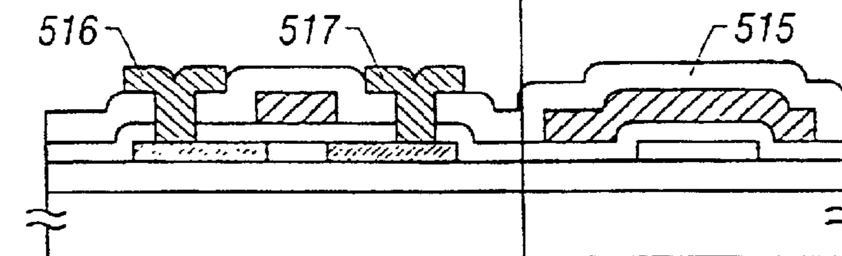
FIG. 5F A LEFT PART A RIGHT PART
