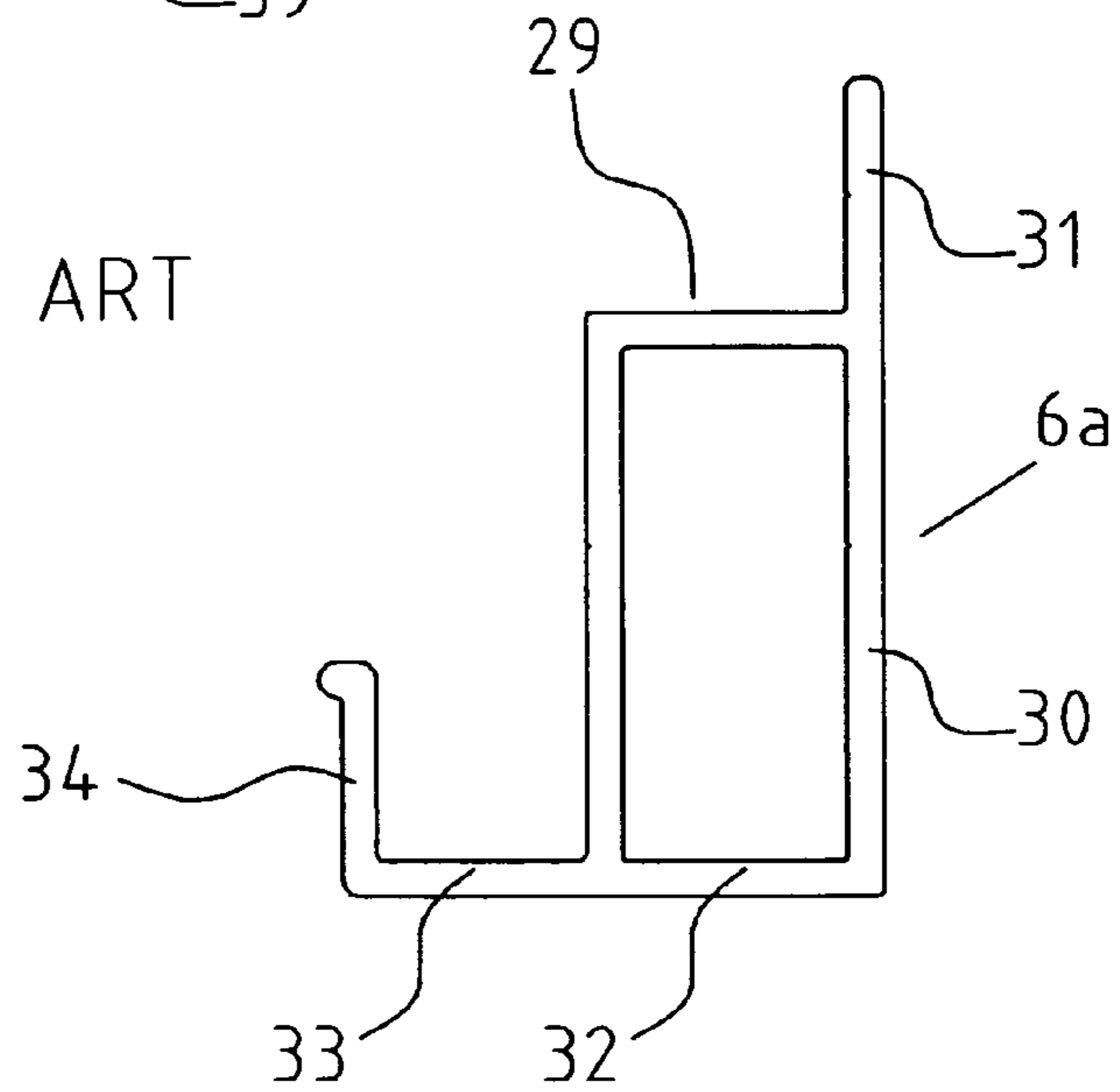
PRIOR ART Fig. 6
