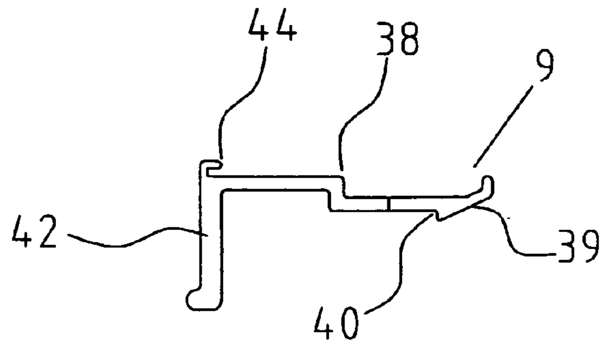
PRIOR ART Fig. 5
