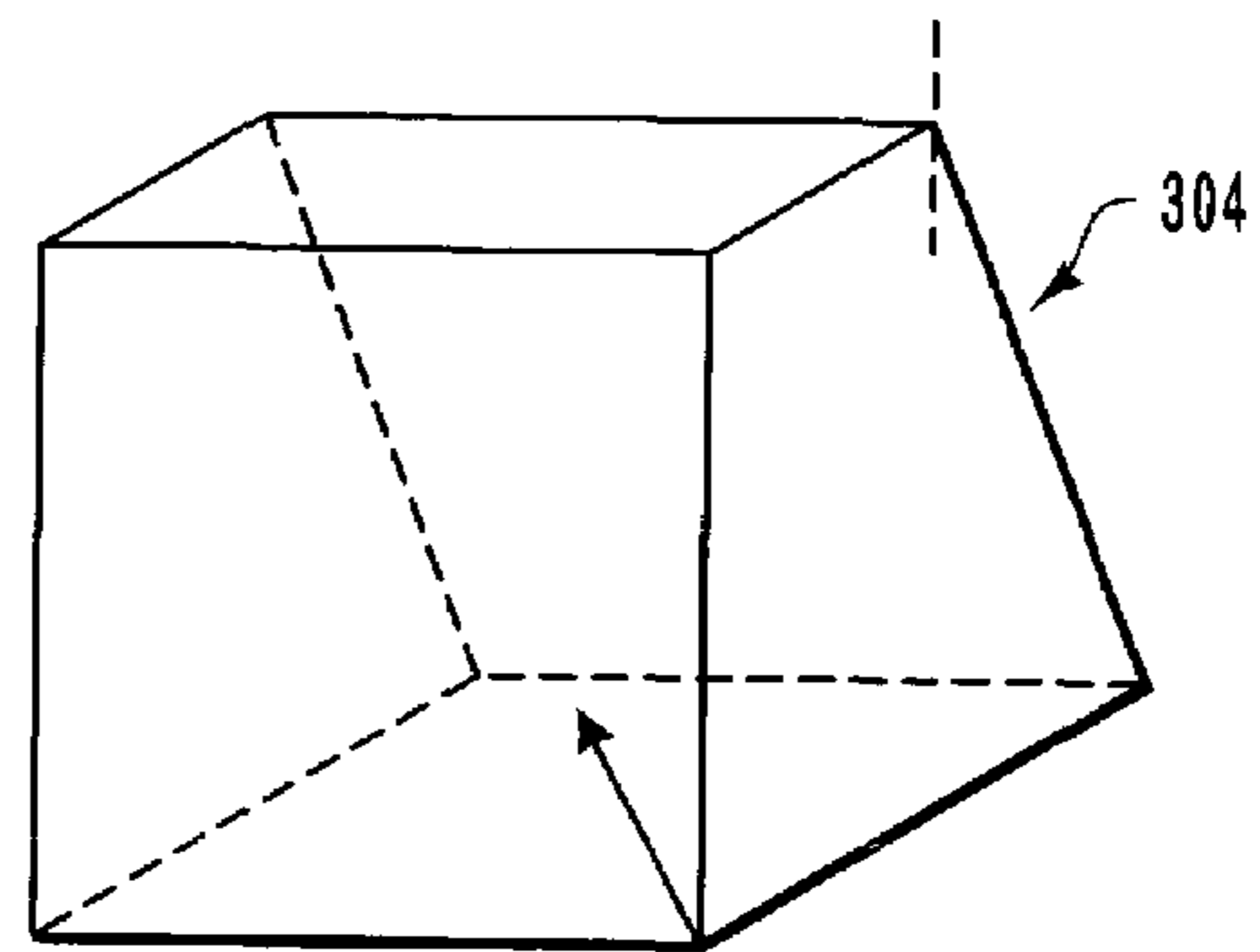
OPTICAL AXIS 45° FIG. 3B
