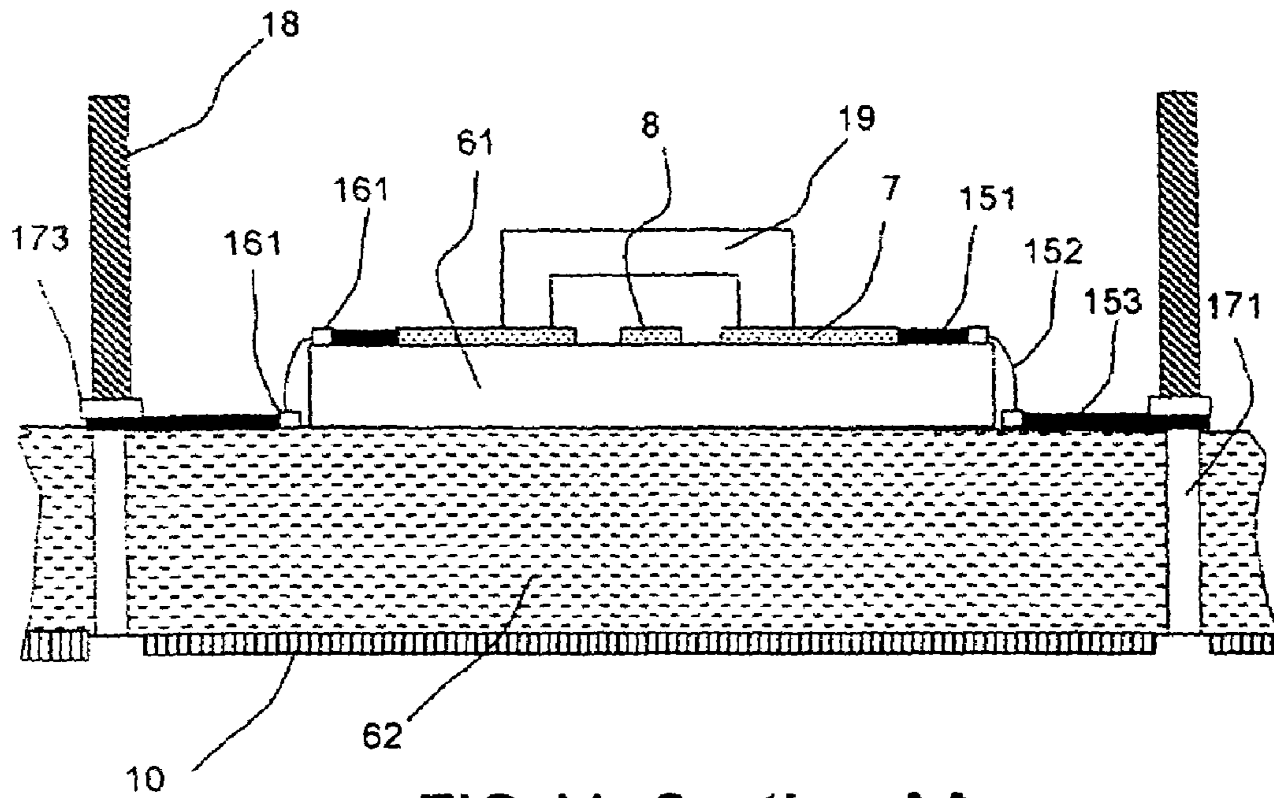
FIG. 11- Section AA
