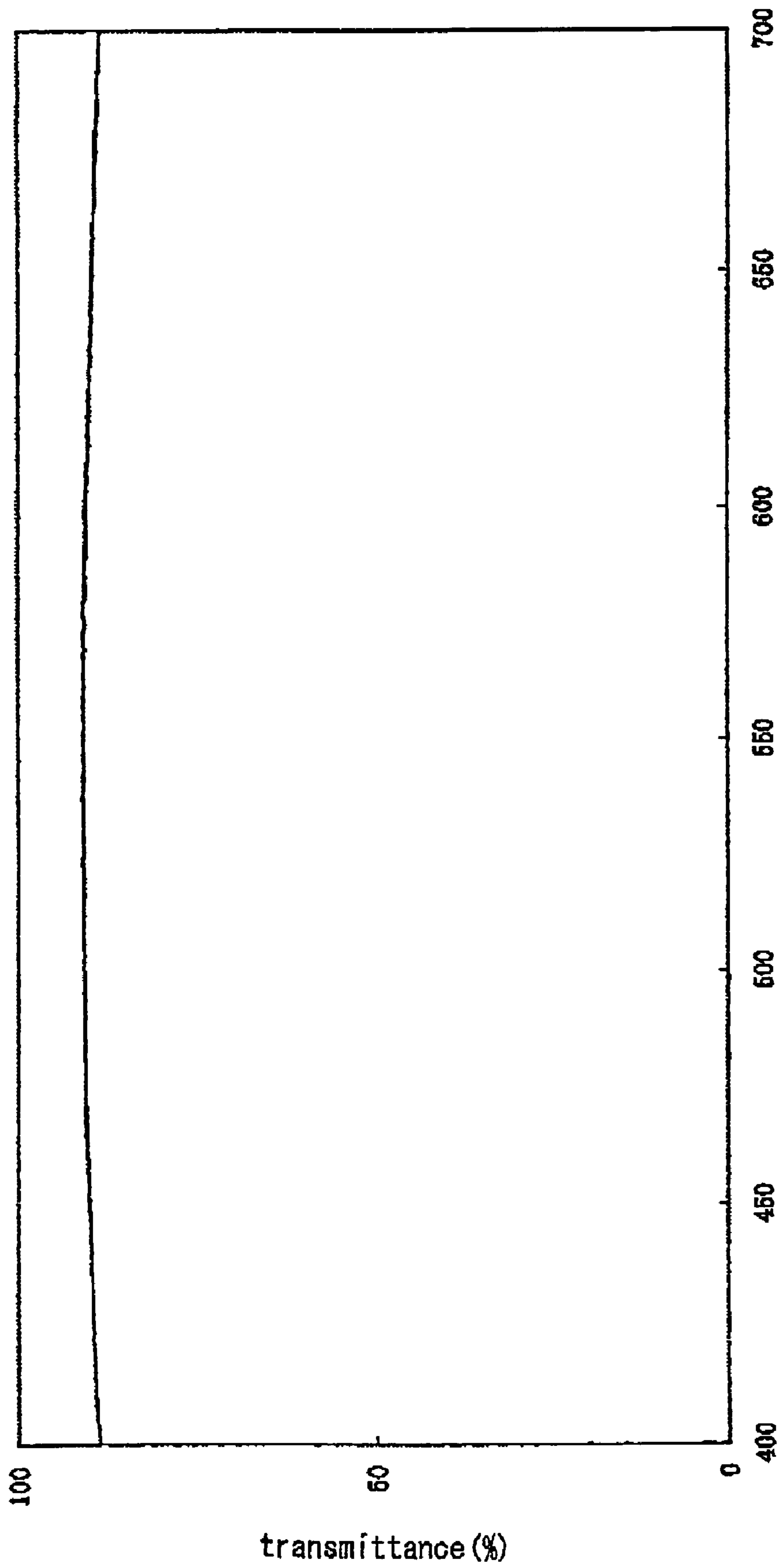
wavelength (nm)
