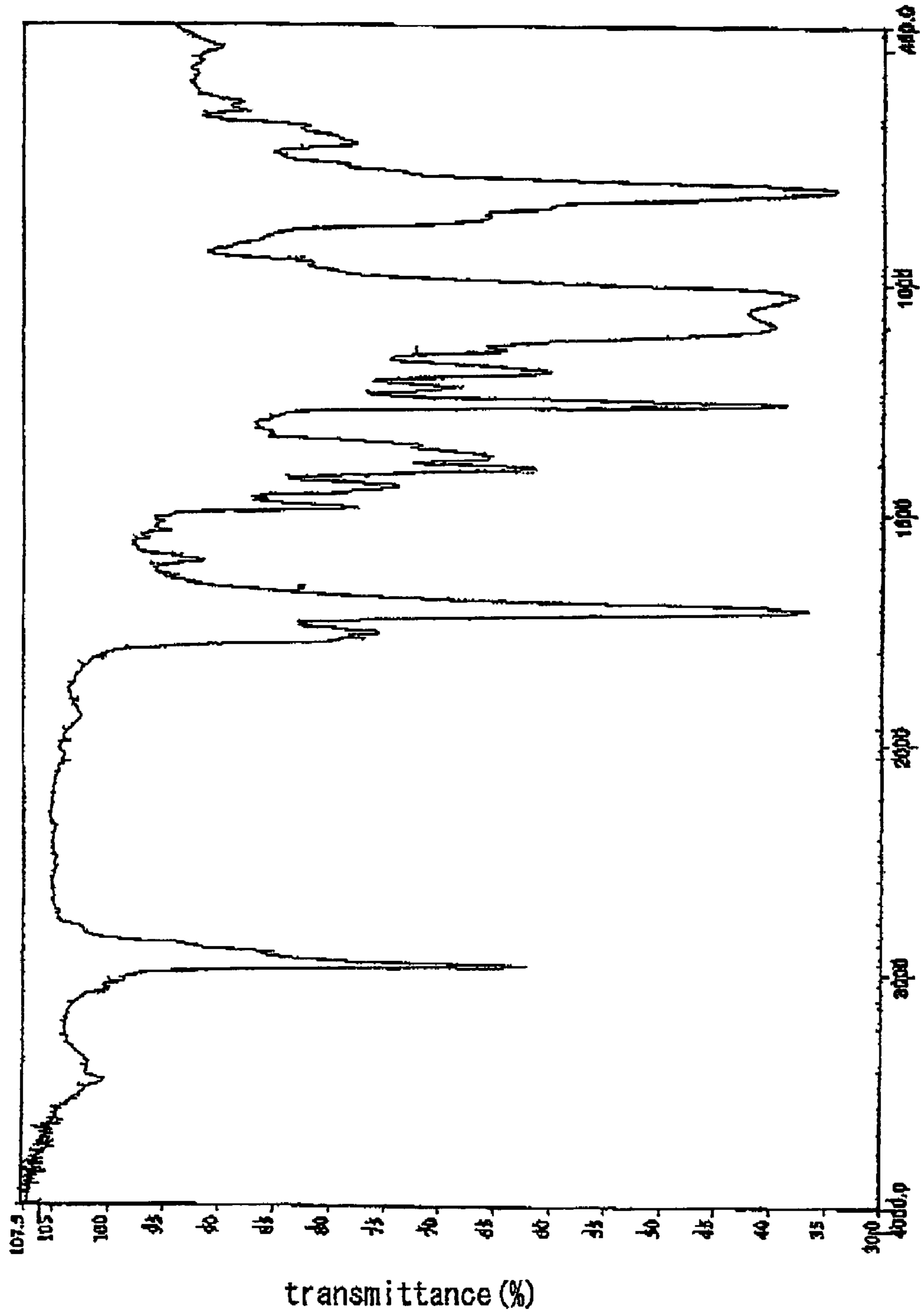
wavenumber (cm -1 )
