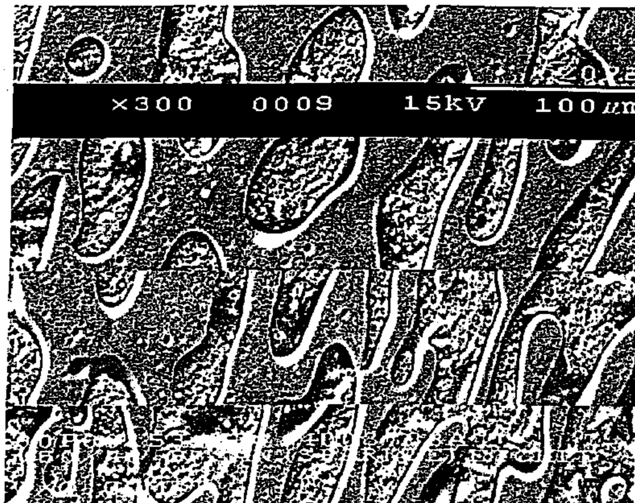
NaOH etched Blend of 60% polycarbonate and 40% SAN at 300X viewed by SEM
