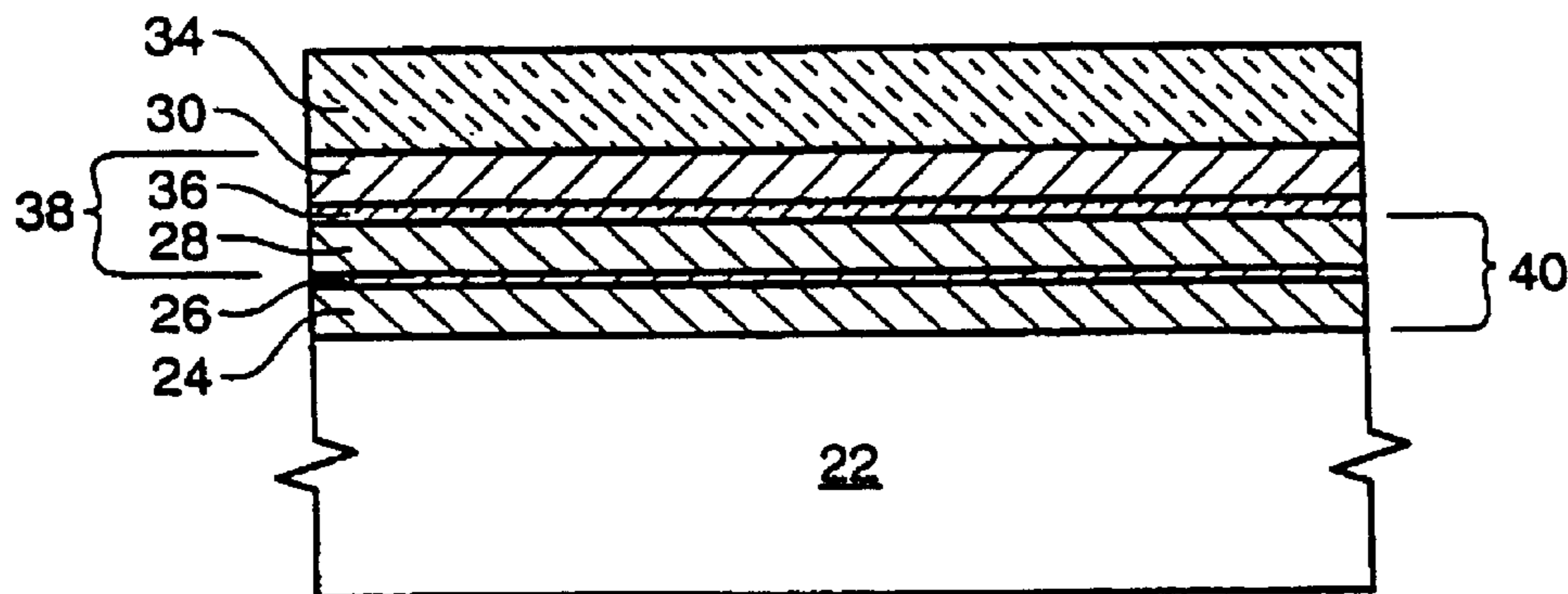
FIG. 3 (PRIOR ART)
