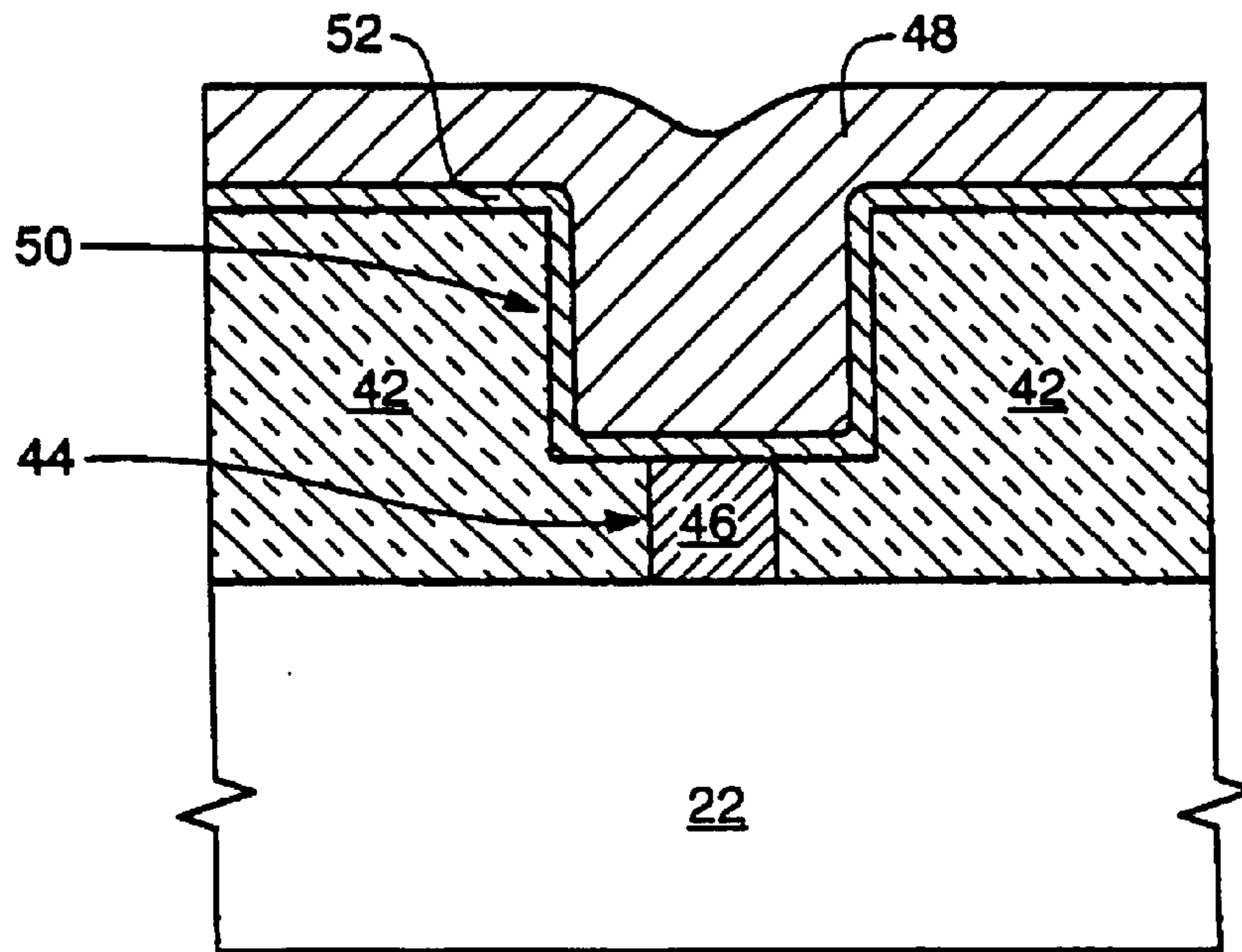
FIG. 7 (PRIOR ART)
