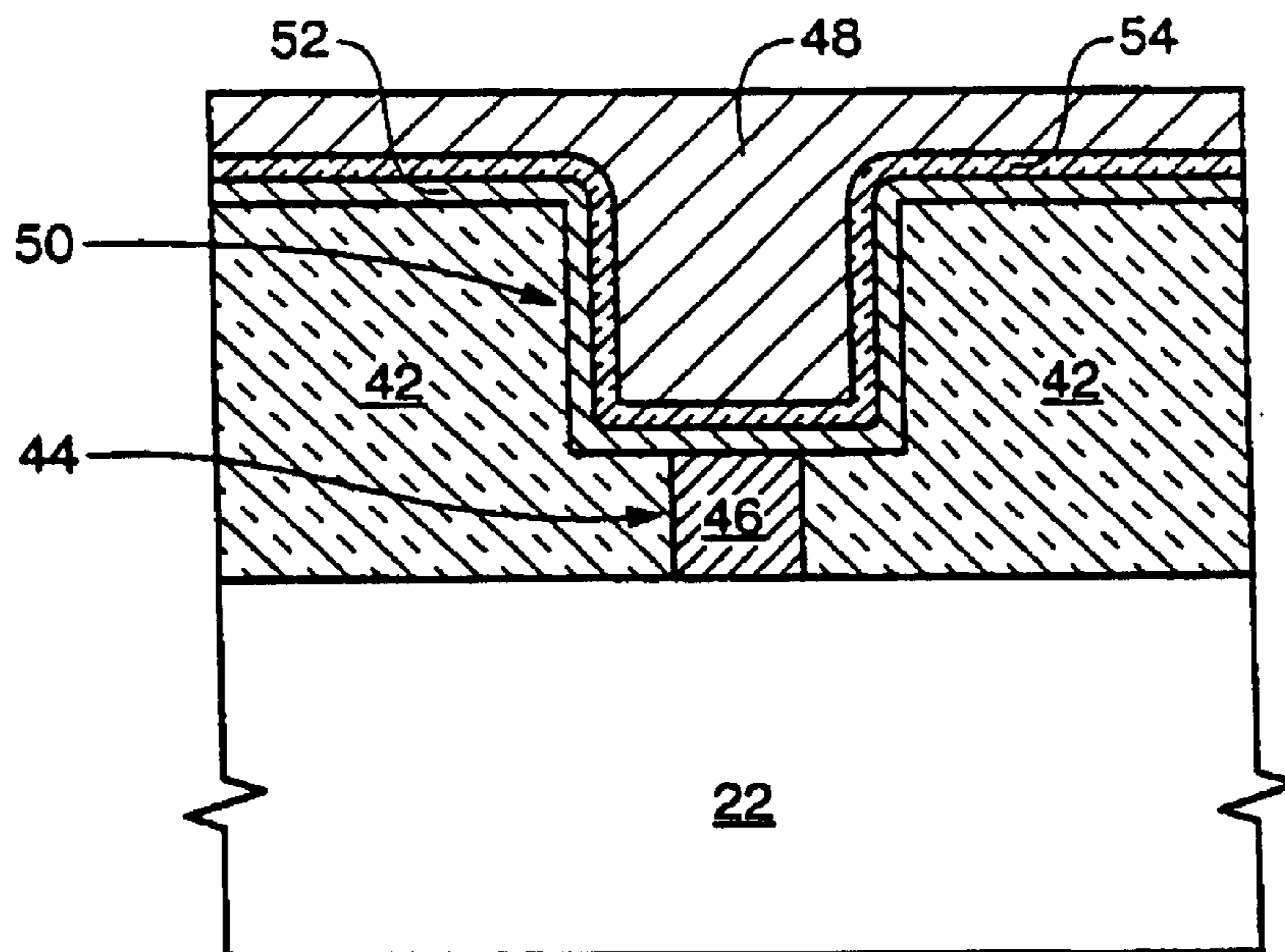
FIG. 8 (PRIOR ART)
