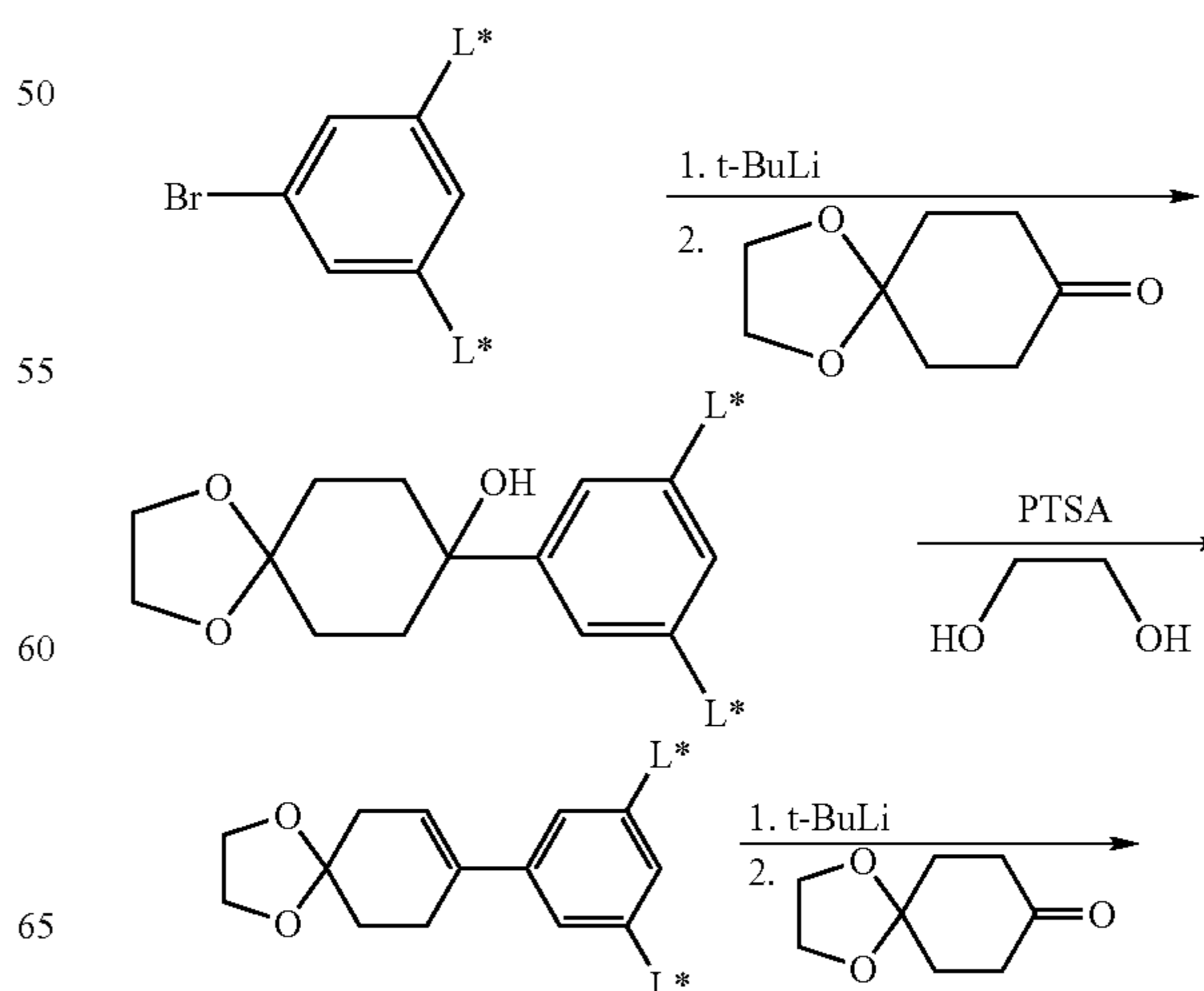
Scheme 1:
