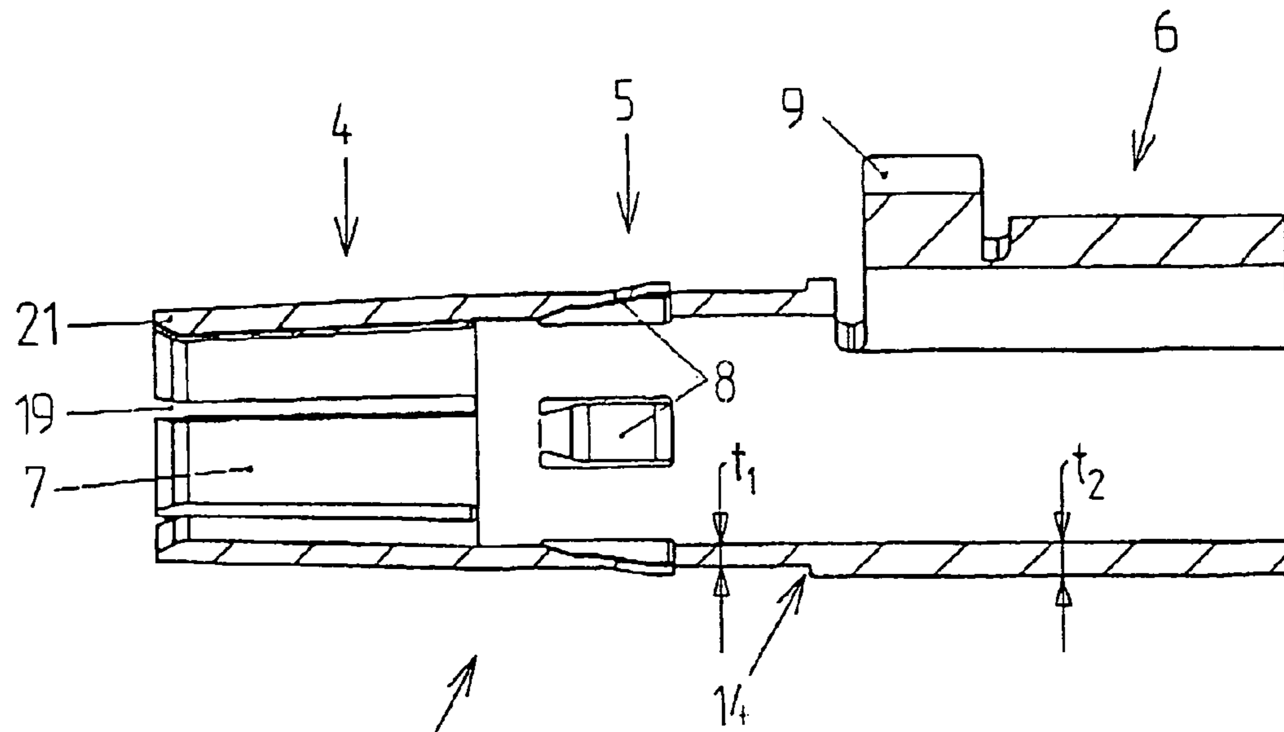
3 Fig 4a (45° cross section in lengthwise axis)
