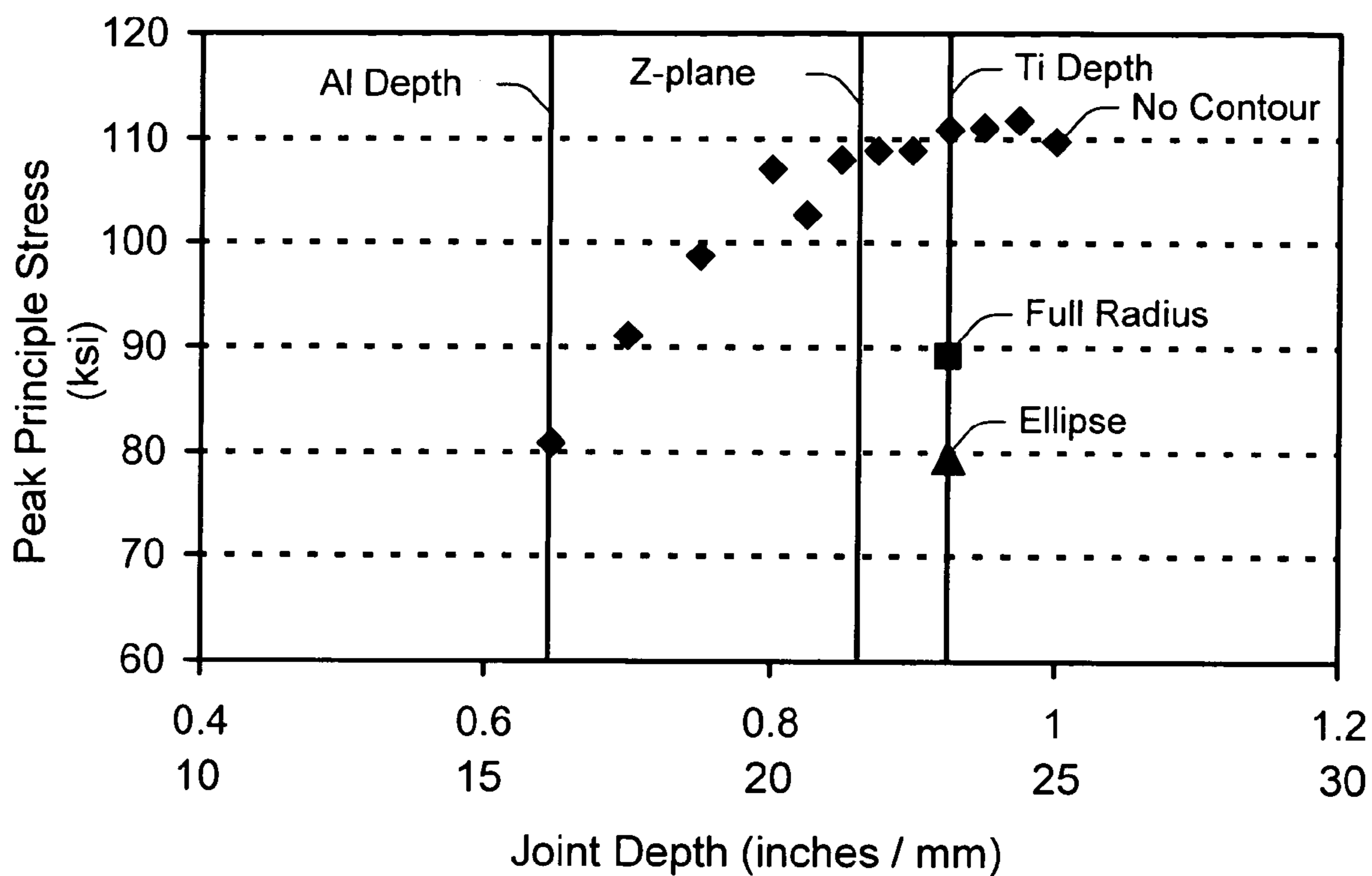
Stress versus Joint Depth (e.g., ~73 mm Ti Wheel Length and ~94 mm Diameter)
