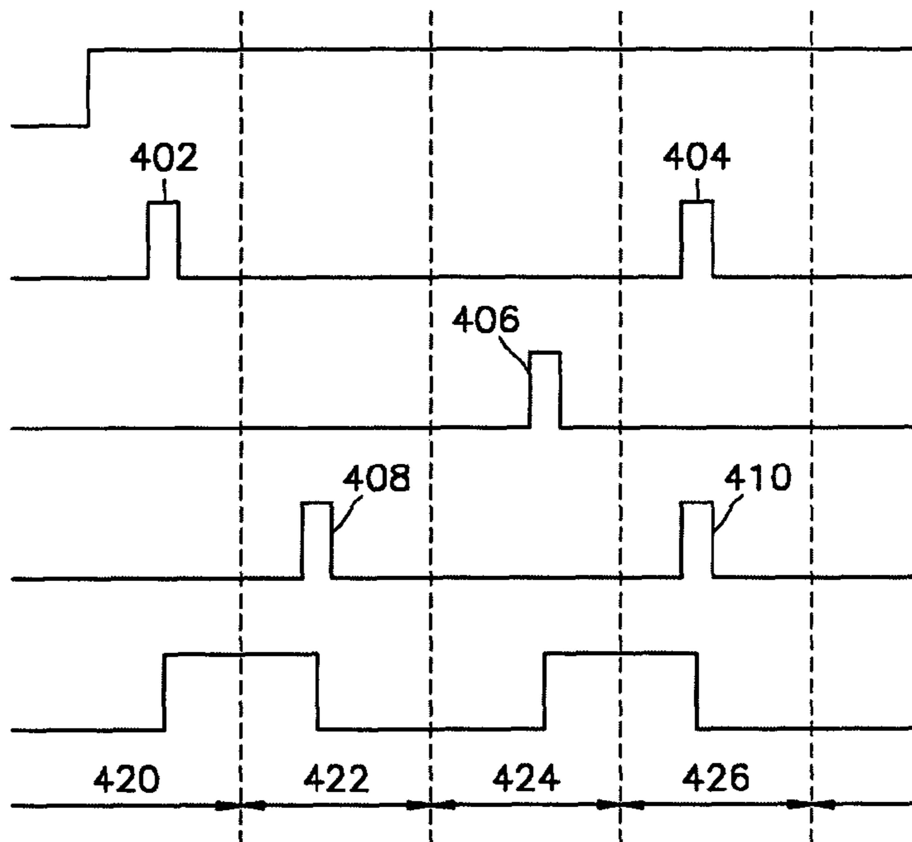
FIG. 4D POWER-OFF SIGNAL
