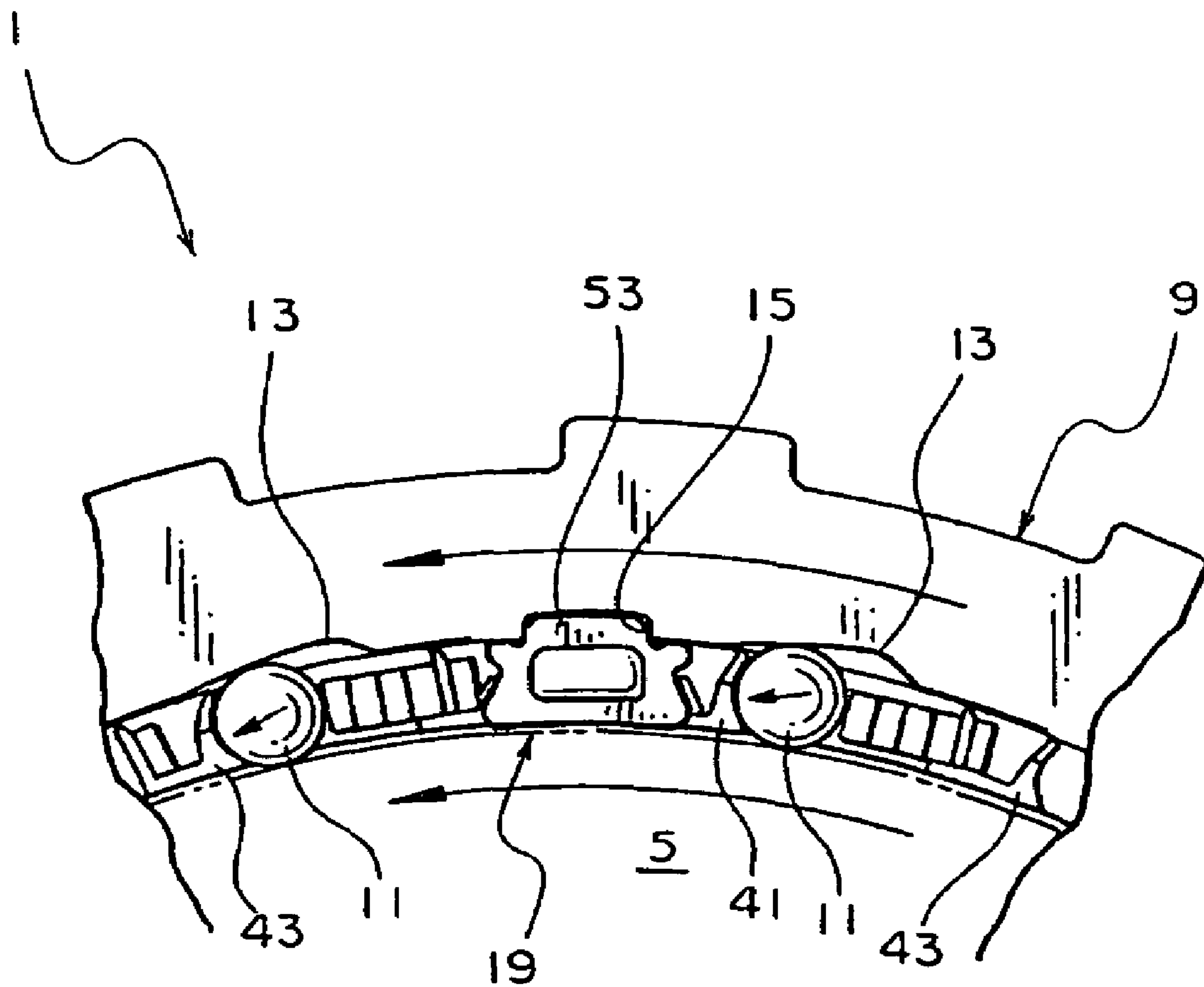
FIG. 15 PRIOR ART
