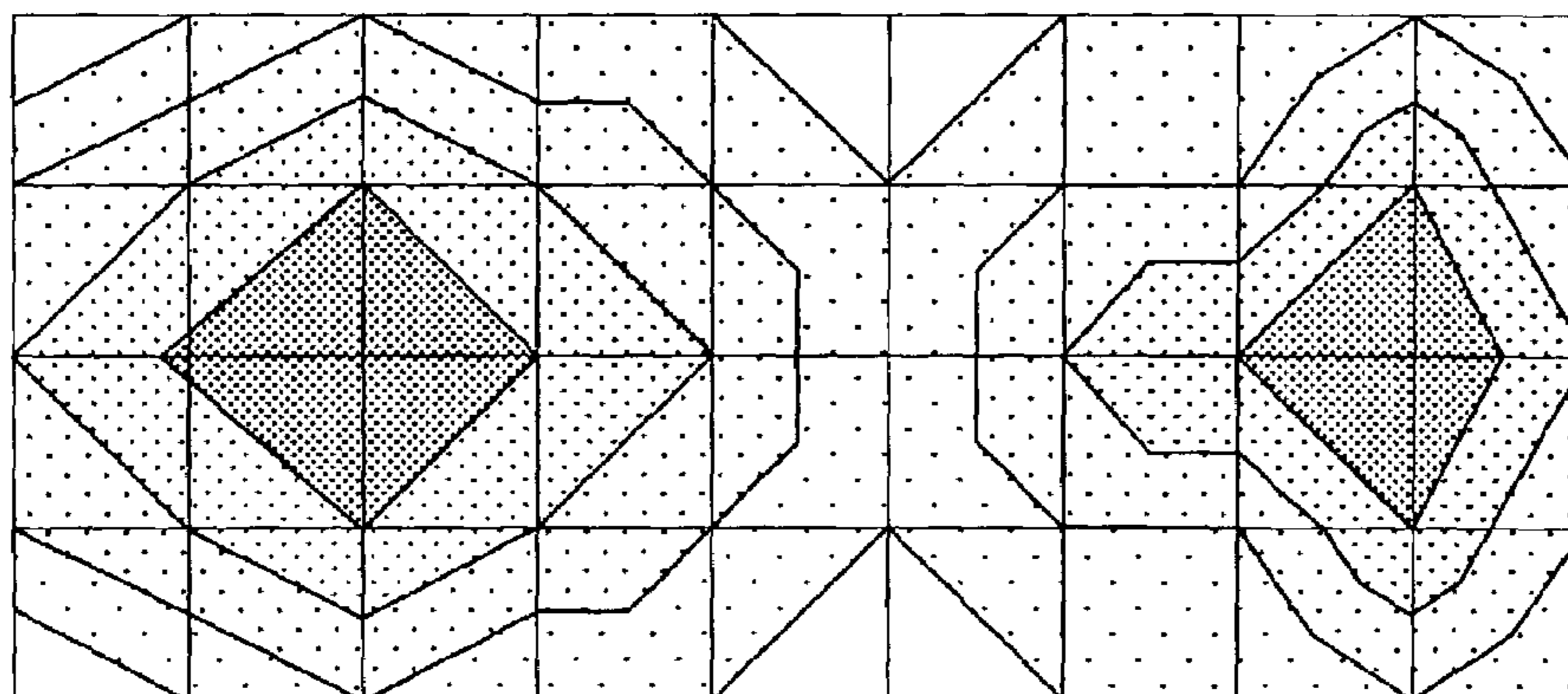
MEASUREMENT RESULT OF PLATE THICKNESS DISTRIBUTION (EXAMPLE)
