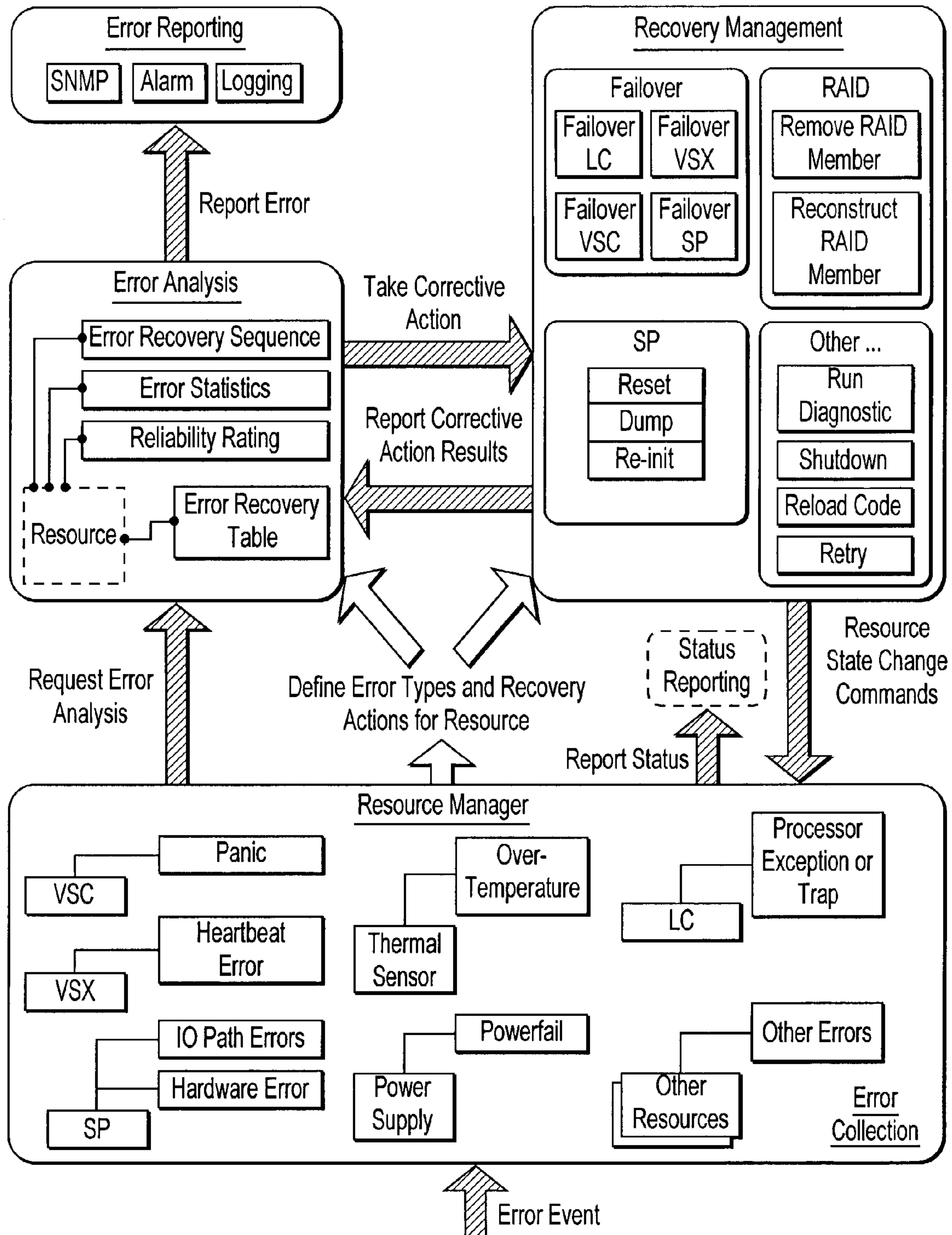
FIG. 1 Error Recovery Architecture
