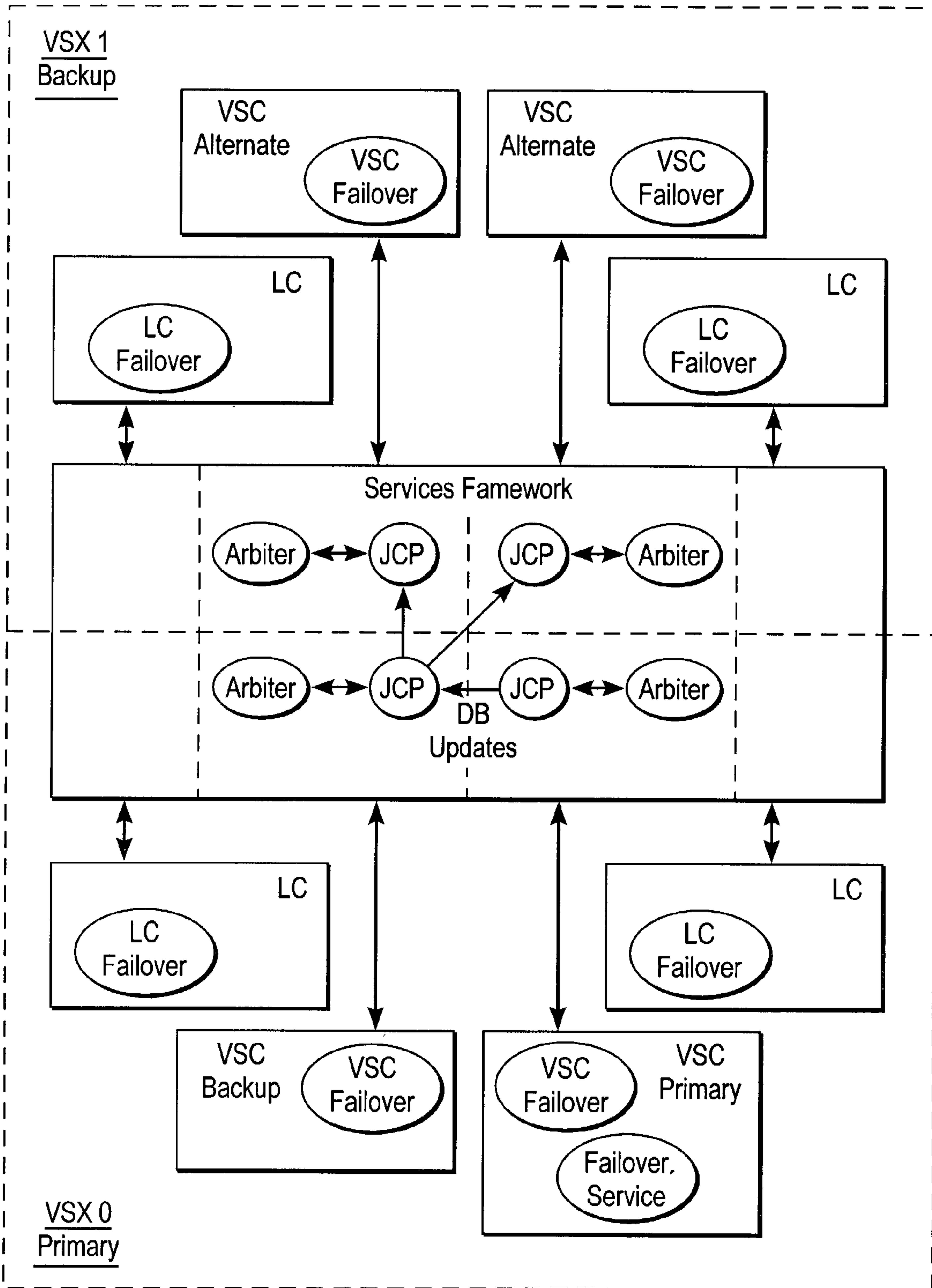
FIG. 21A Failover Service Architecture
