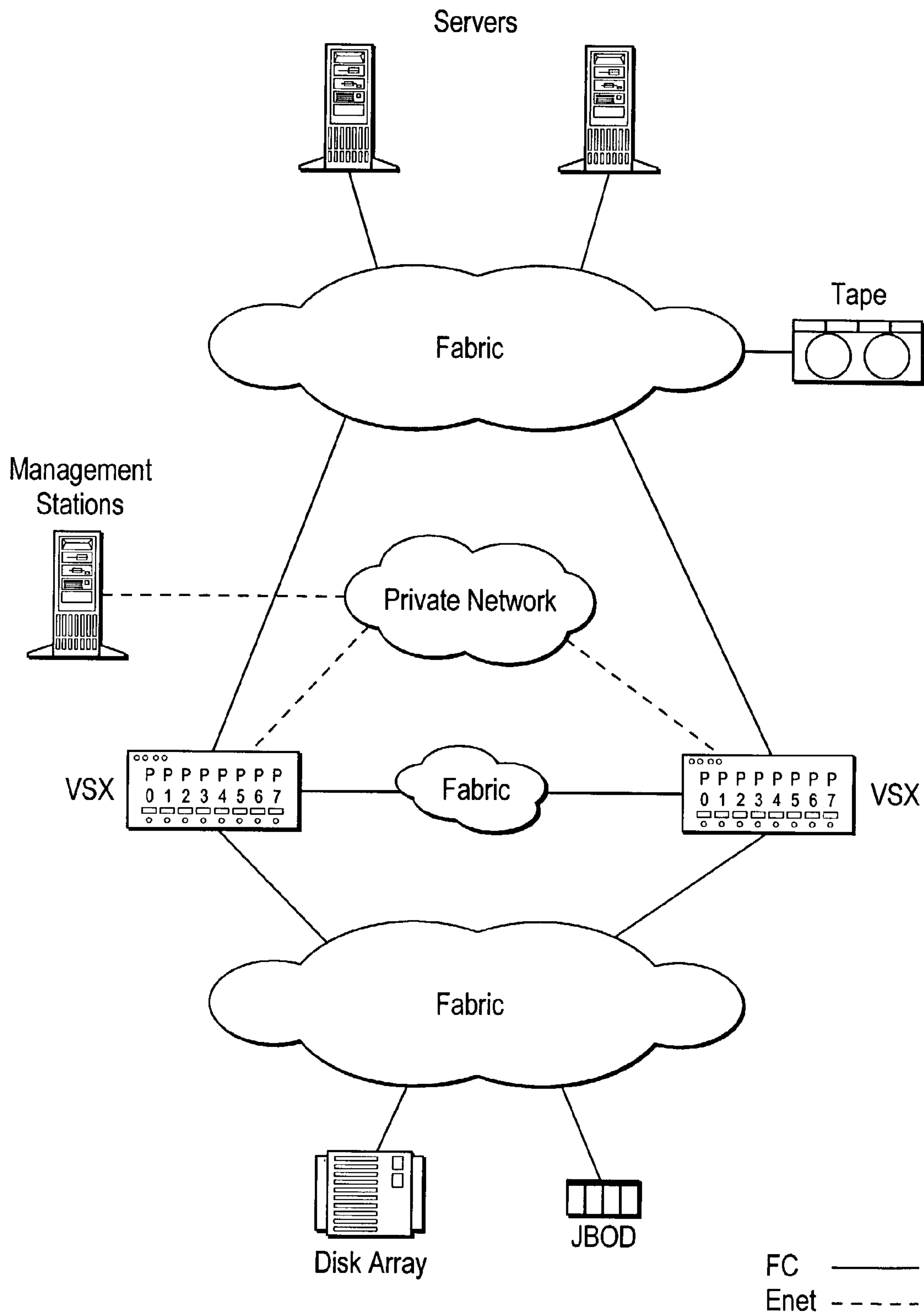
FIG. 36C Physical Setup for VSX-HA — Variation 3
