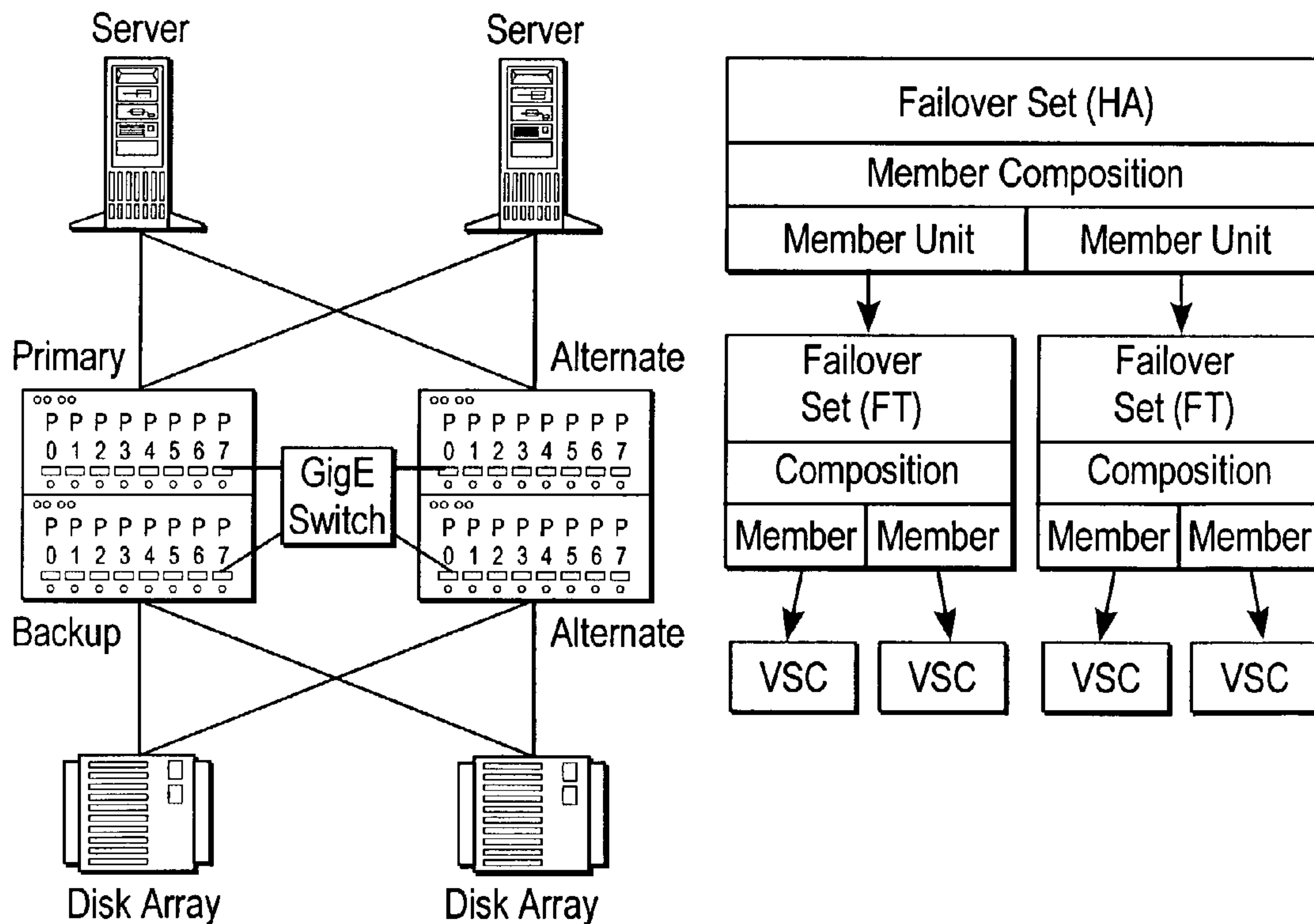
FIG. 29 Hierarchical HA Configuration
