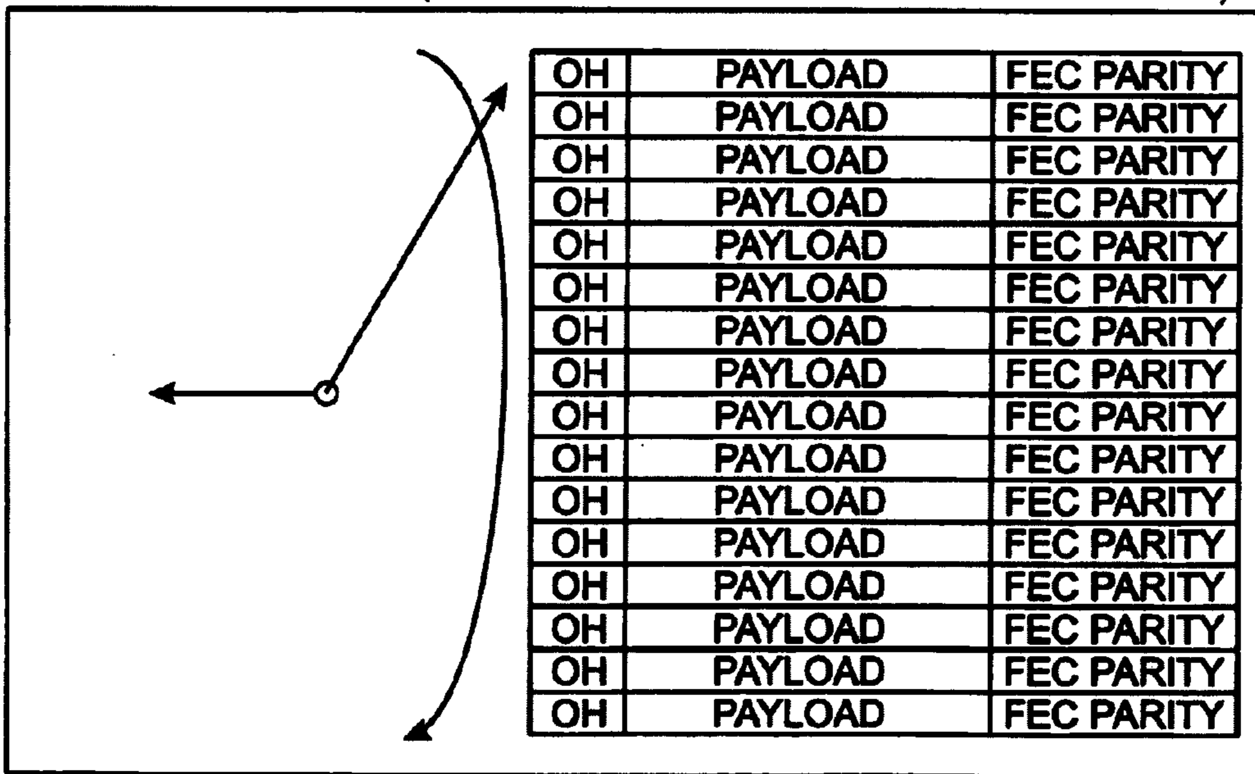
Fig. 2a OTUK ROW (SHOWN BEFORE INTERLEAVED TRANSMISSION)
