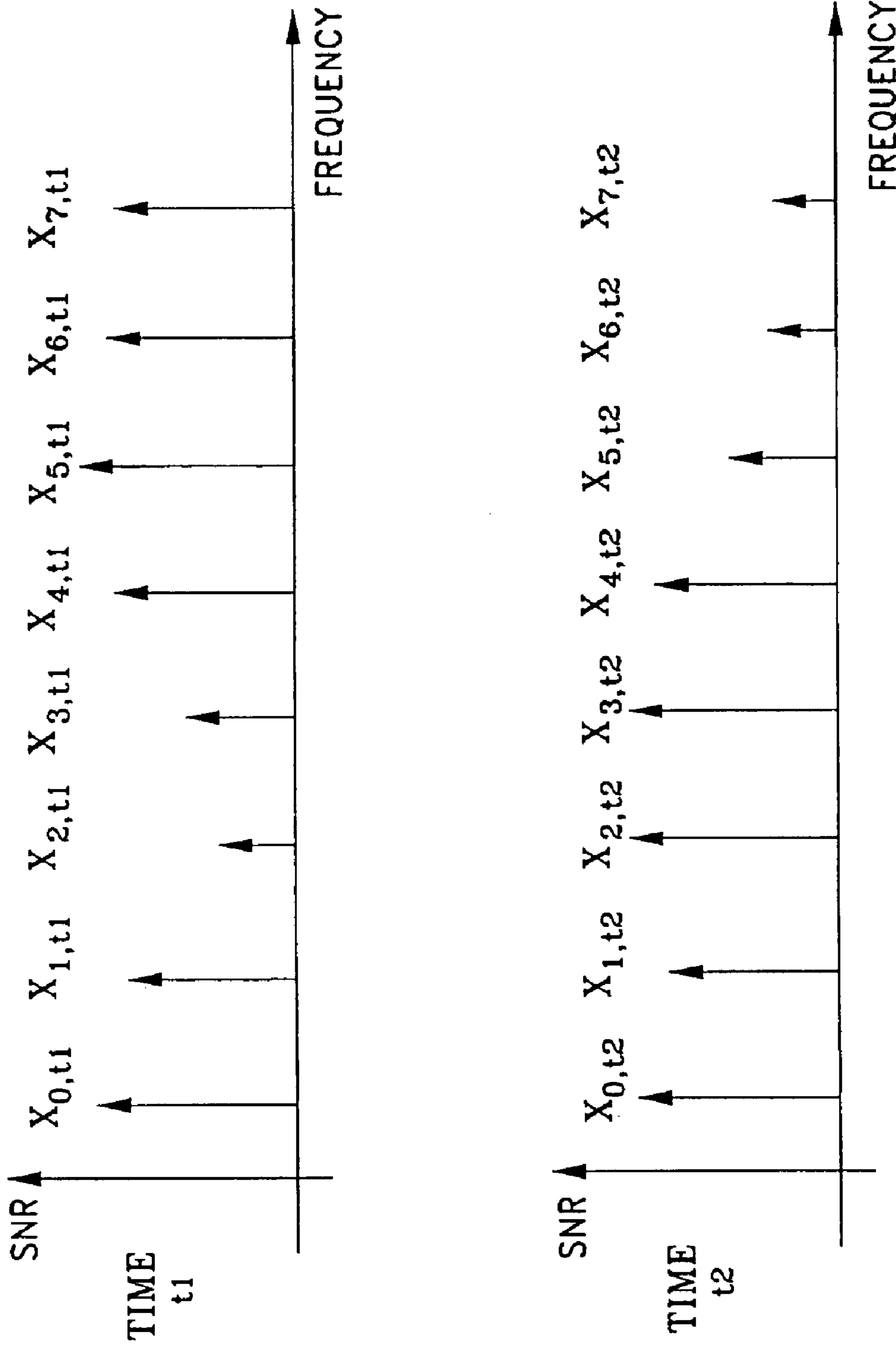
FIG. 2 (PRIOR ART)
