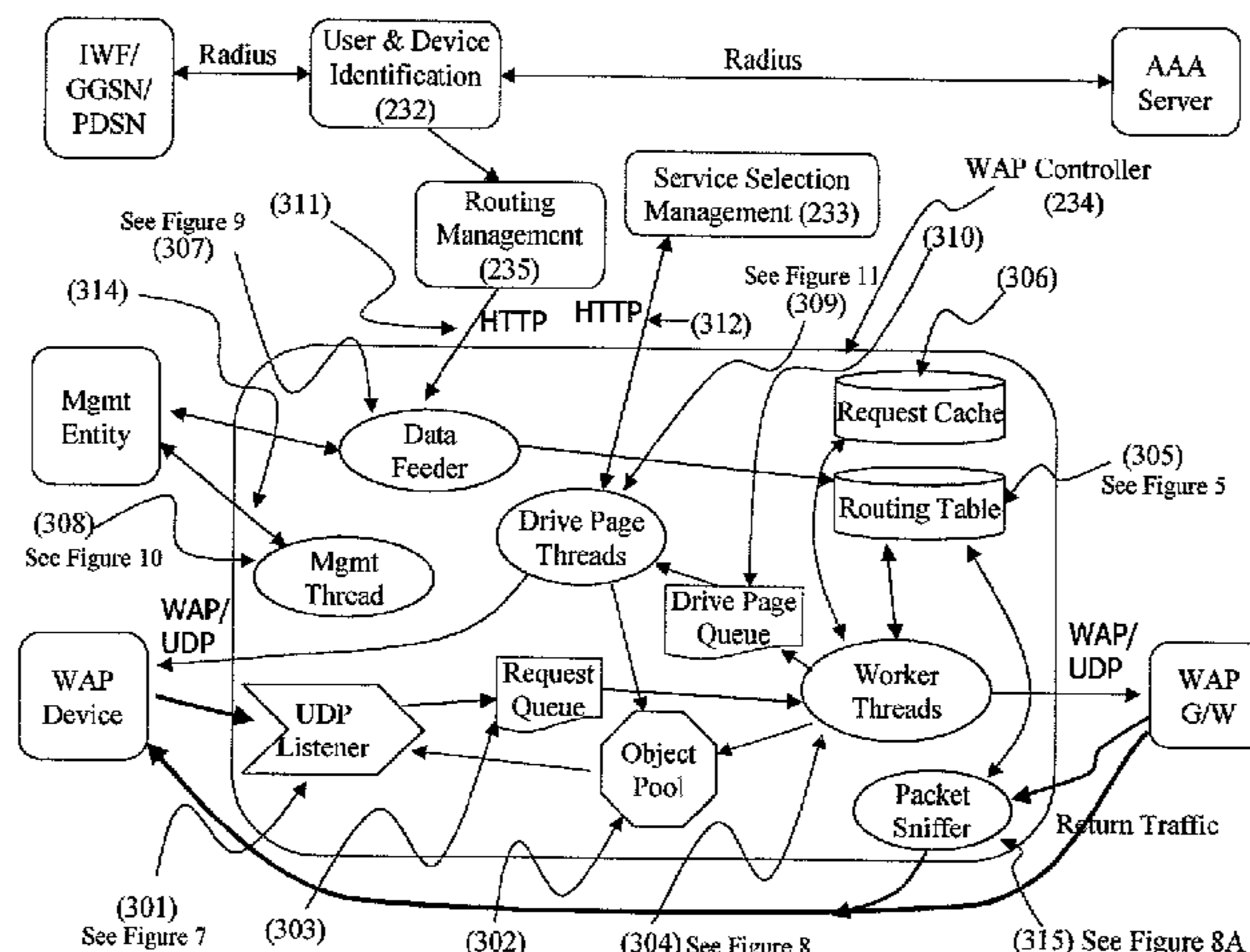
WAP Controller (234) Block Diagram
