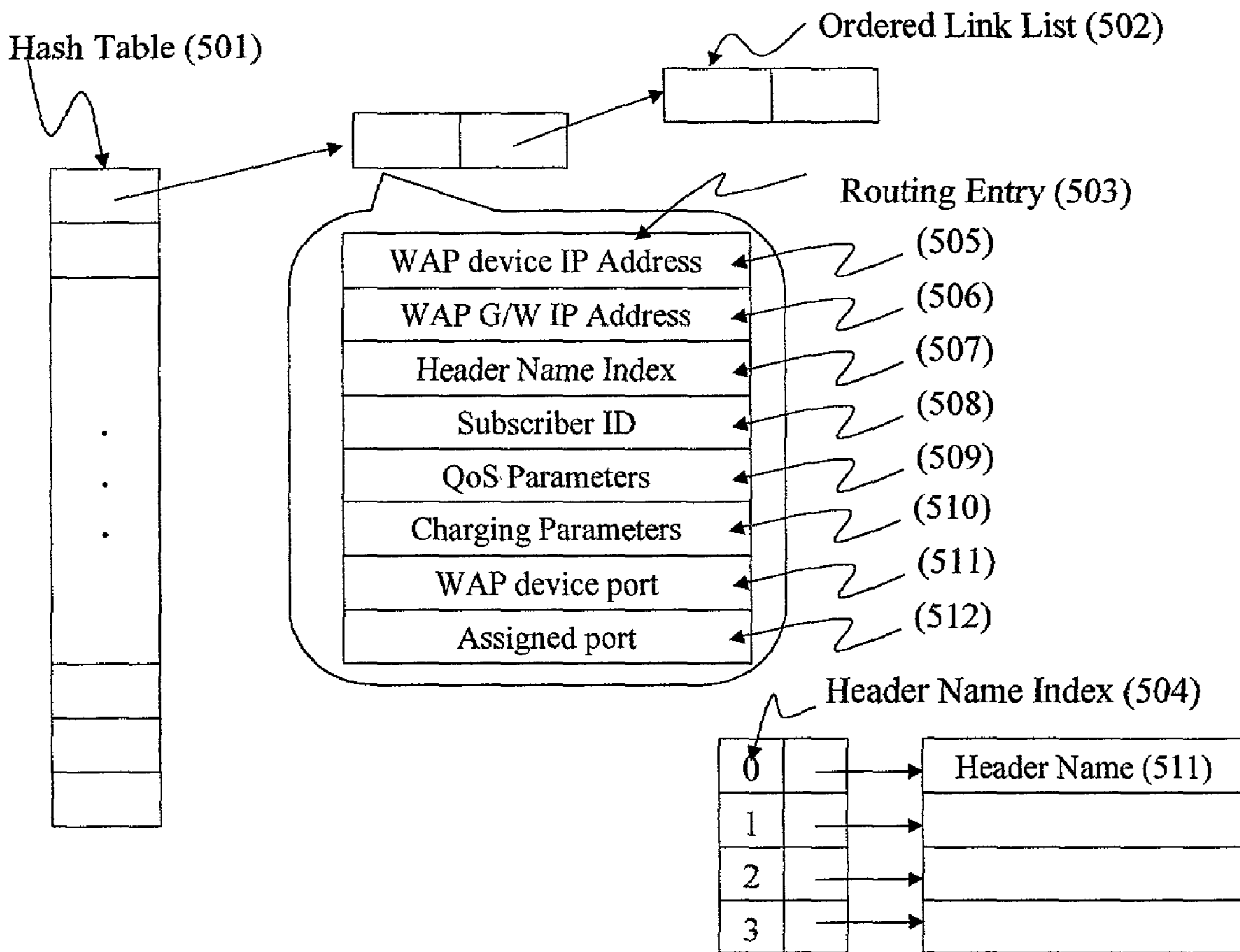
Figure 5 WAP Controller (234) Routing Table (305) Data Structure
