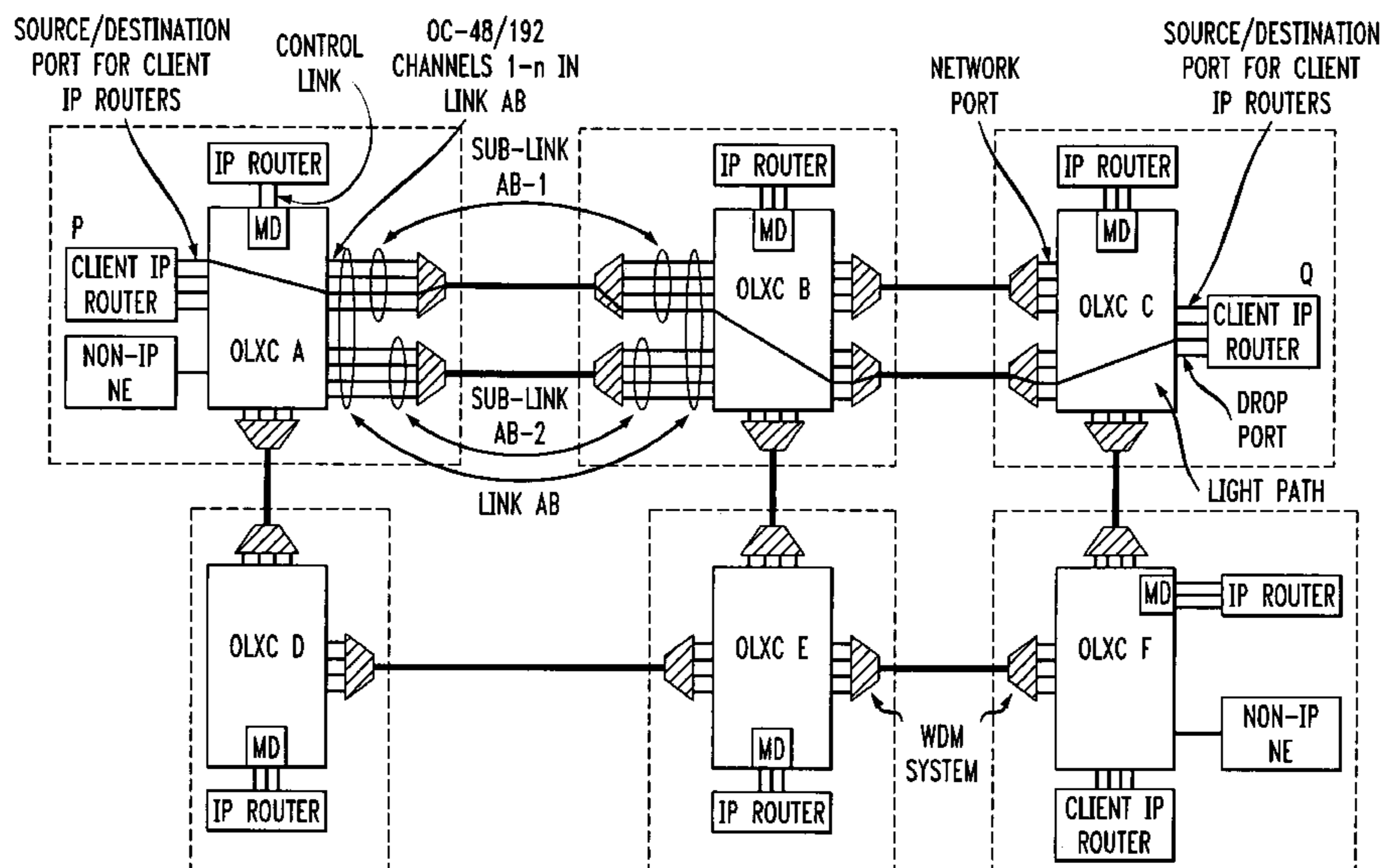
EXAMPLE OPTICAL NETWORK ILLUSTRATING DEFINED NETWORK ELEMENTS
