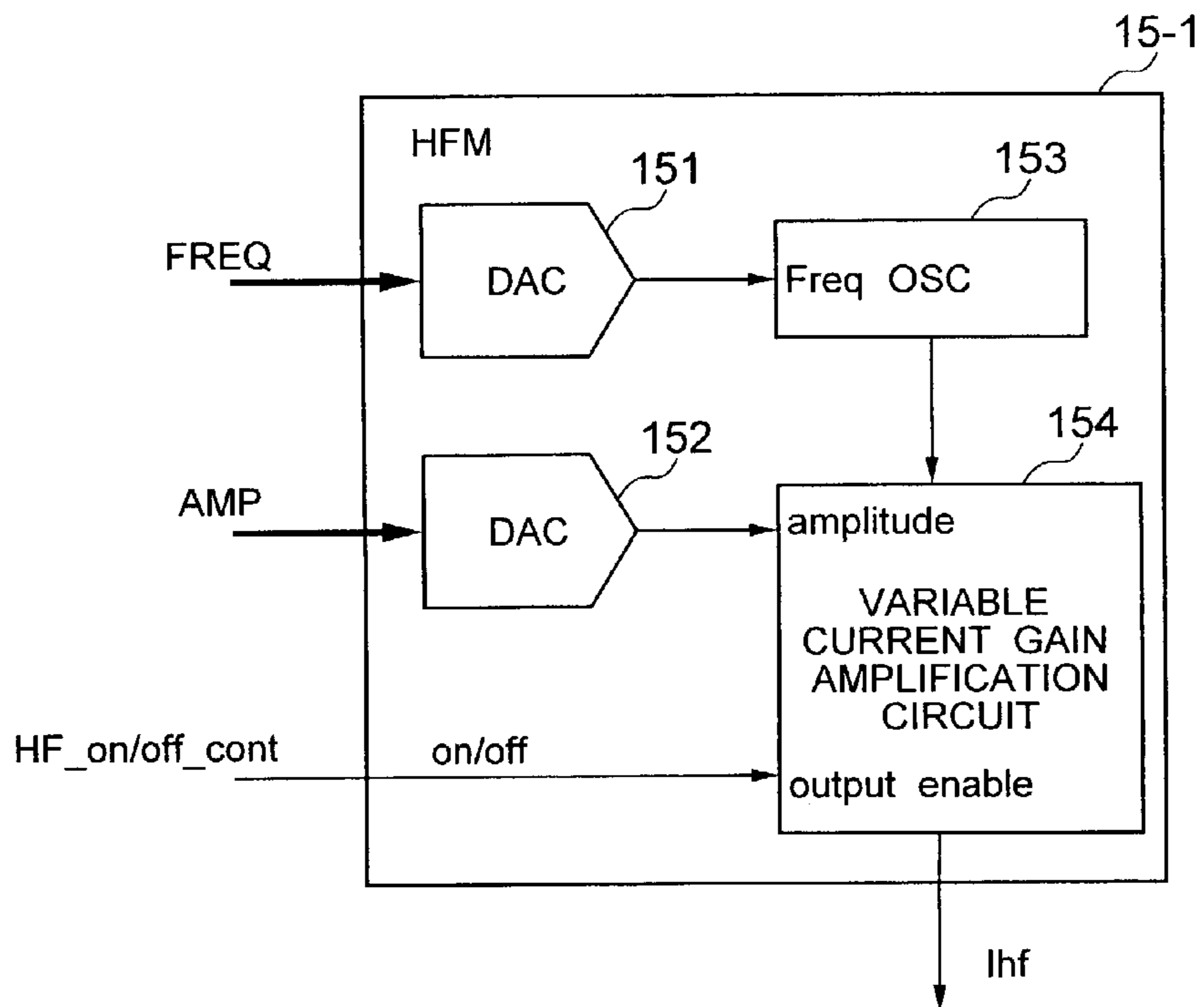
CONFIGURATION OF HIGH-FREQUENCY COMPONENT GENERATION CIRCUIT (HFM) 15-1
