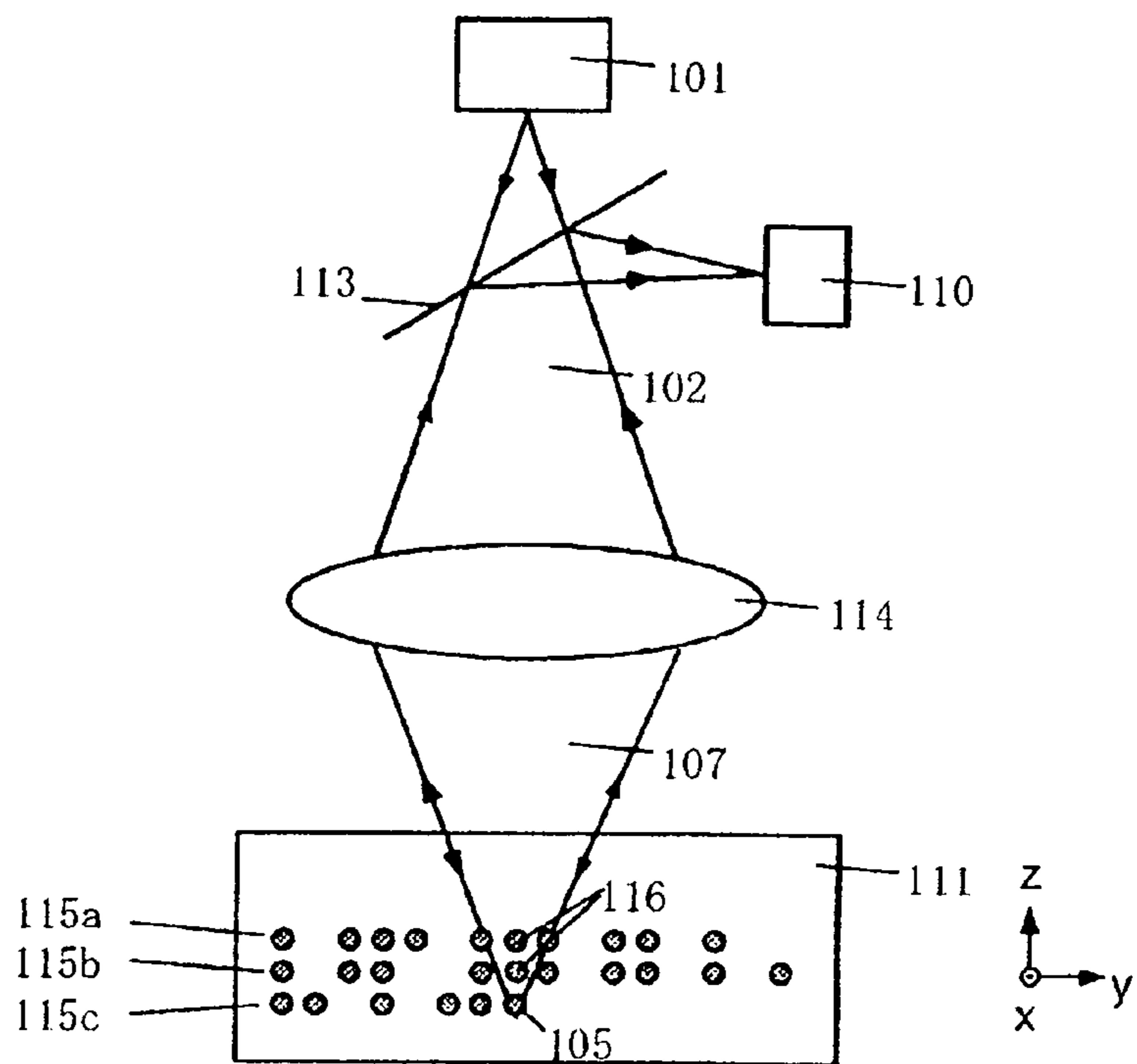
Fig. 8 PRIOR ART
