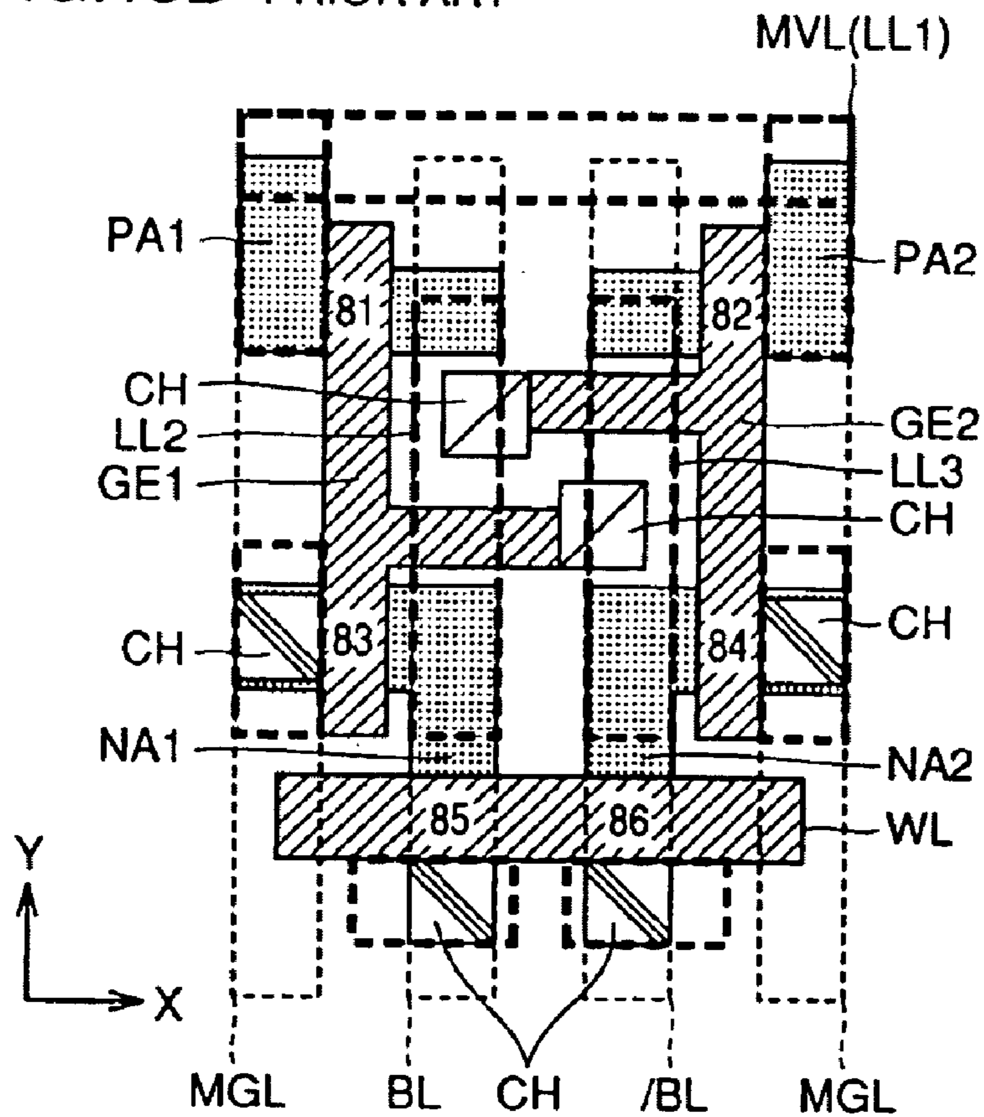
FIG. 13B PRIOR ART
