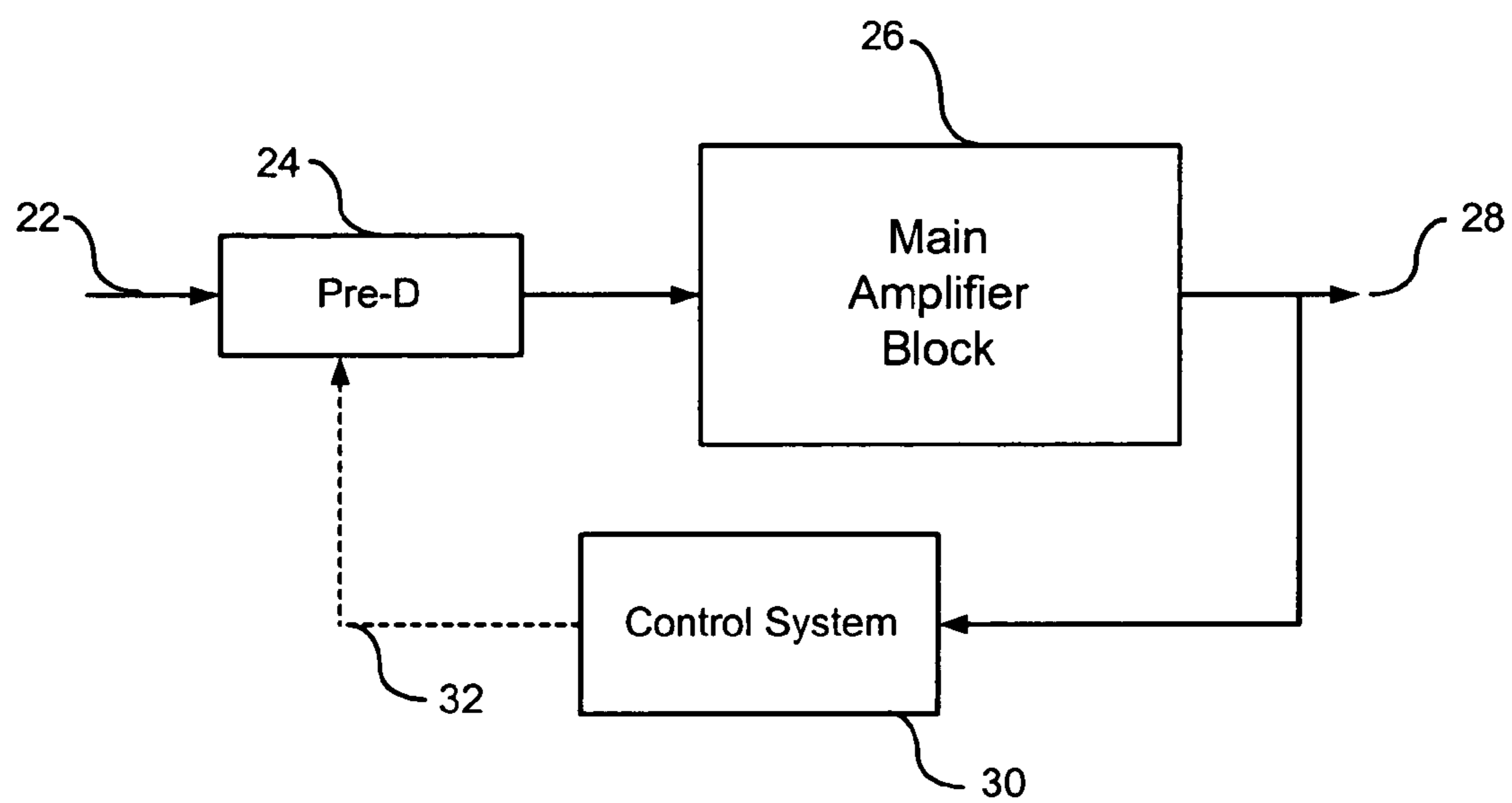
FIG. 6 PRIOR ART
