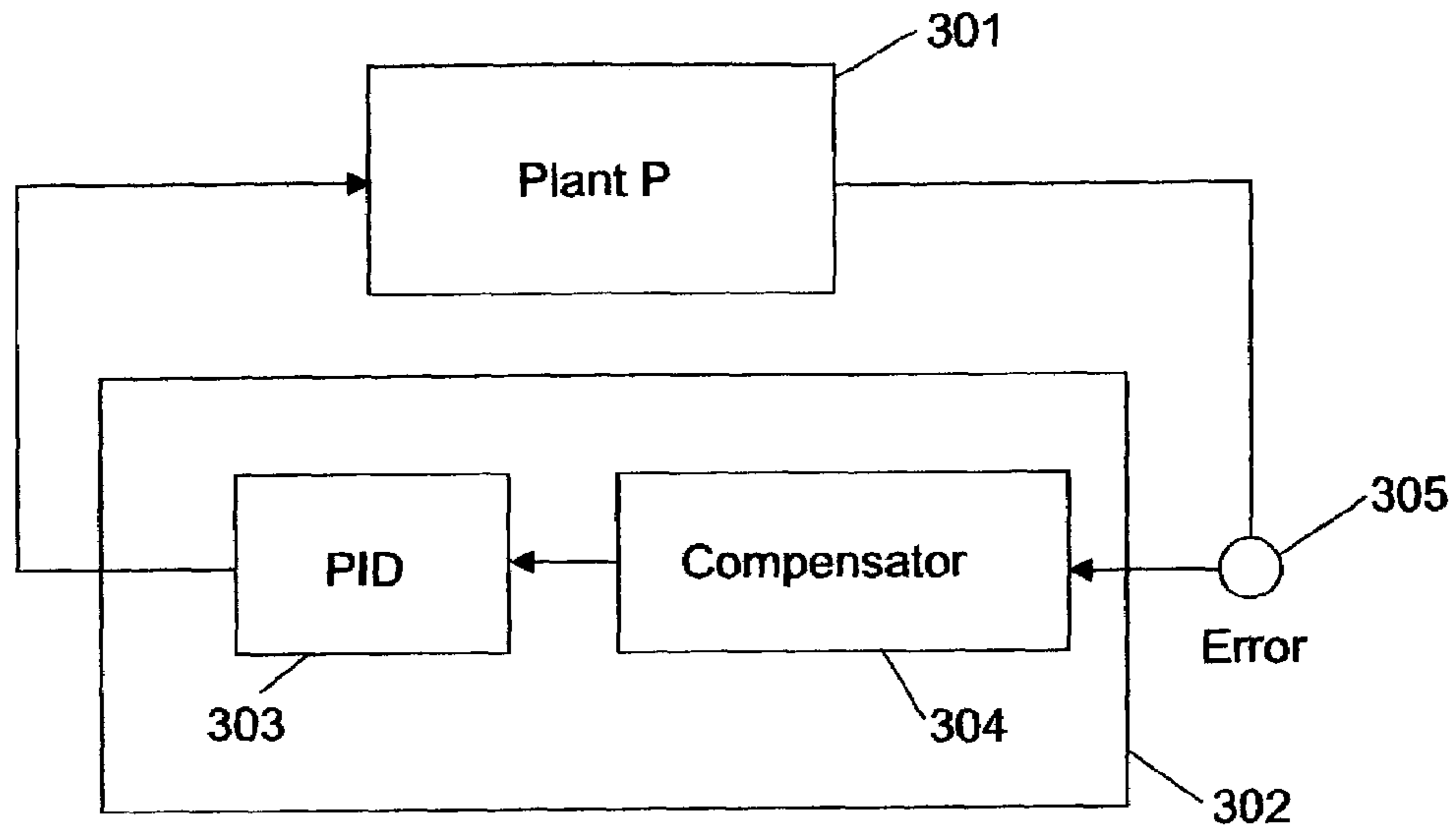
FIG. 3 Prior Art
