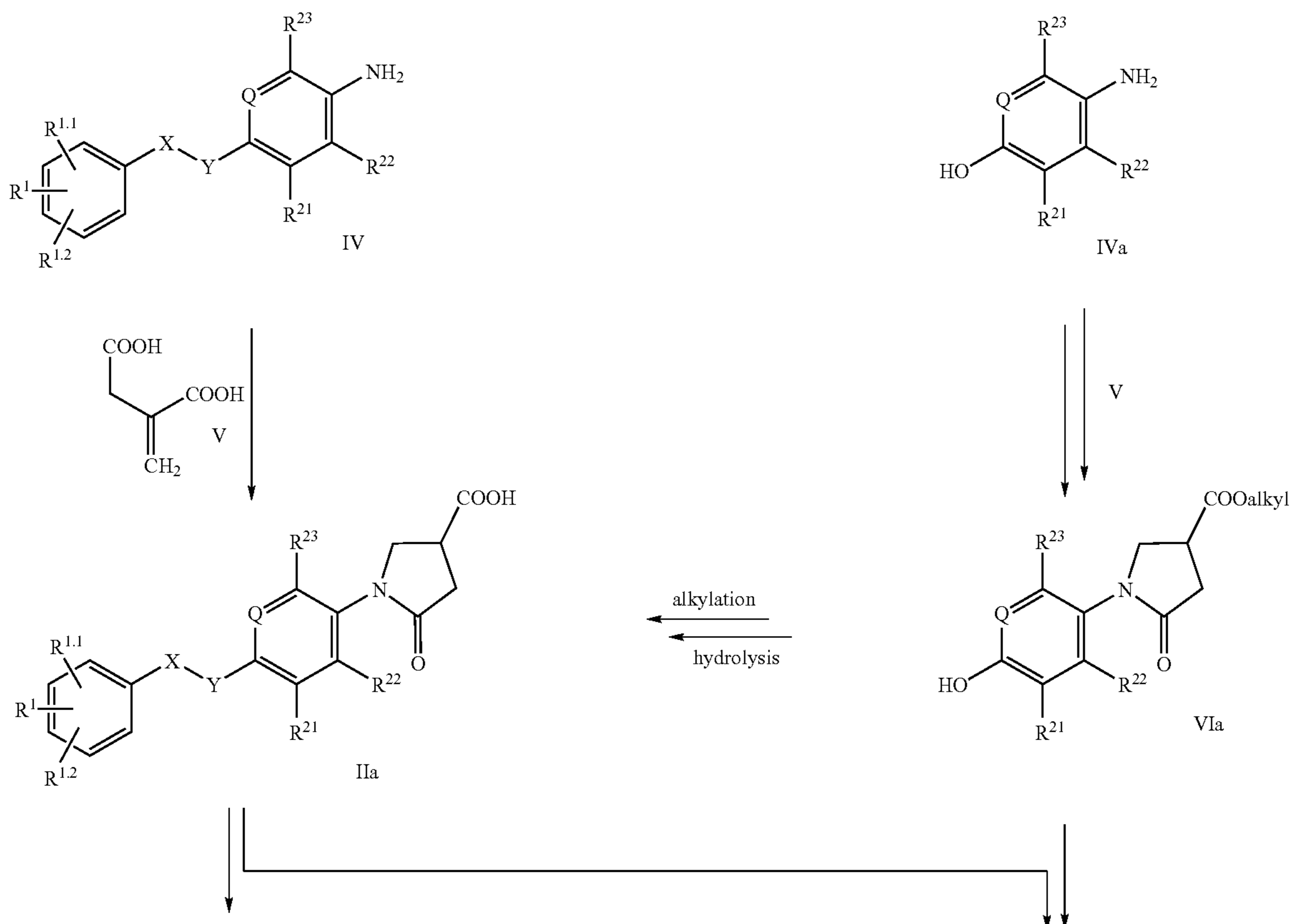
Scheme 1
