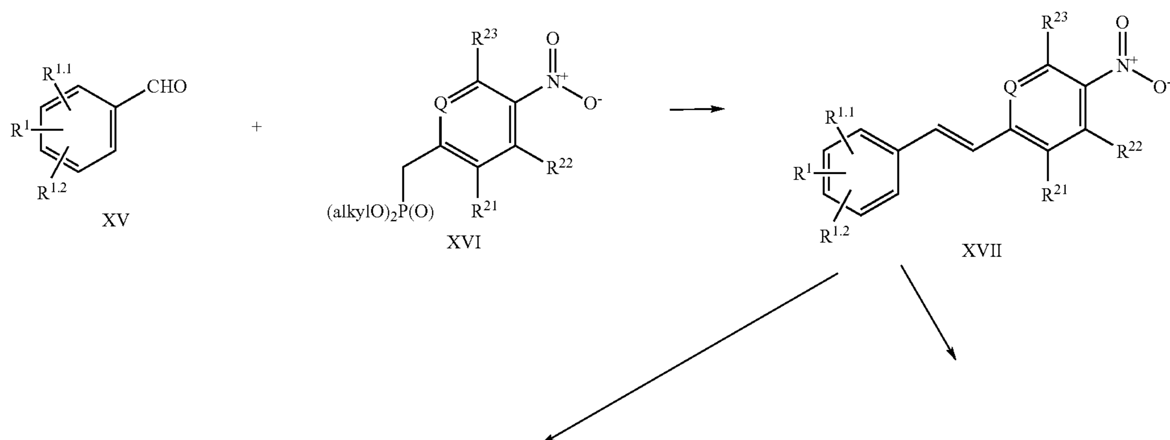
Scheme 4
