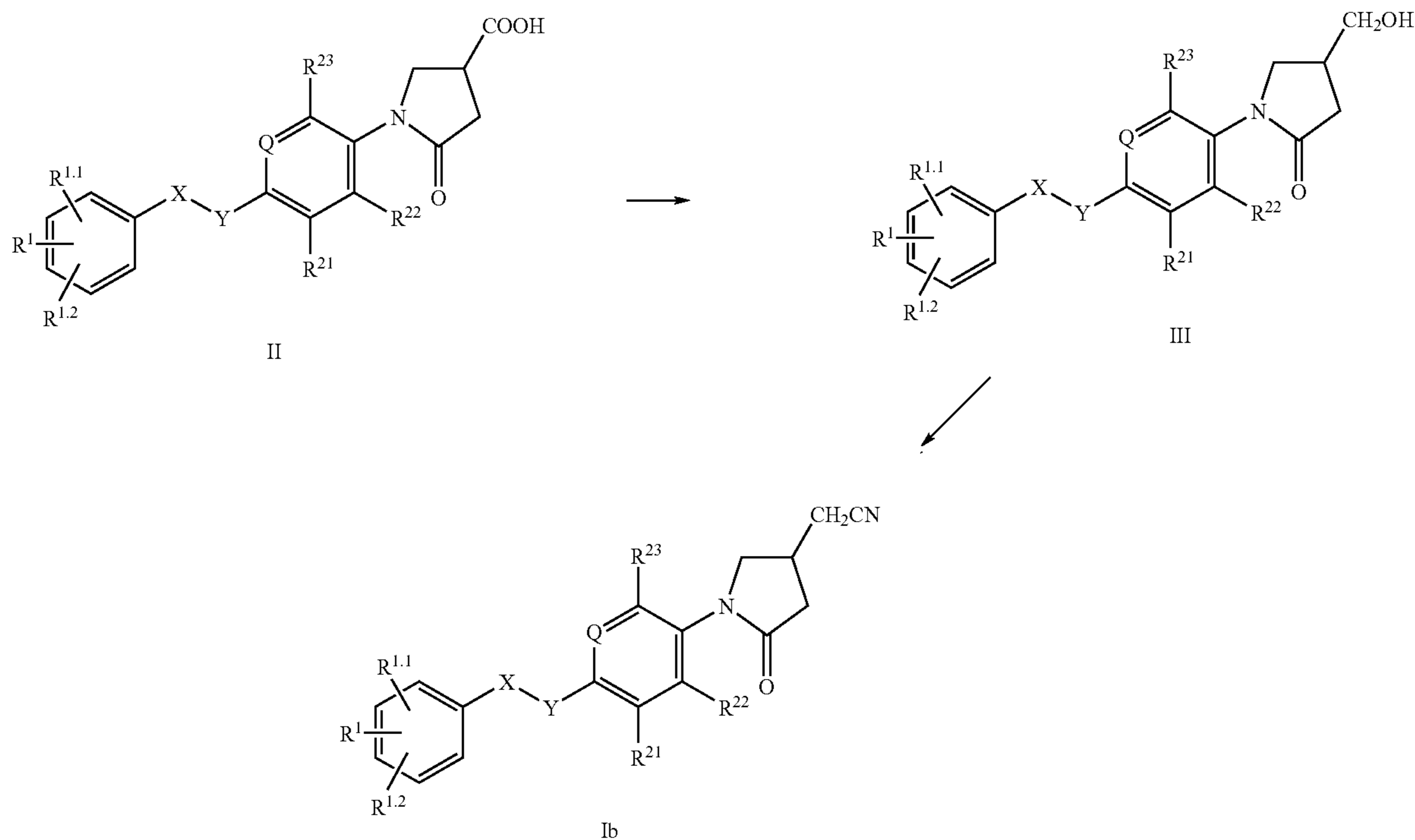
Scheme 5
