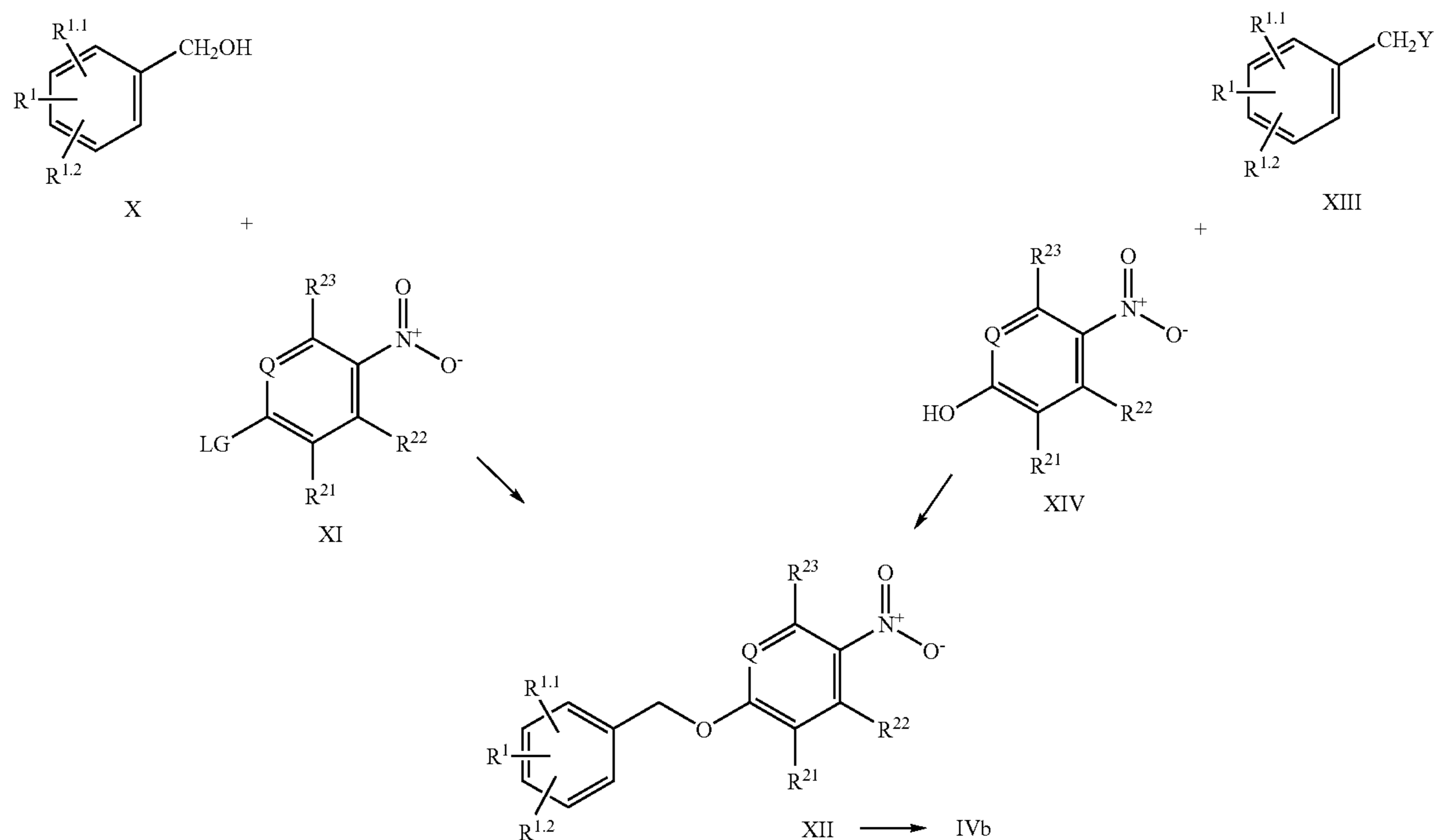
Scheme 3
