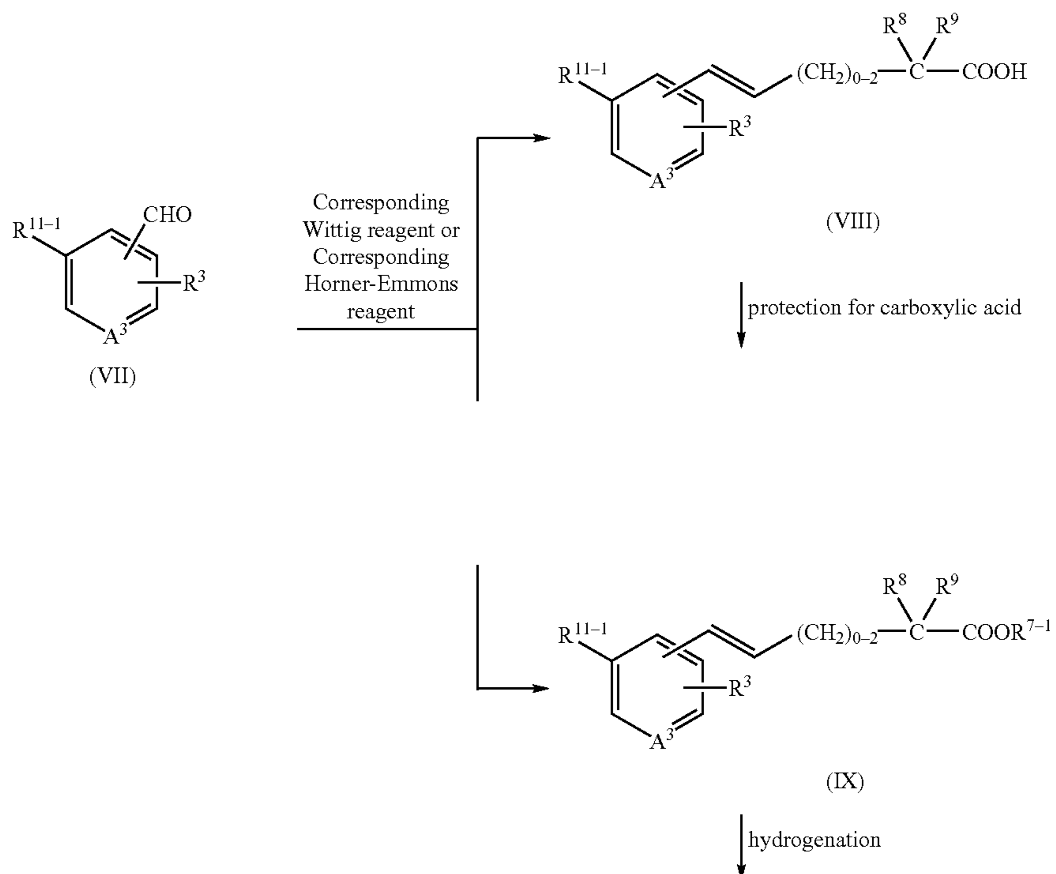
Scheme 1
