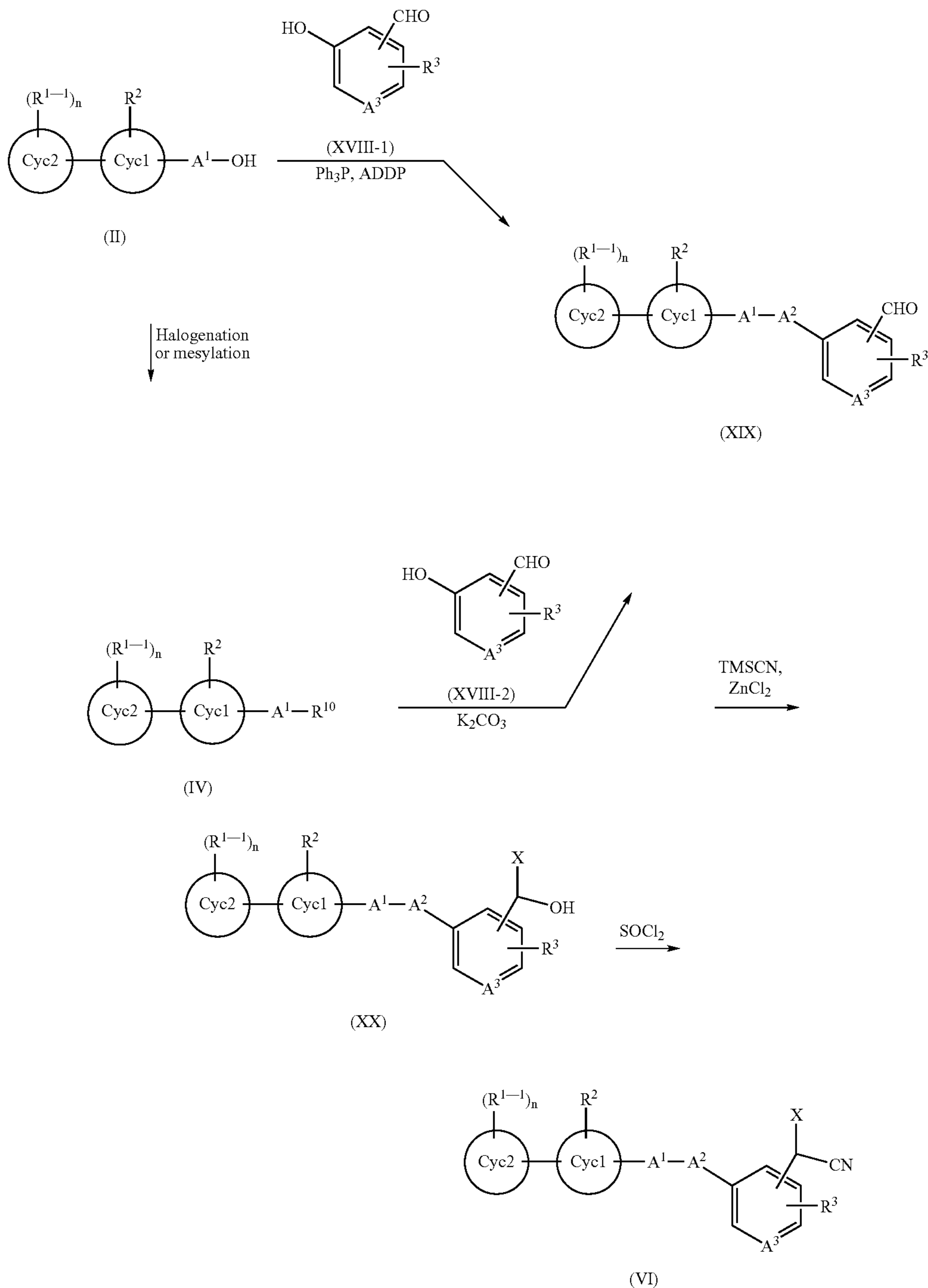
Scheme 4
