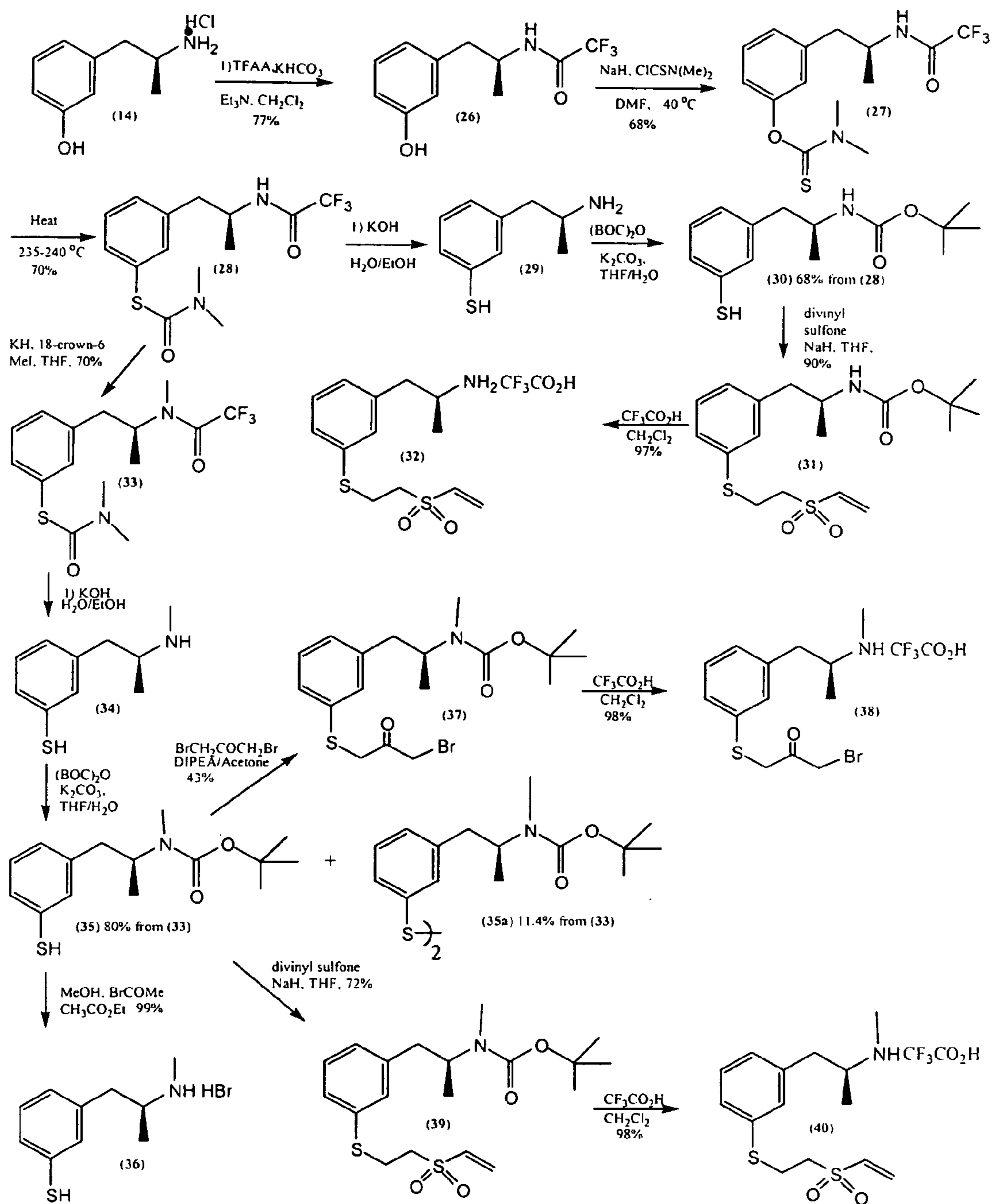
Fig. 2. Syntheses of Stereospecific Amphetamine Haptens (32),(36), (38) and (40)
