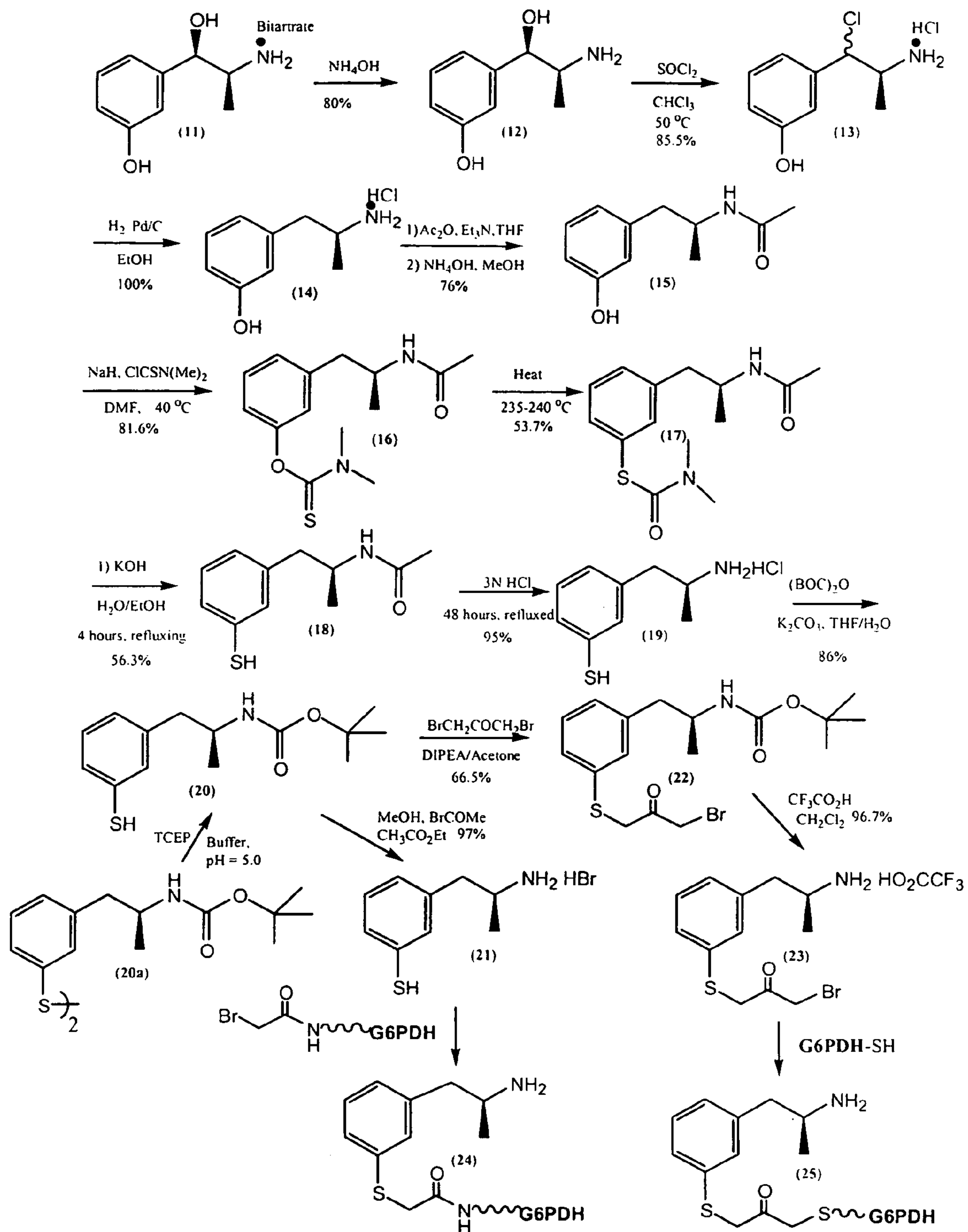
Fig. 1. Syntheses of Stereospecific Amphetamine Haptens (21) and (23)
