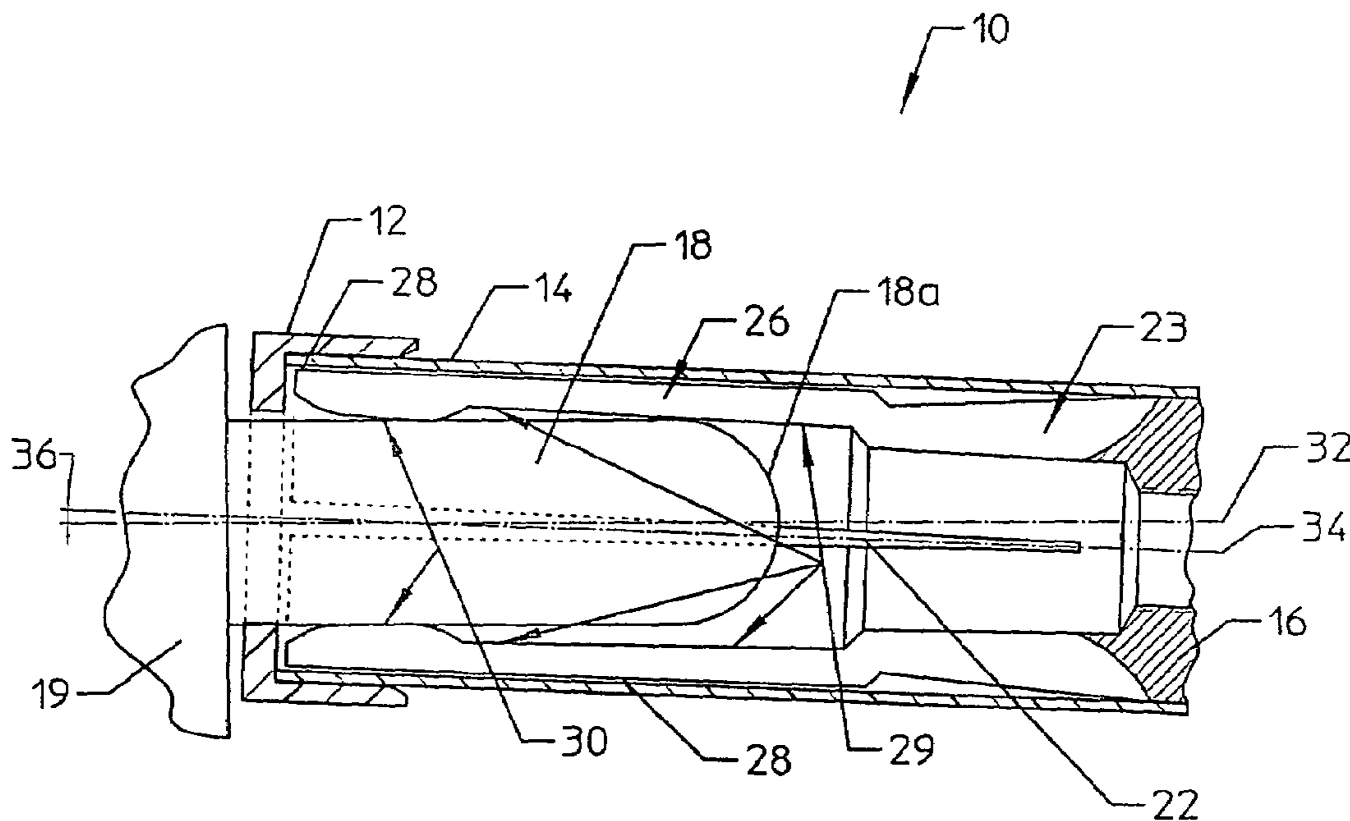
DETAIL A (MATED)
