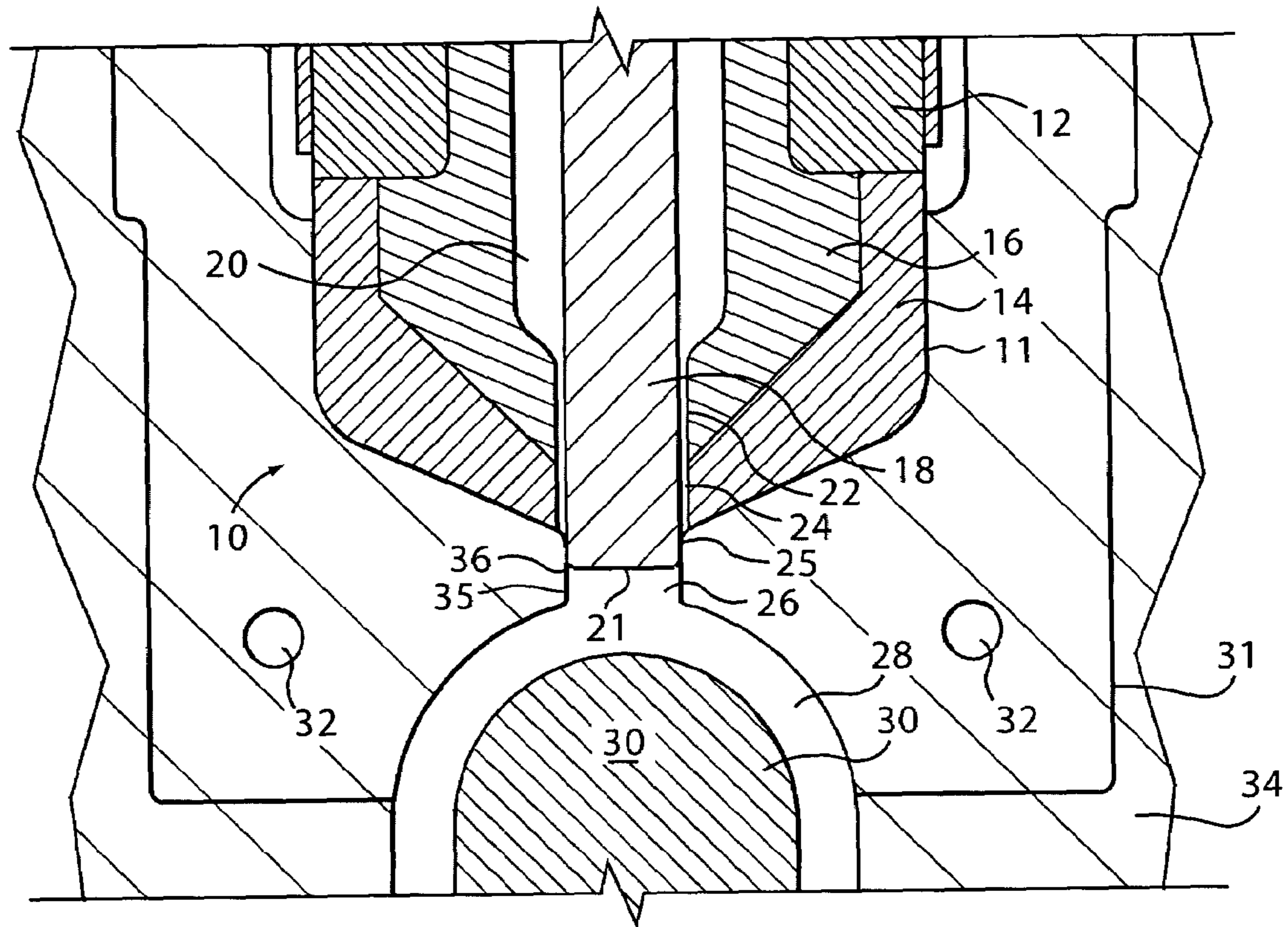
FIG. 1 (PRIOR ART)
