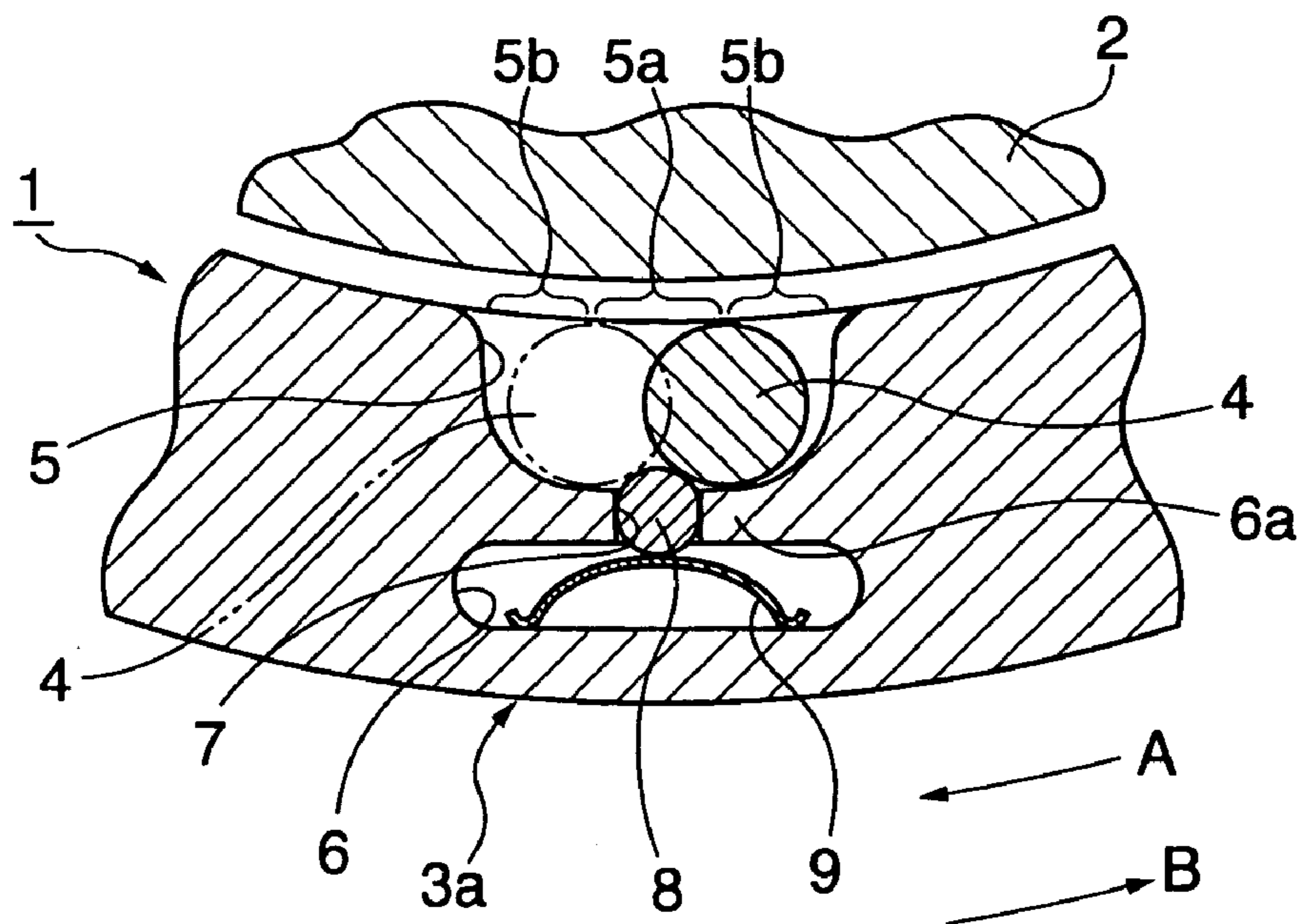
FIG. 2 PRIOR ART
