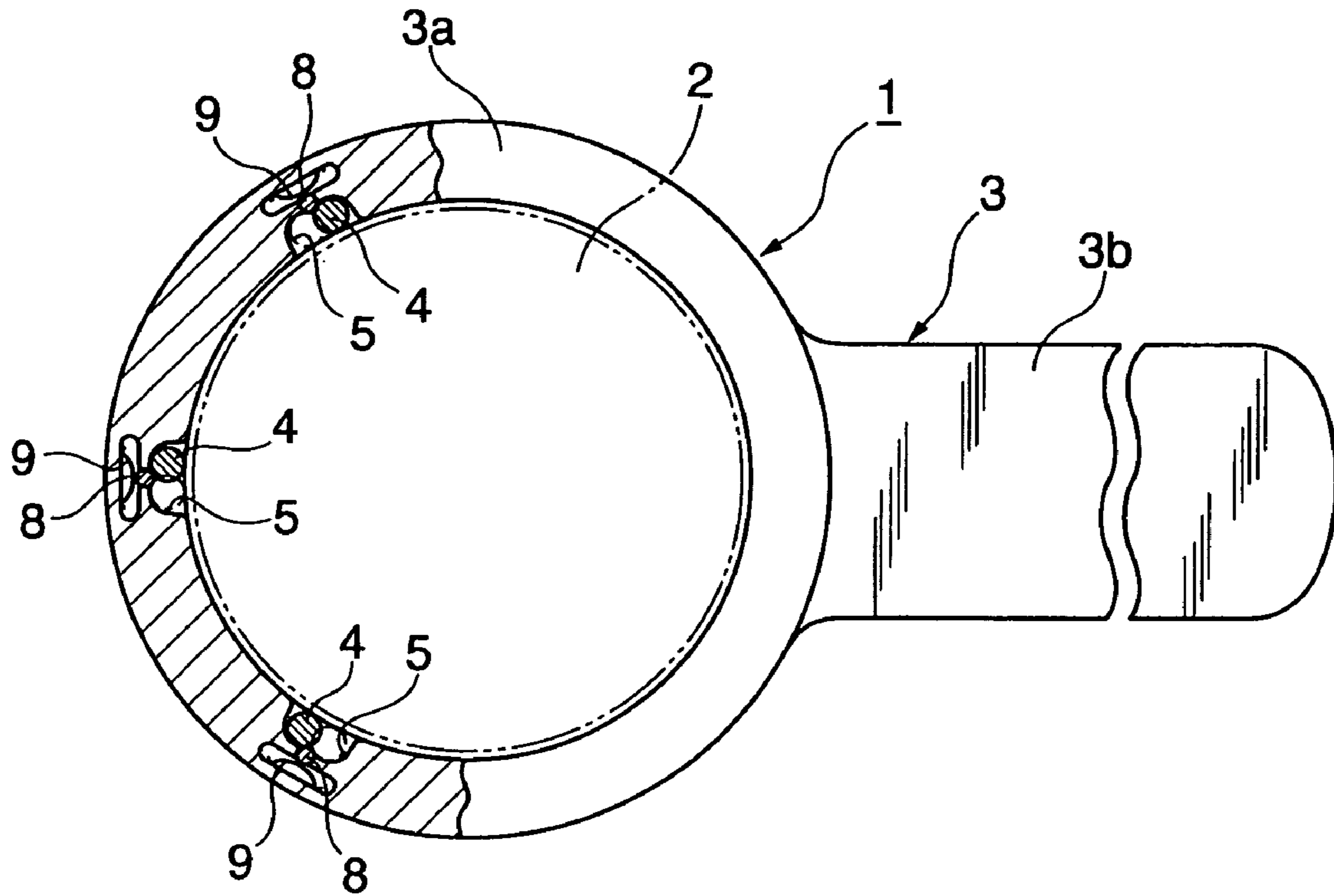
FIG. 1 PRIOR ART
