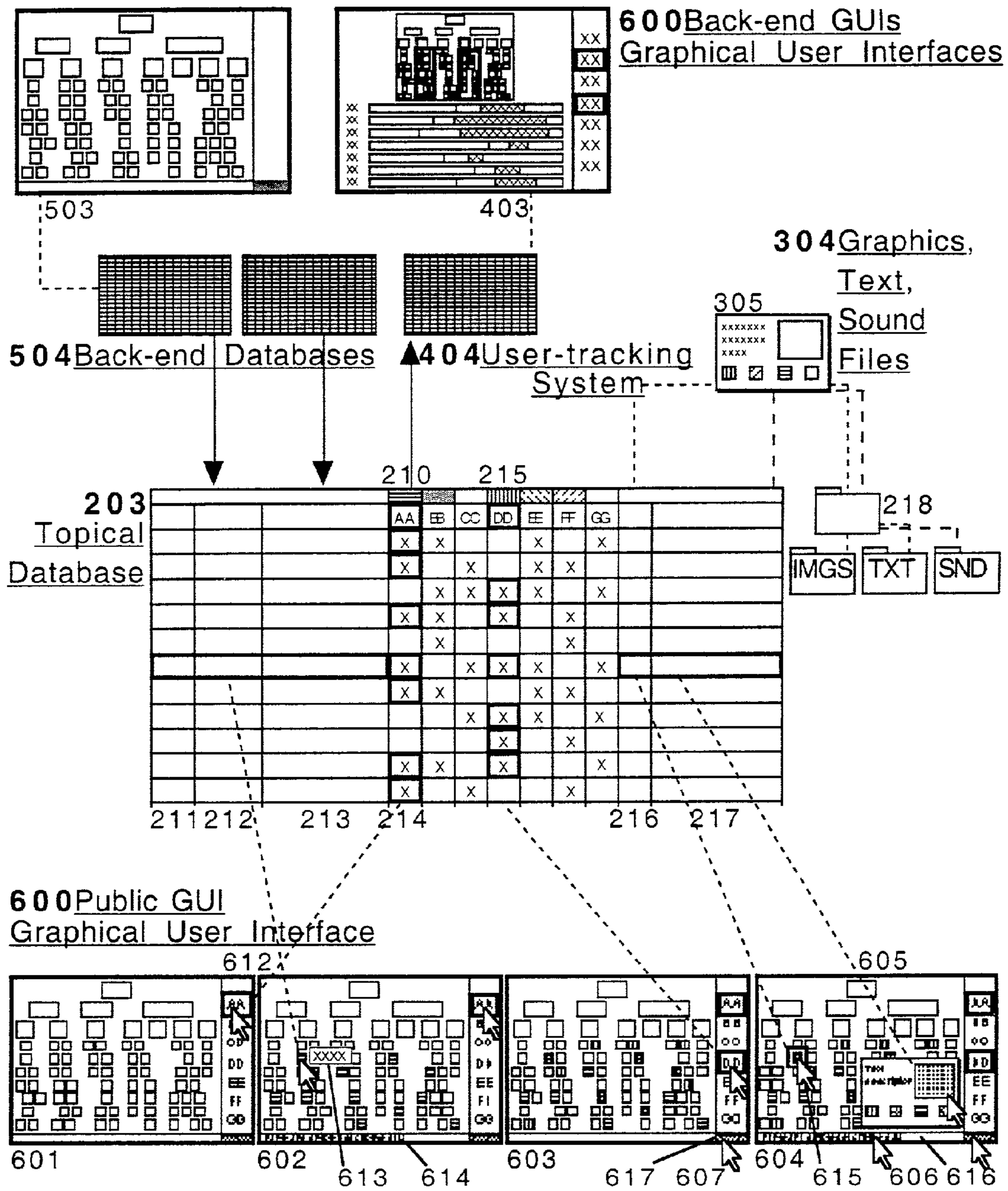
FIG. 4 GUI/Database Operations
