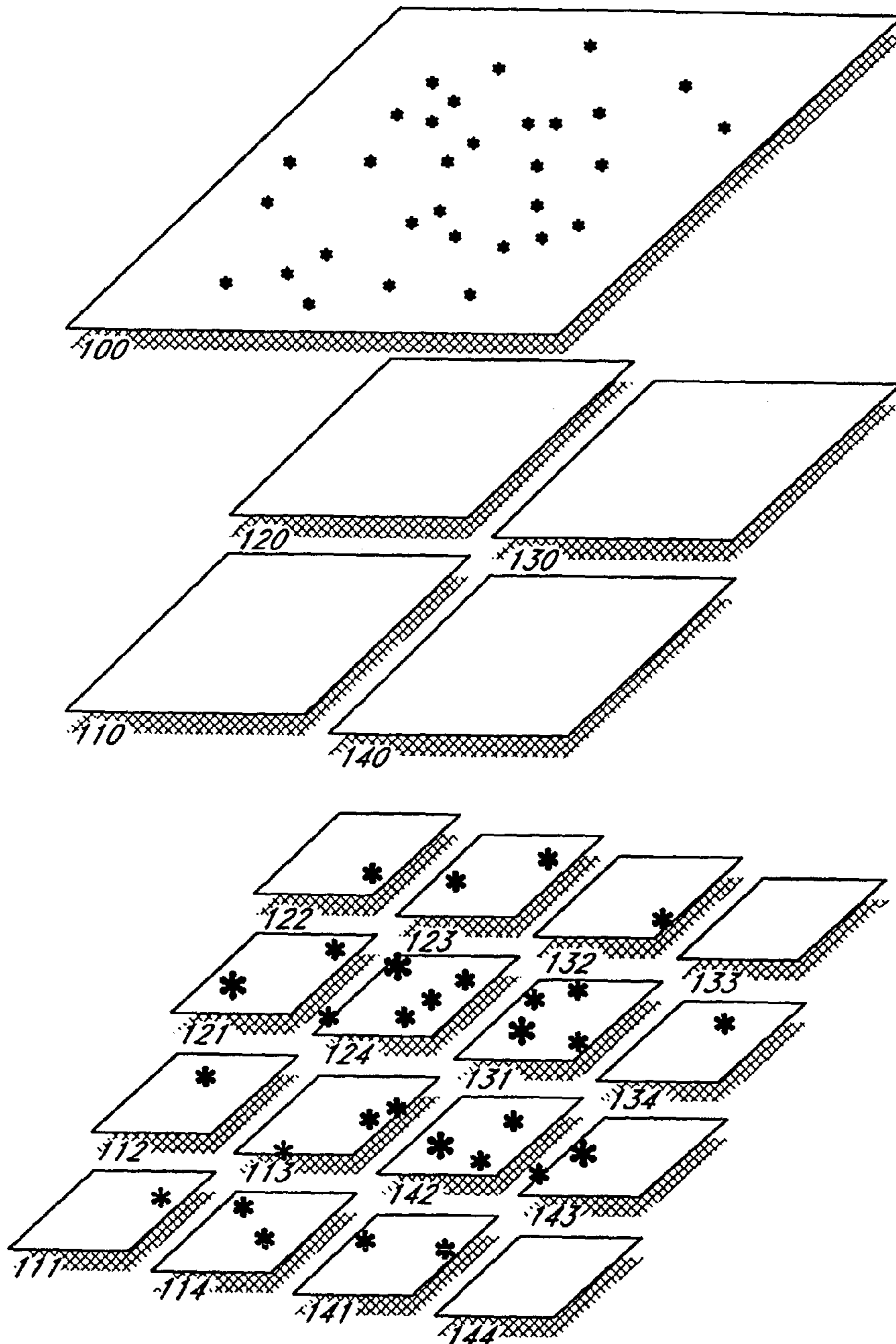
FIG. 9 (PRIOR ART)
