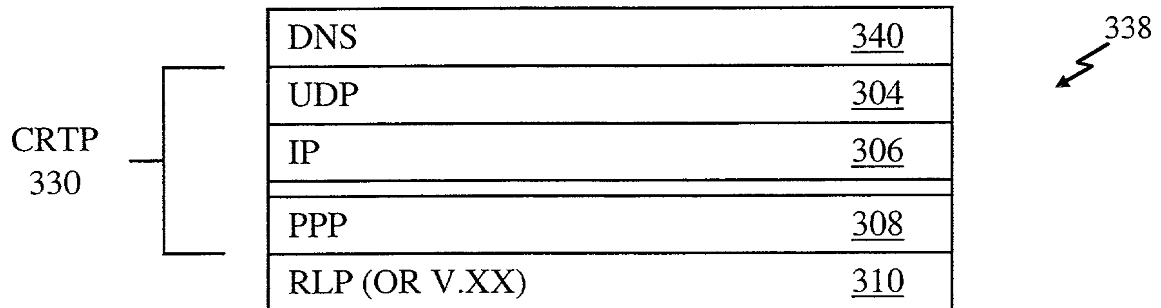
DNS CLIENT PROTOCOL STACK
