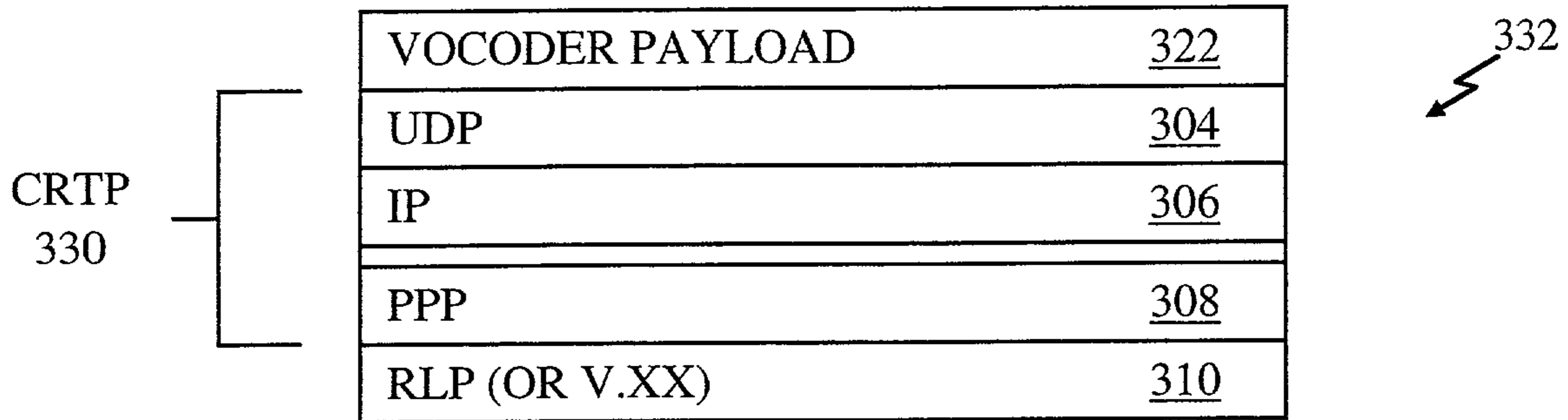
UDP VOICE MEDIA PROTOCOL STACK
