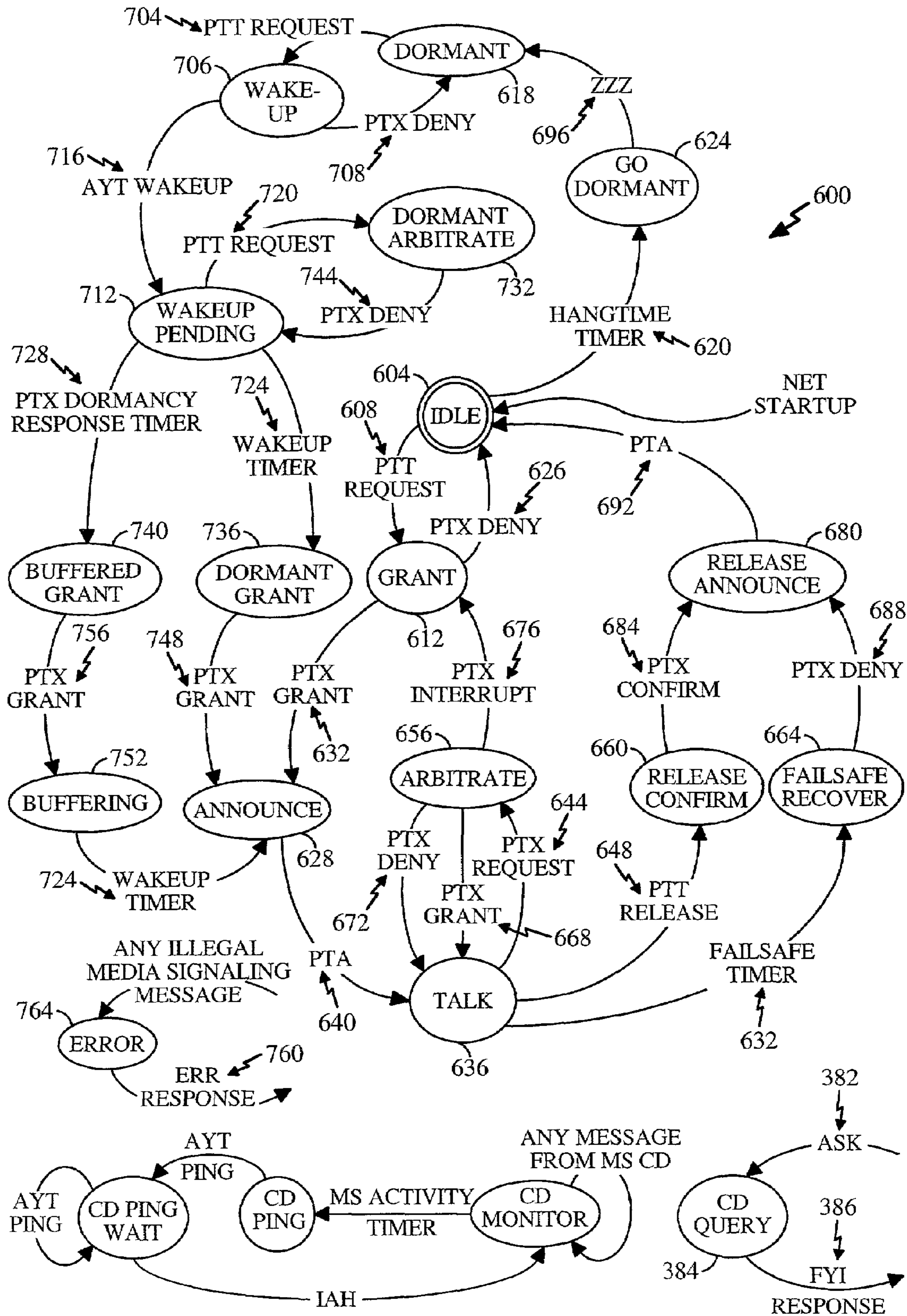
FIG. 15 MEDIA SIGNALING STATE DIAGRAM
