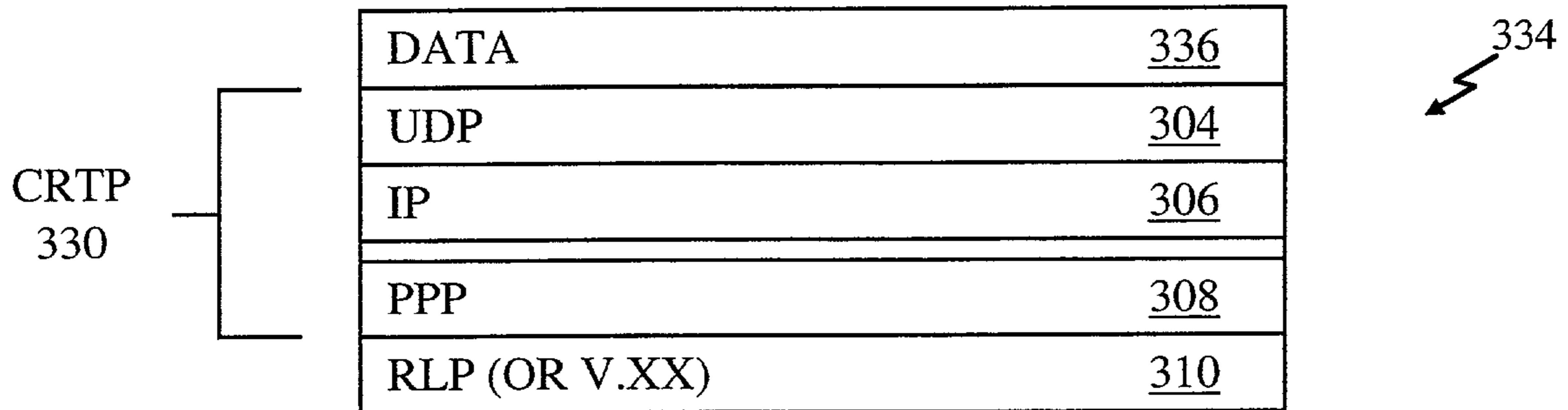
MEDIA TRAFFIC (DATA) PROTOCOL STACK
