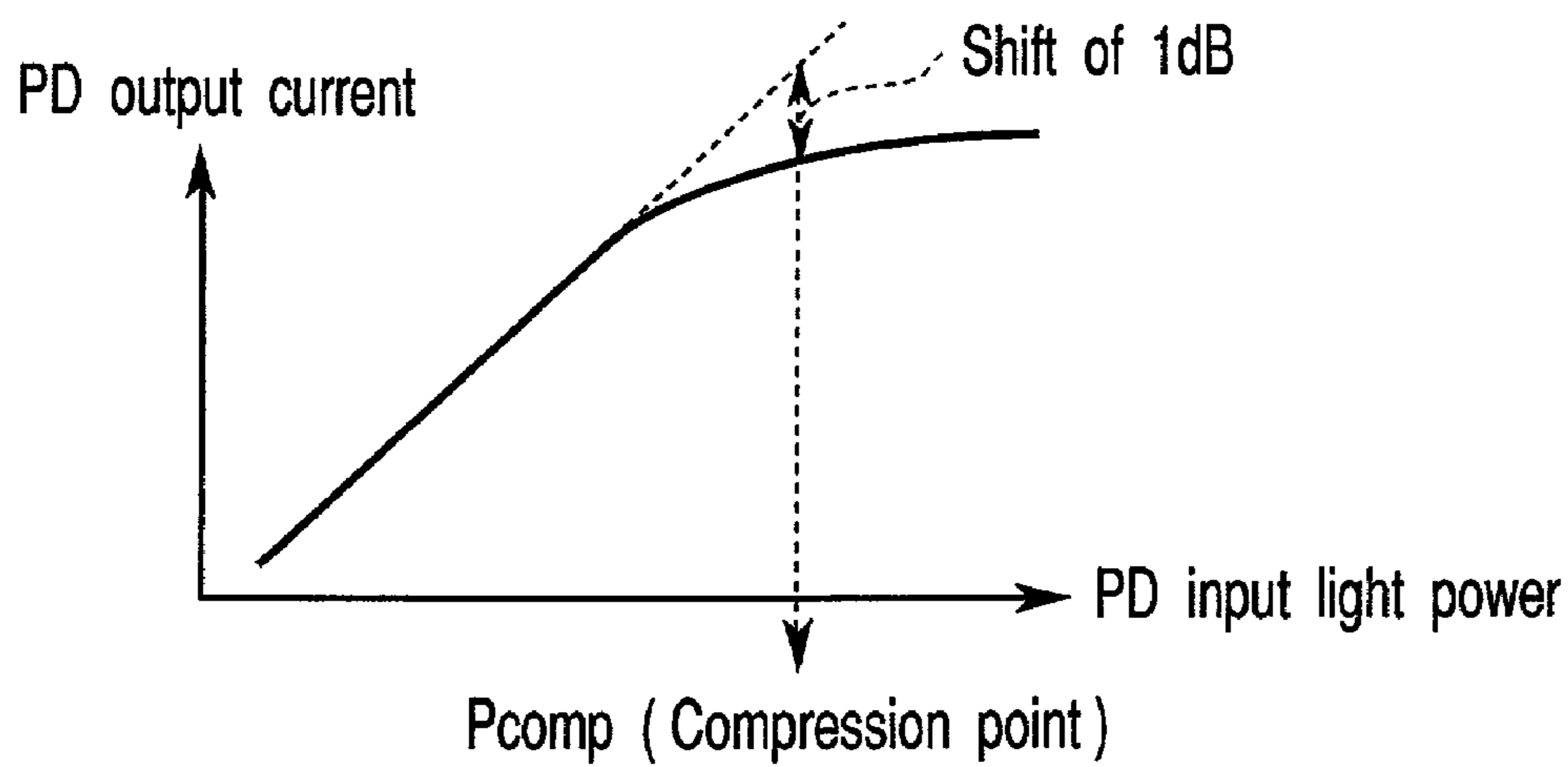
FIG. 7 (Prior art)
