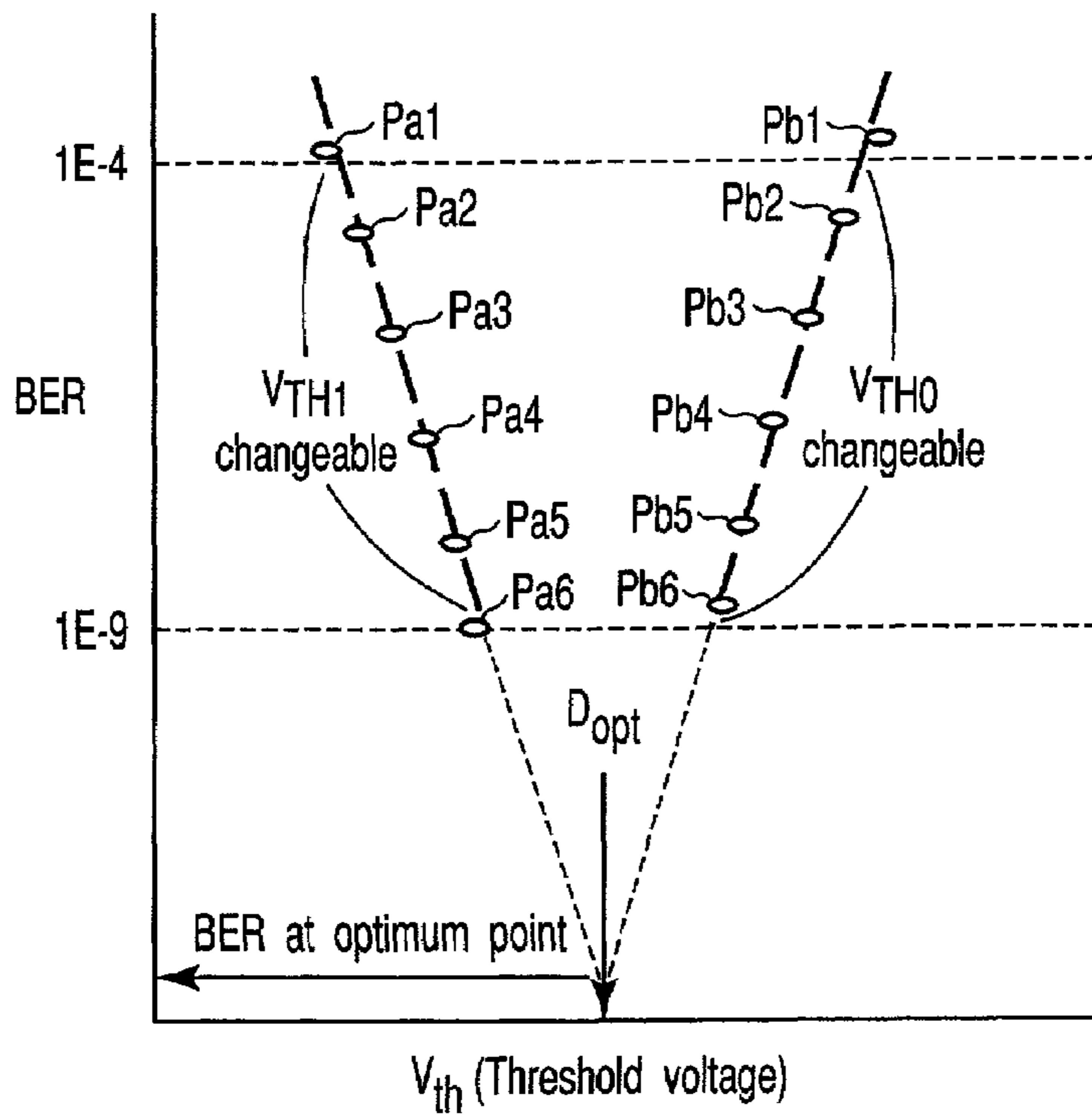
FIG. 9 (Prior art)
