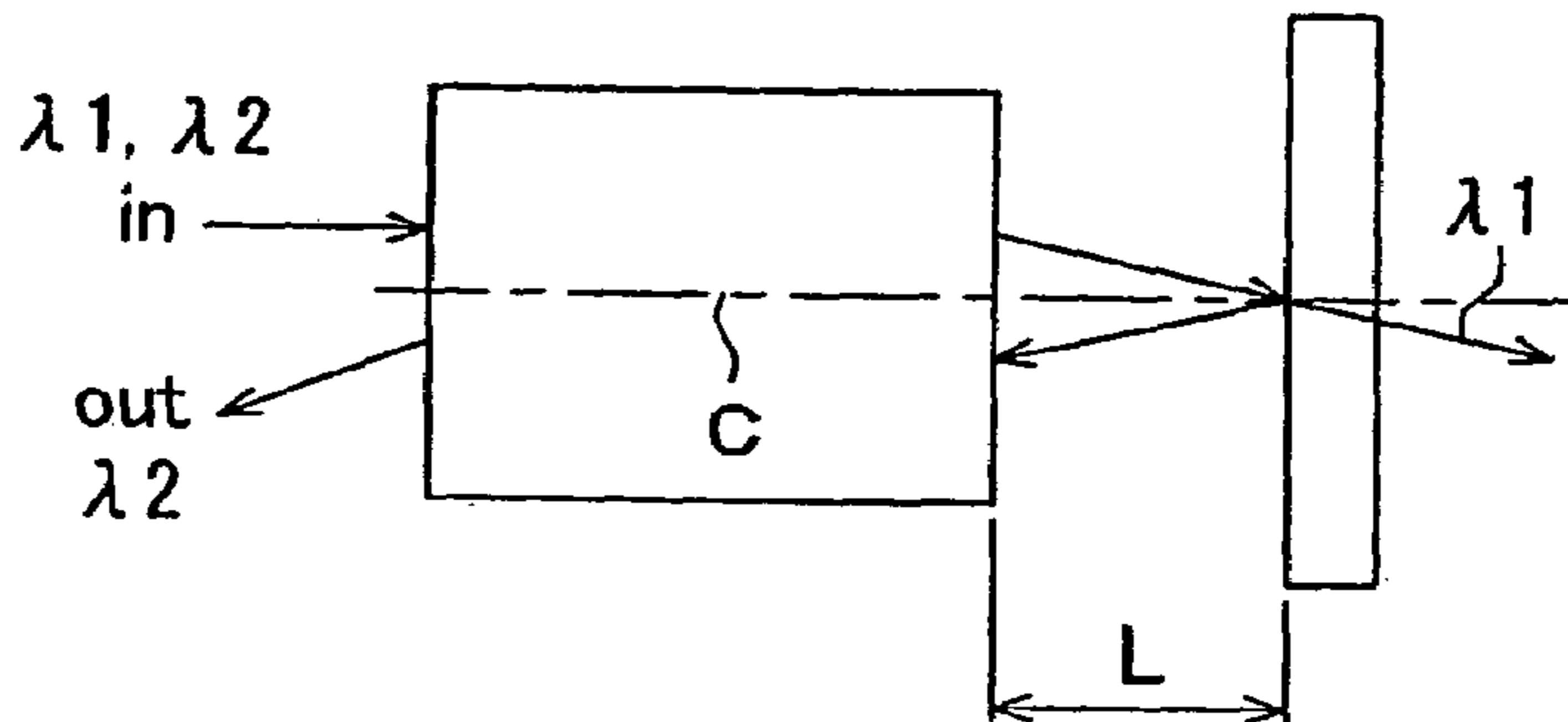
Mirror displaced from Focal Point of Lens
