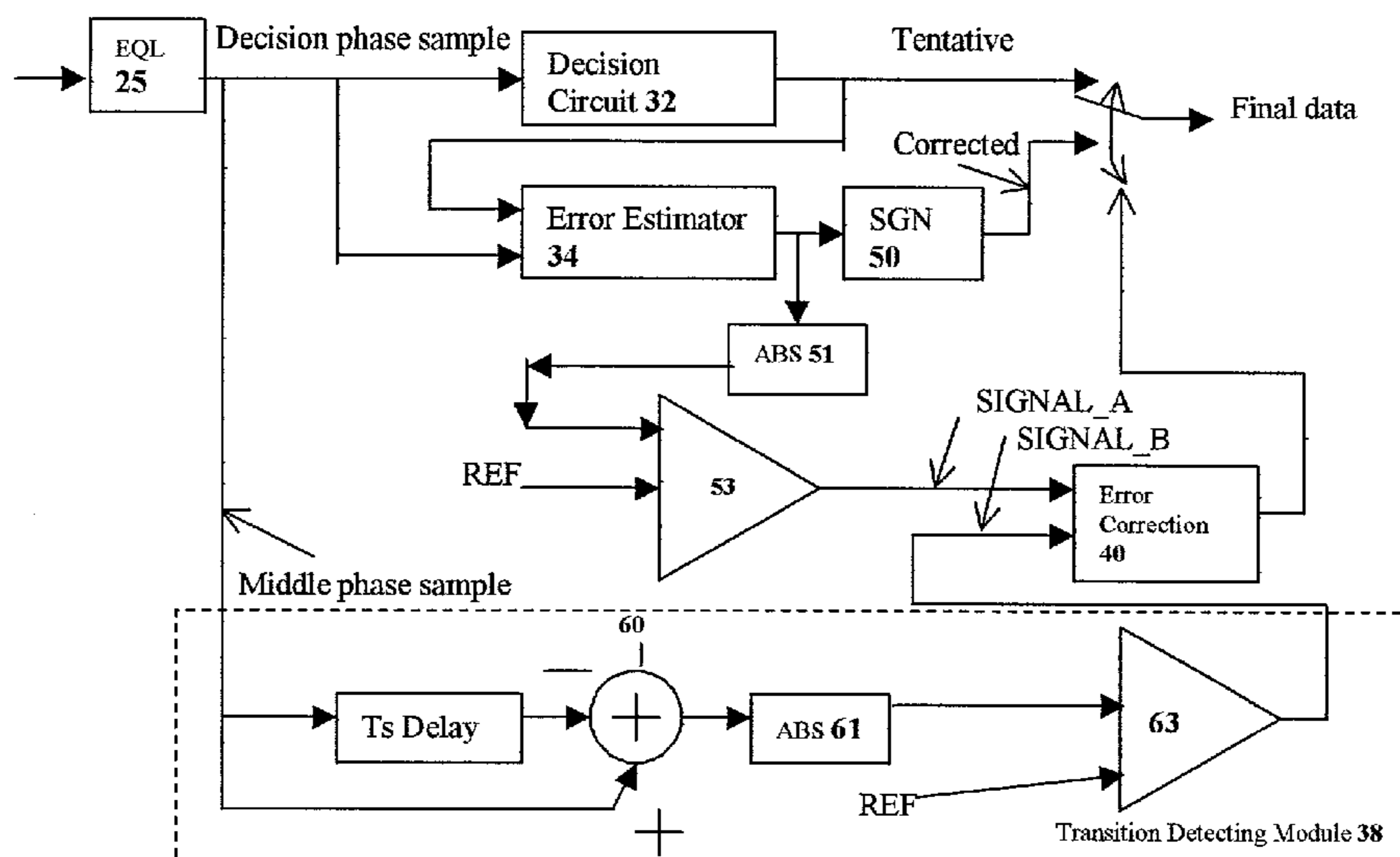
Block Diagram of Error Corrector
