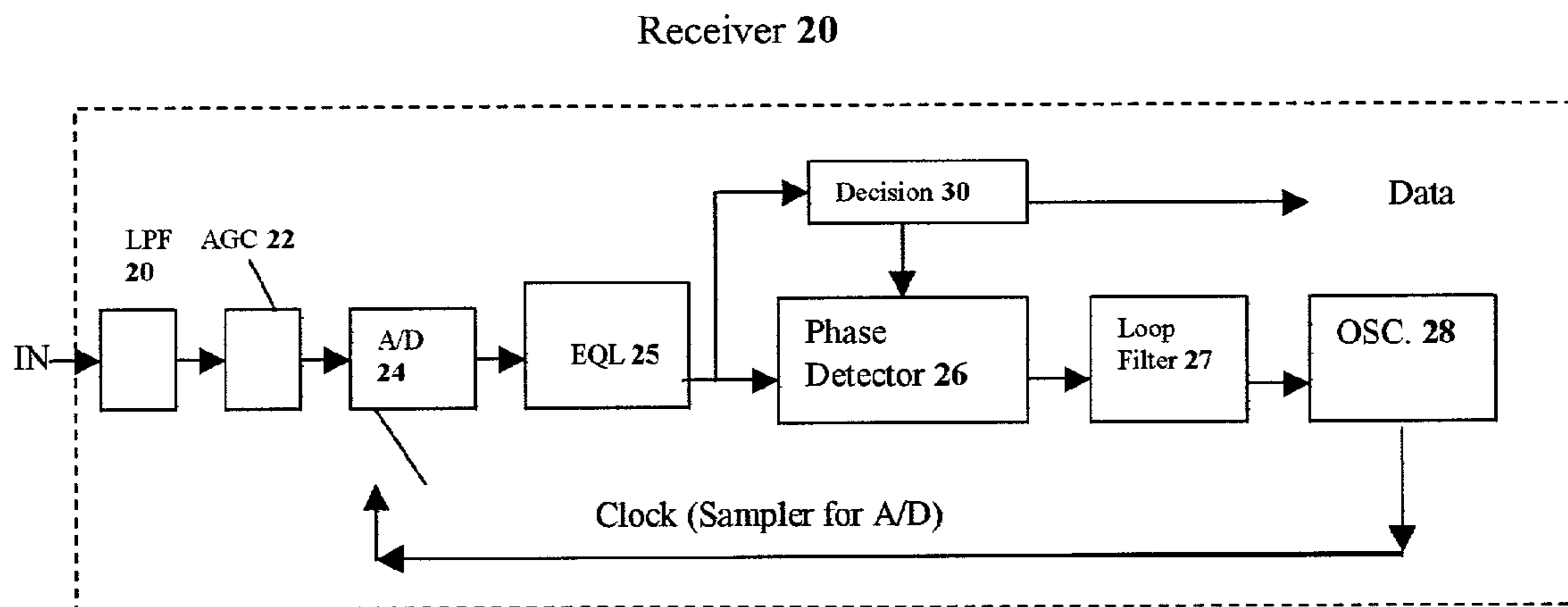
Figure 3. Block Diagram of the Entire Receiver
