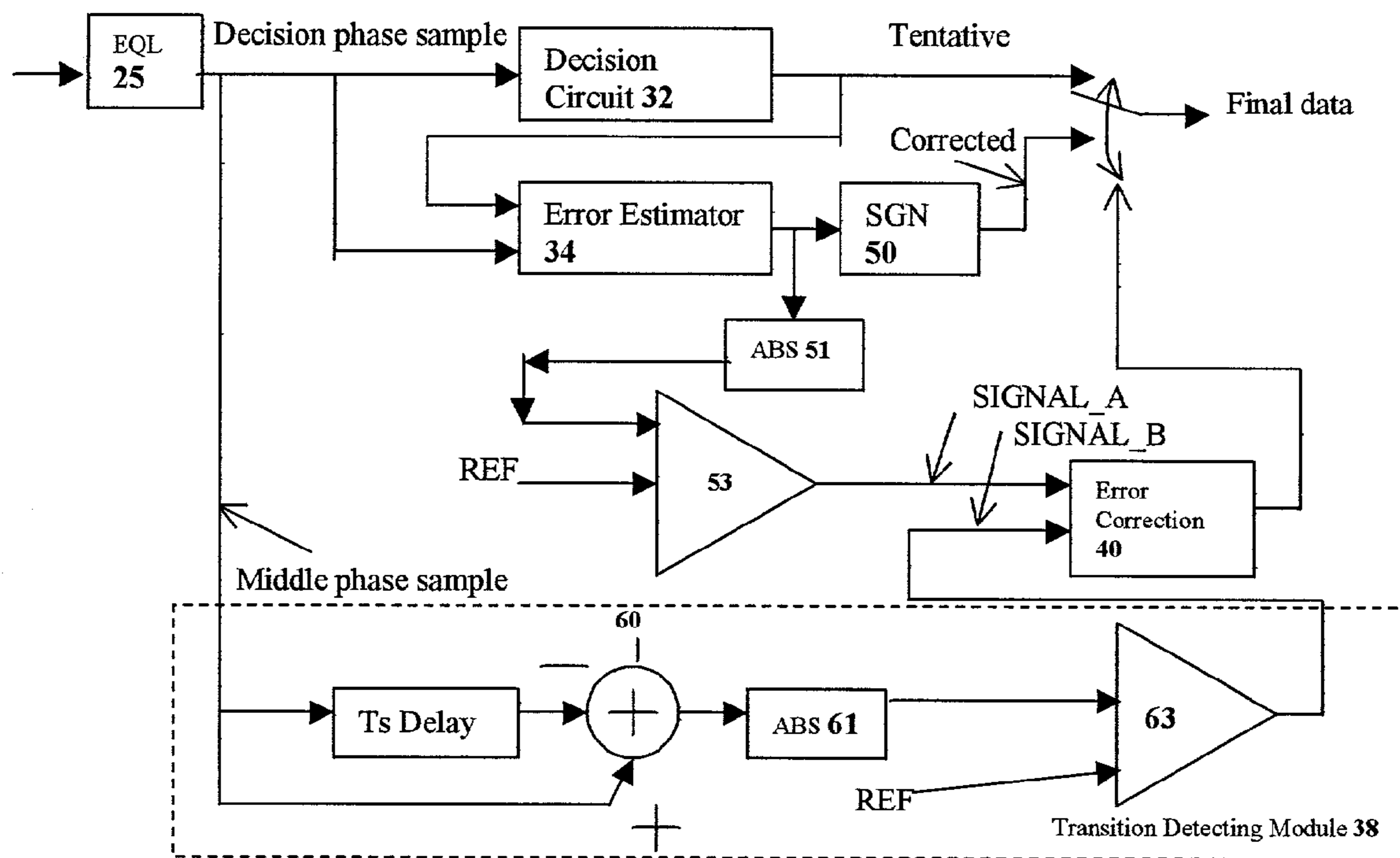
Figure 5. Block Diagram of Error Corrector
