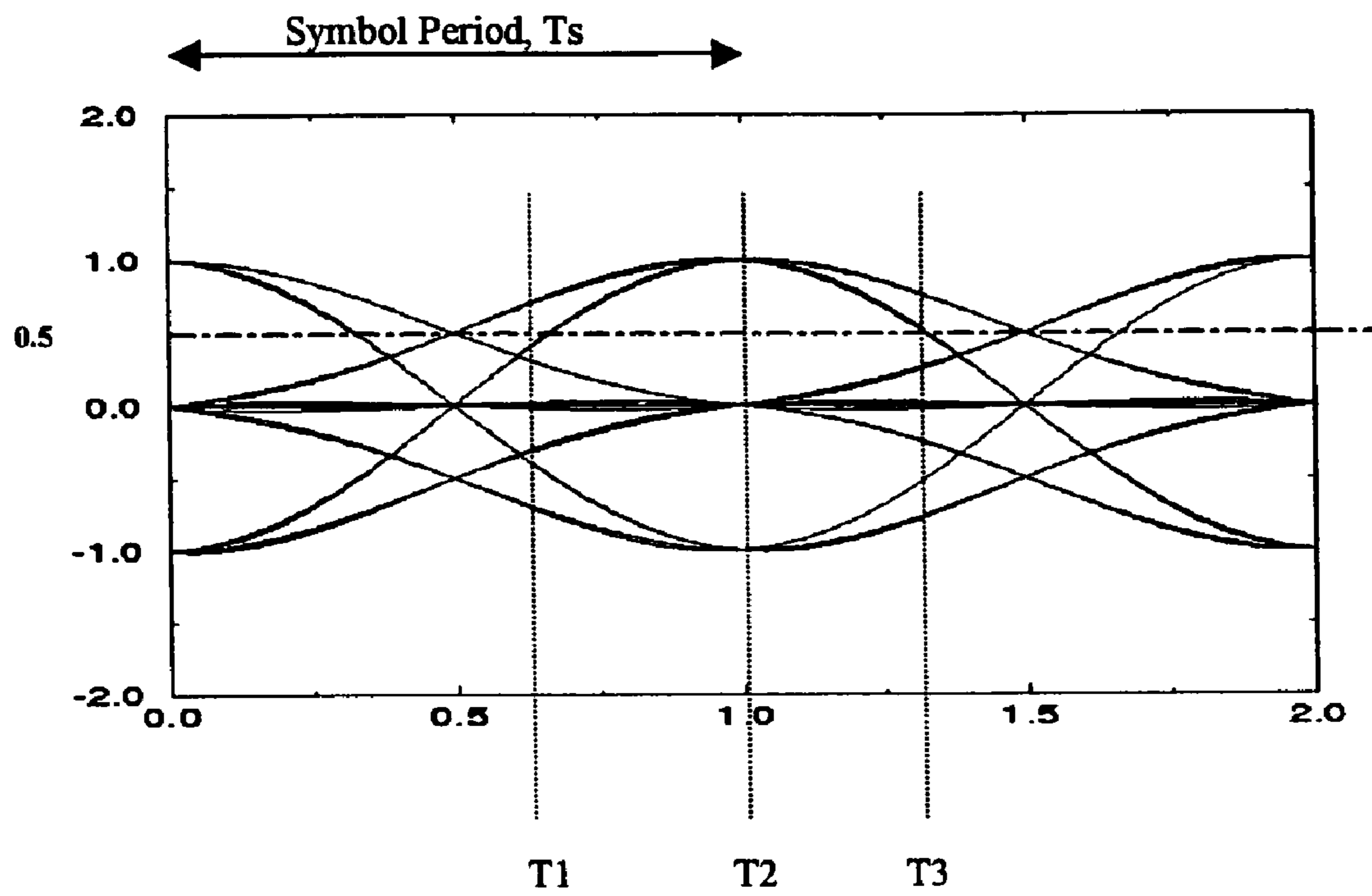
Figure 1. Eye Pattern
