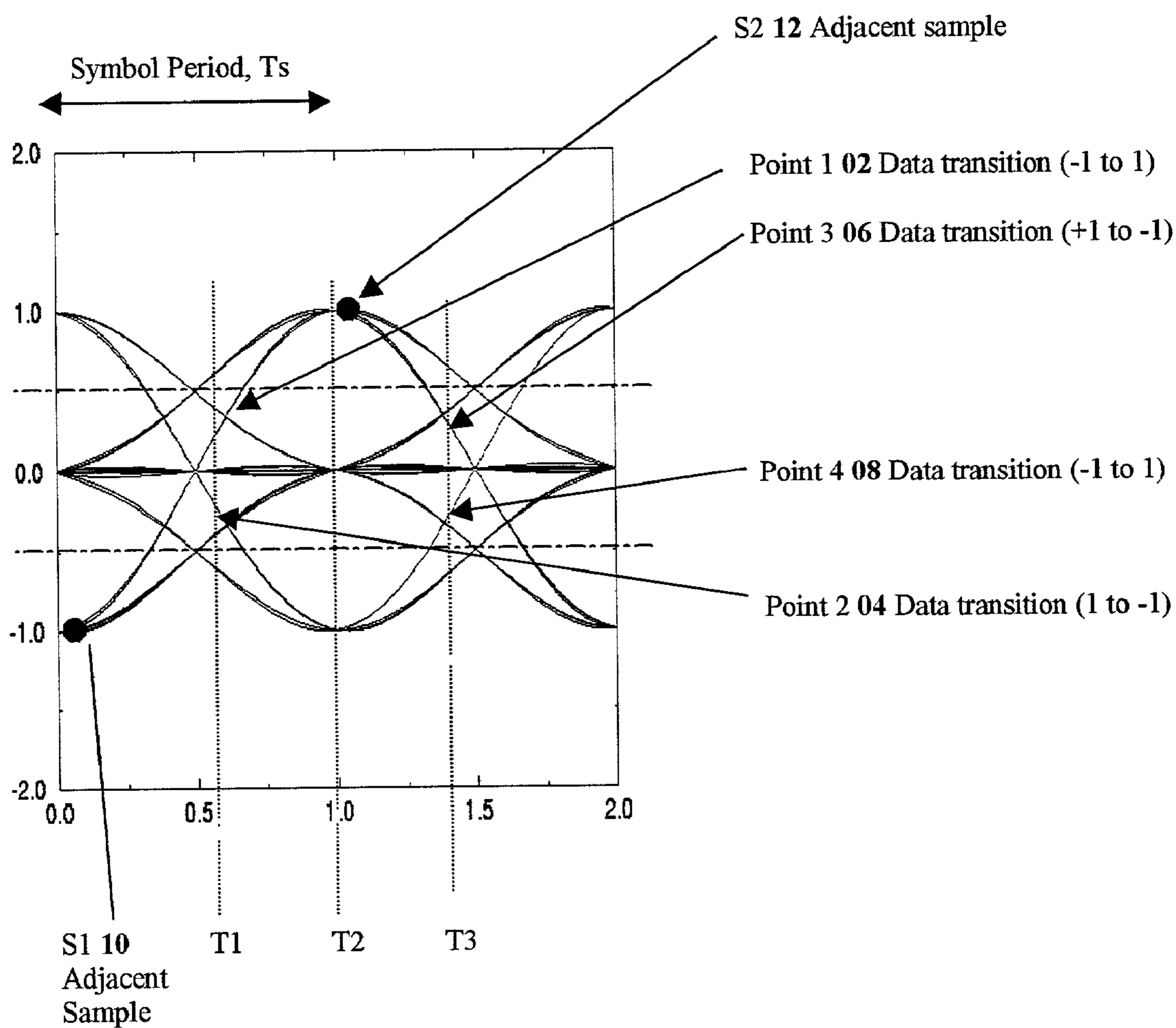
Figure 2. Error Events in Eye Diagram
