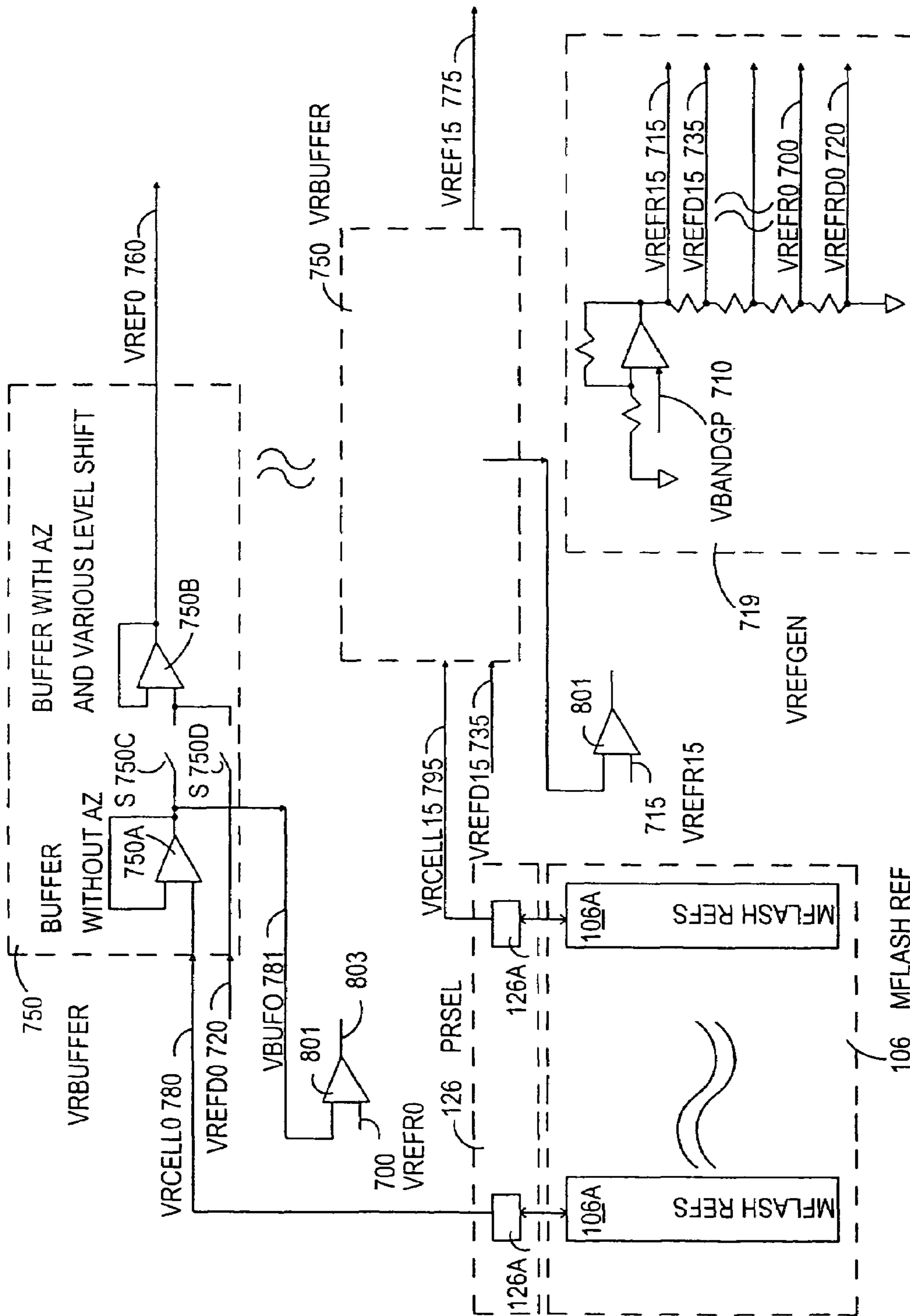
BLOCK DIAGRAM OF REFERENCE SYSTEM FOR SUPER HIGH DENSITY DIGITAL MULTILEVEL NON-VOLATILE MEMORY
