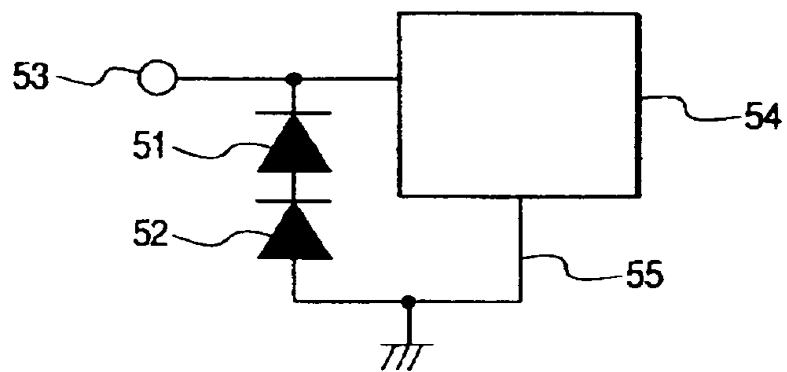
FIG. 11 PRIOR ART
