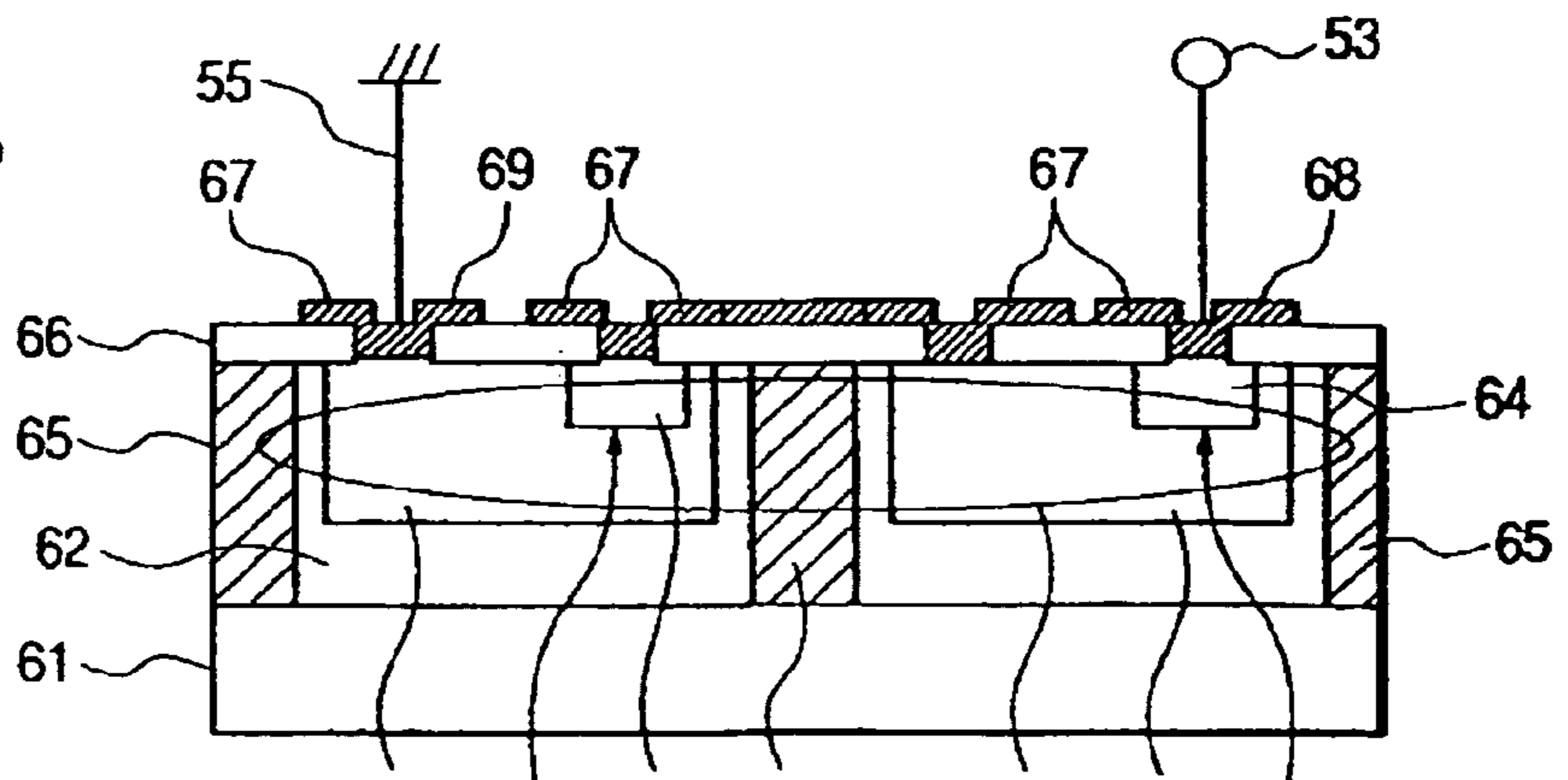
FIG. 12 PRIOR ART
