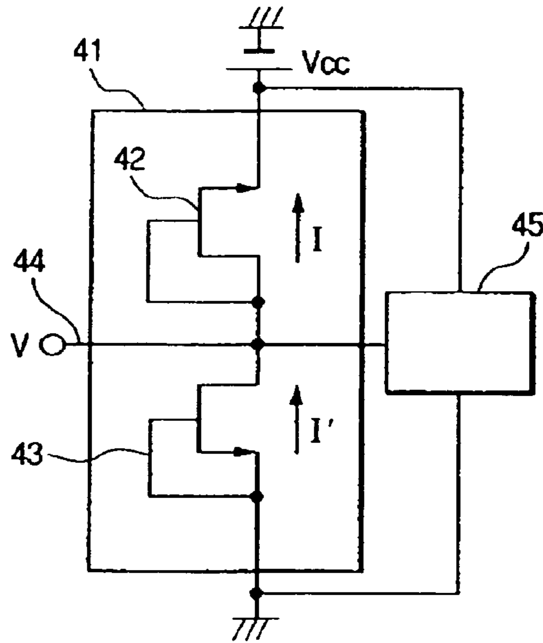
FIG. 10 PRIOR ART
