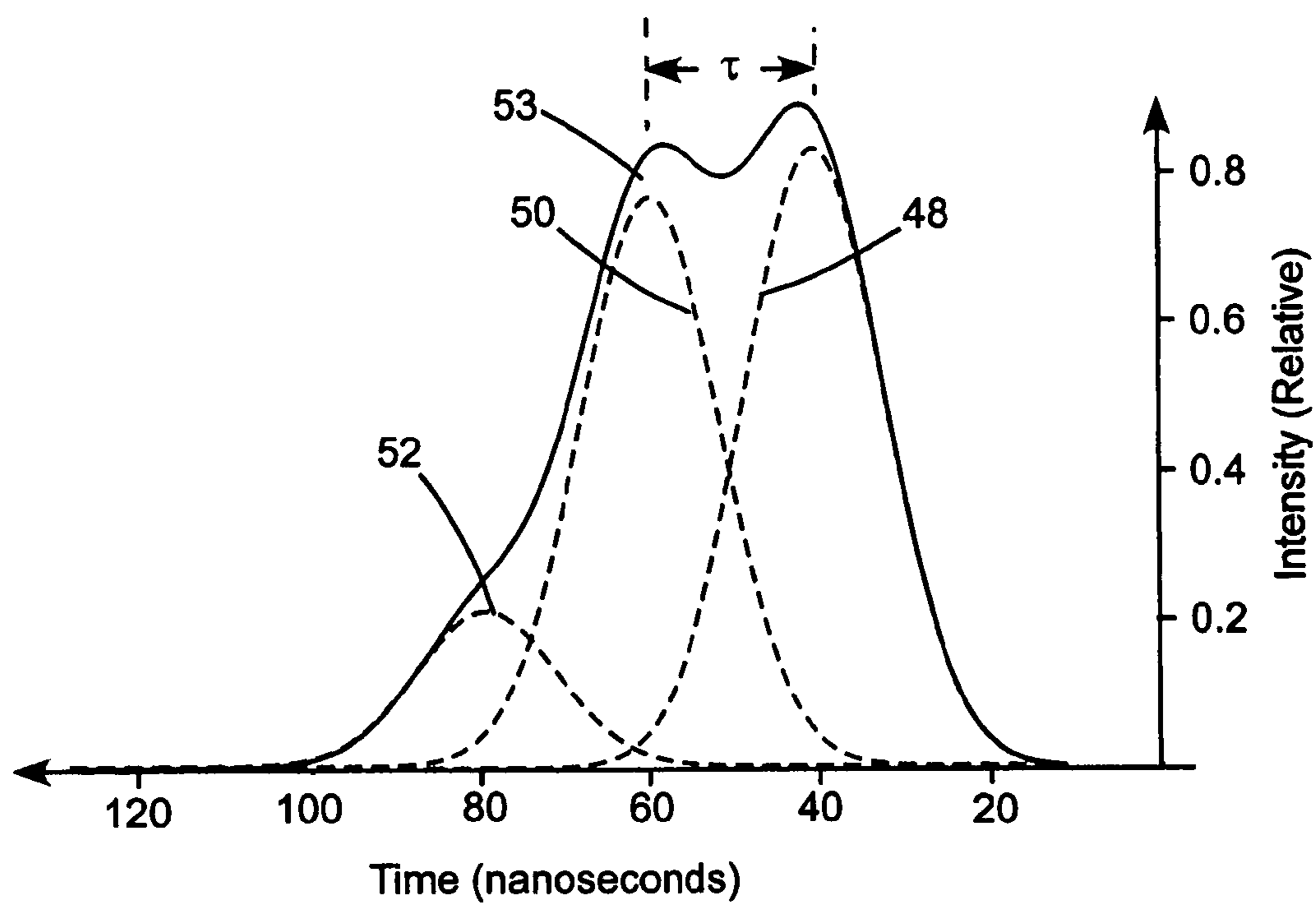
FIG. 3 (Prior Art)
